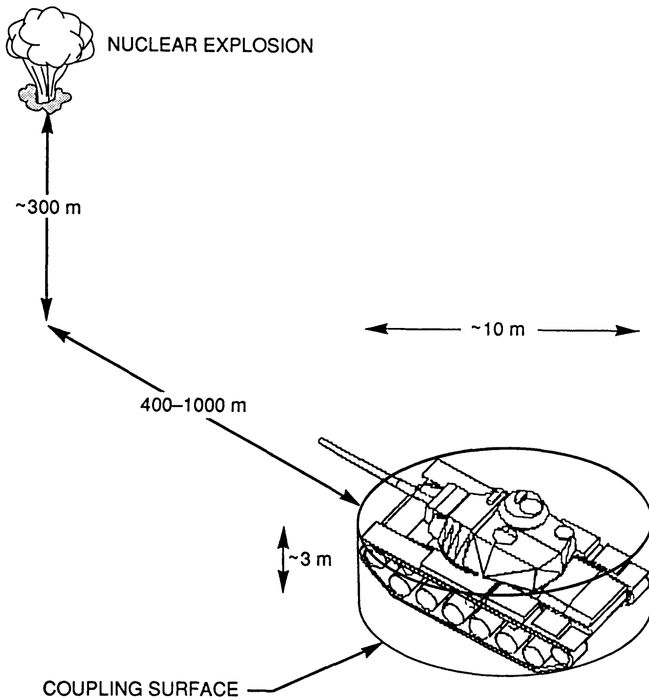
Figure 1-1. Typical VCS Problem Involving an Armored Vehicle.
