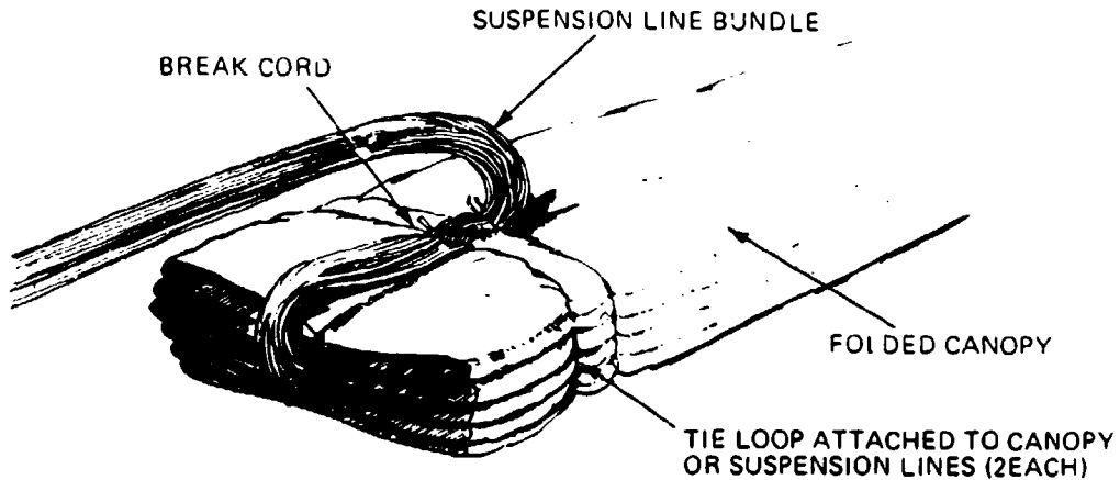
FIGURE 6-39. Skirt Hesitator.
