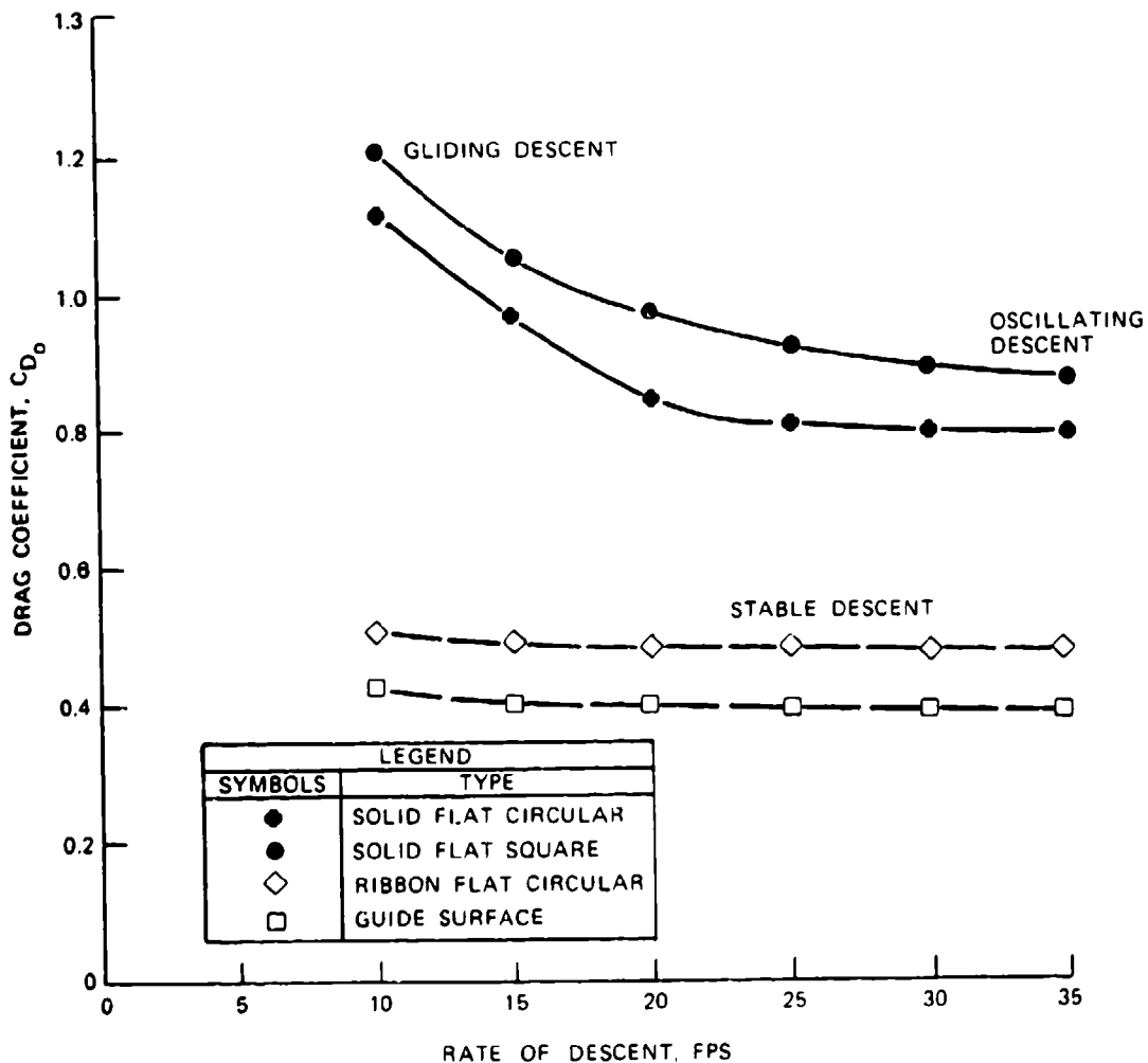
FIGURE 5-18. Drag Coefficient Versus Rate of Descent for Two Stable and Two Unstable Parachutes.
