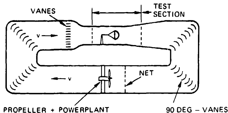
FIGURE 4-16. Closed-Throat, Full-Return Wind Tunnel.
