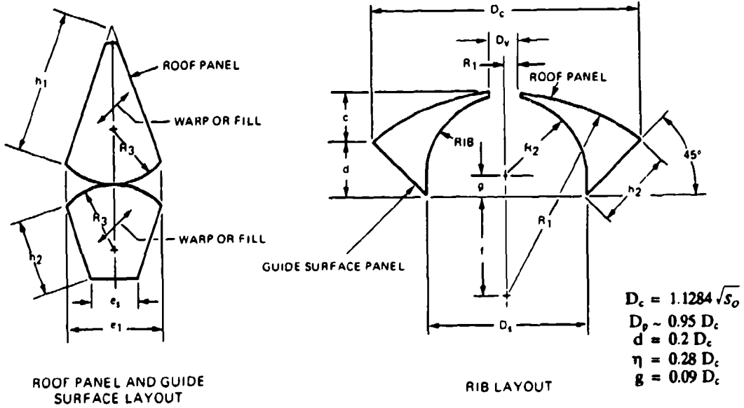
FIGURE 6-20. Ribbed Guide Surface Parachute Design.
