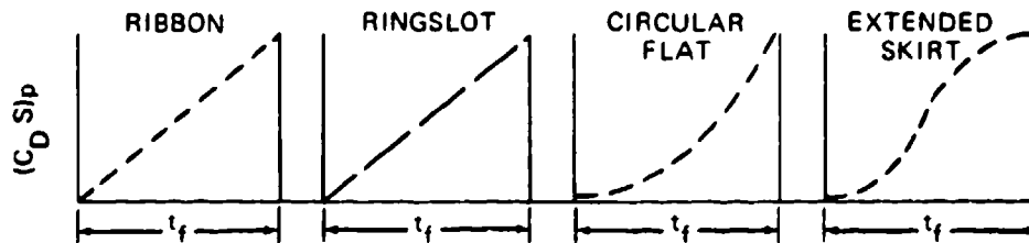
FIGURE 5-38. Typical Drag-Area-Versus-Time Increase for Various Parachute Types.
