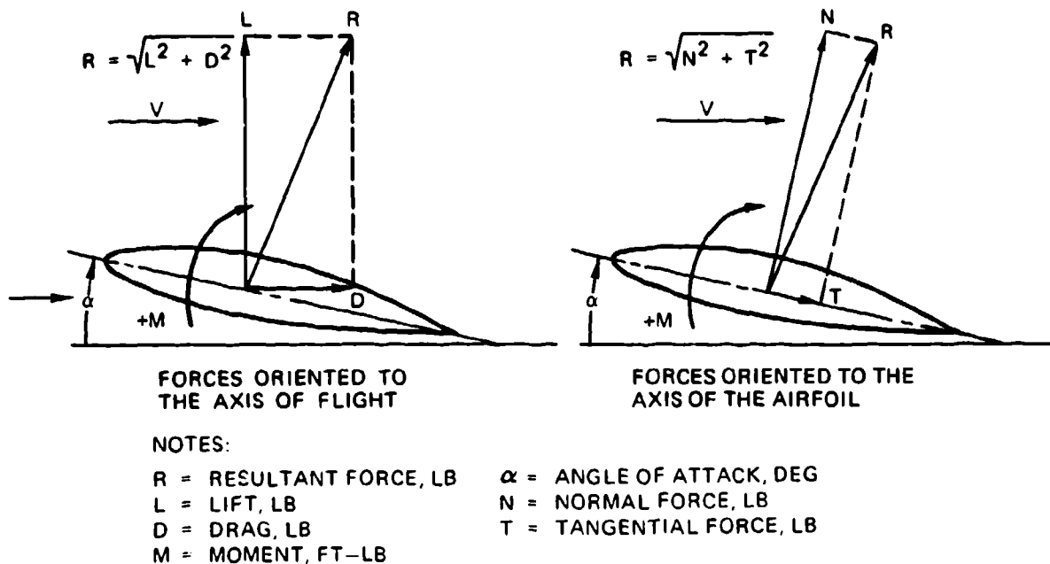
FIGURE 4-7. Aerodynamic Forces Acting on an Airfoil.
