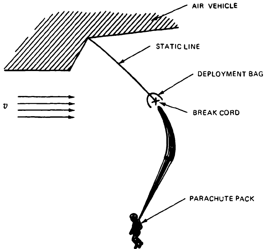
FIGURE 6-3. Parachute Static-Line Deployment.
