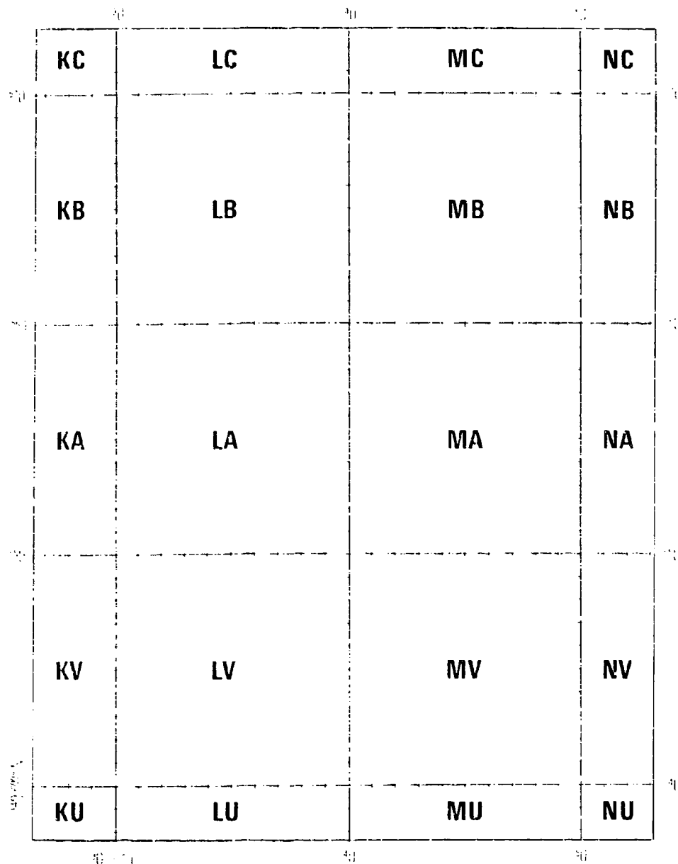
FIGURE LINE 1 AT 10000 METER INTERVALS AND DEER TICKS AT 1000 METER INTERVALS INDICATE THE UNIVERSAL TRANSVERSE MERCATOR GRID ZONE DESIGNATION 380 WORLD GEODETIC SYSTEM ELLIPSOID Scale 1:1,000,000 (in miniature)
