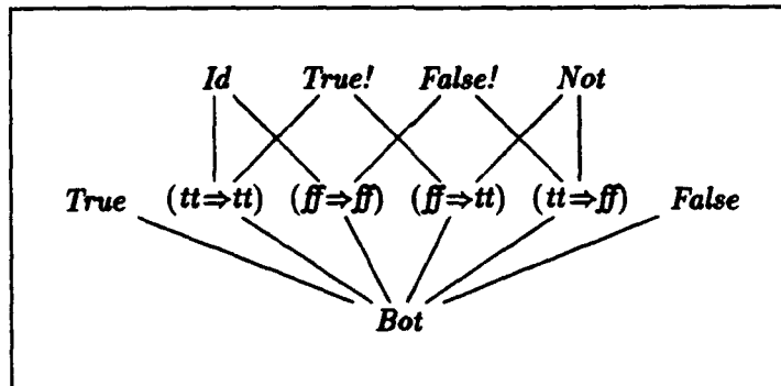
Figure 5: Stable ordering of o \rightarrow o
