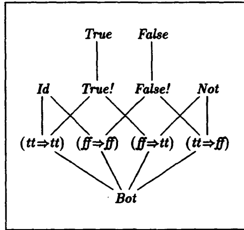
Figure 4: Pointwise ordering of o \rightarrow o
