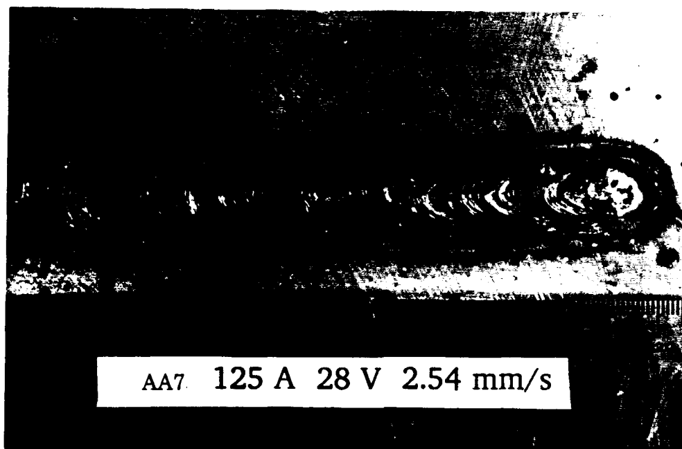
Figure 44. Bead morphology of weld AA7.
