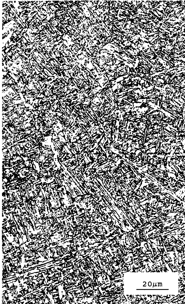
Figure 25. Light micrograph of weld HCB2.
