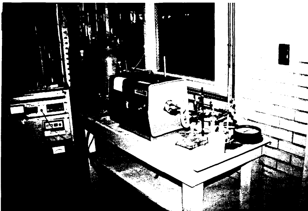
Figure 40. Experimental apparatus for the determination of electrode coating moisture content.
