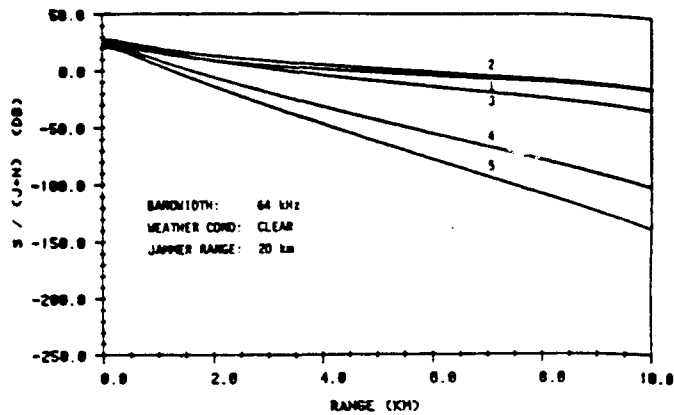
Figure E. Signal-to-(jamming + noise) vs. communications range for coherent FSK/standoff jammer in clear air.
