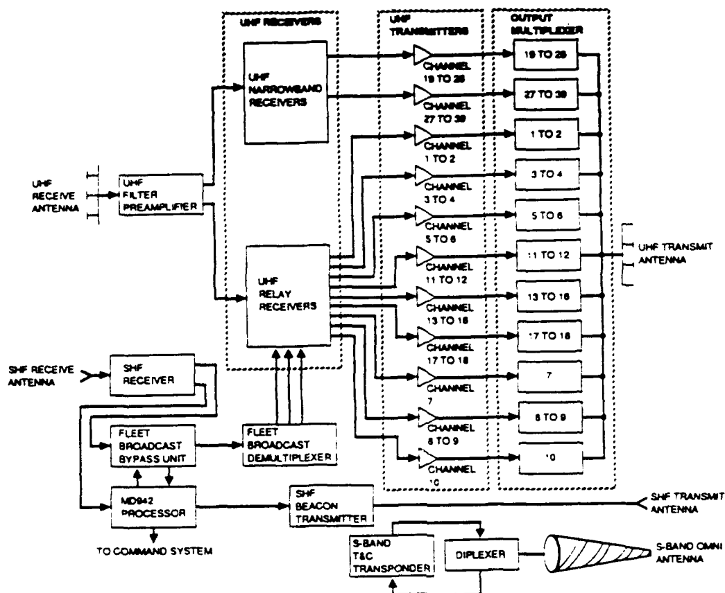
Figure II-4 Simplified Payload
