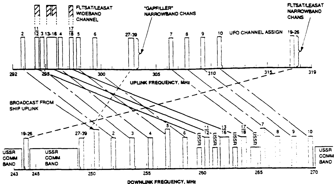
Figure IV-2 UHF Communications Frequency Plan
