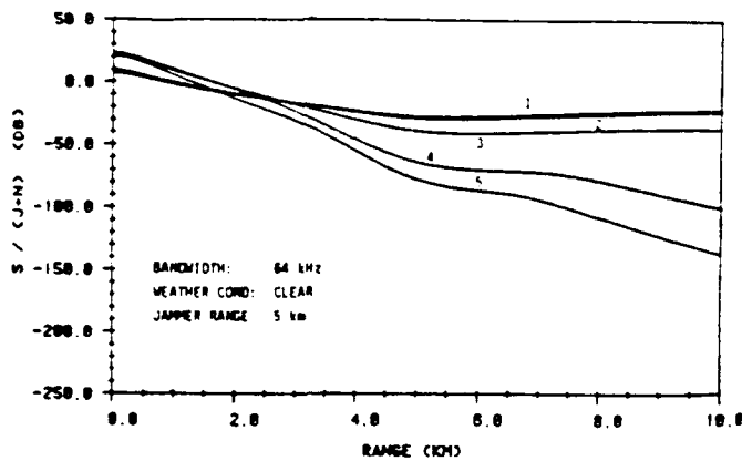
Figure G. Signal-to-(jamming + noise) vs. communications range for coherent FSK/close-in jammer in clear air.
