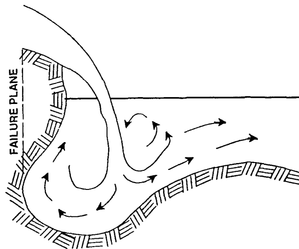
Figure 1. Conceptual Model of Scour Hole Development
