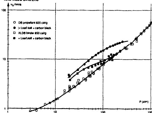
Fig. 10 DOUBLE-BASE PROPELLANT AND ACTIVE BINDER BURNING RATES
