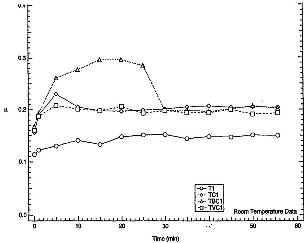
Figure 13 Friction Coefficient Versus Time (23°C)
