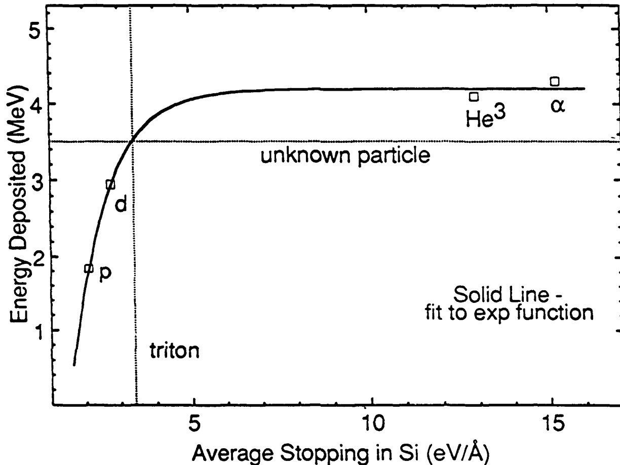
Figure 5. Energies deposited in the unbiased detector for normally incident 5-MeV ^3\text{He} , ^4\text{He} , protons and deuterons produced in a tandem Van DeGraaff accelerator are plotted against particle stopping powers in silicon averaged over the particle range. The solid line represents a least-squares fit of the data to an exponential function. The observed energy registered at zero bias by the particles detected in our experiment is shown as a horizontal dotted line. The intersection of this line with a vertical dotted line representing the average stopping power of tritium in Si and with the fitted curve suggests that a triton is the most likely candidate for the detected particles.
