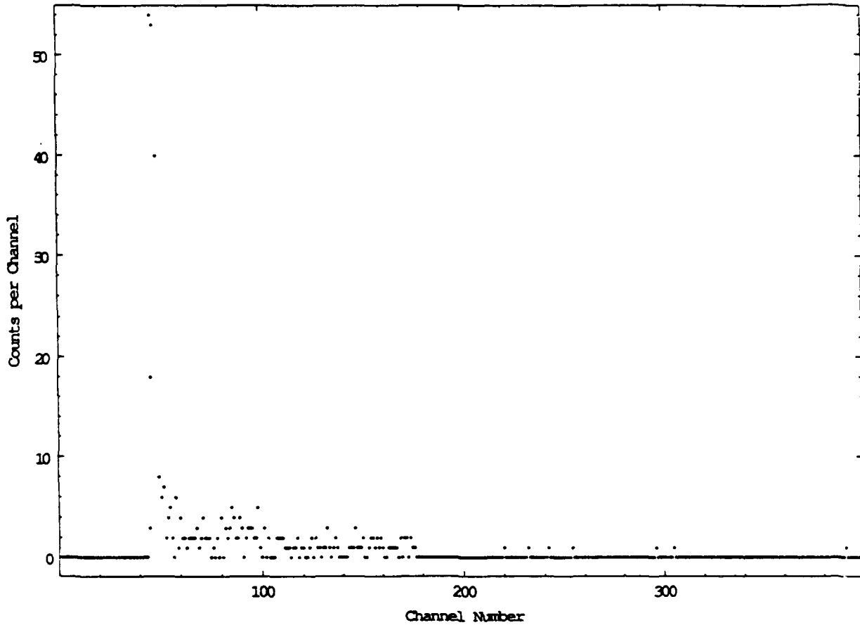
Figure 4. Spectrum acquired for a four hours during a control experiment where hydrogen ions were accelerated an energy of 500 eV at a current density of 200 \mu\text{a}/\text{cm}^2 onto a TiD 2 thin-film sample. Counts above 1 MeV are caused by arcing (voltage breakdown of the accelerator grids, see text) as observed on a storage oscilloscope. There are no peaks in the spectrum.
