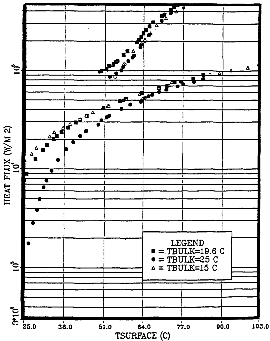
Figure 17. Subcooling.
