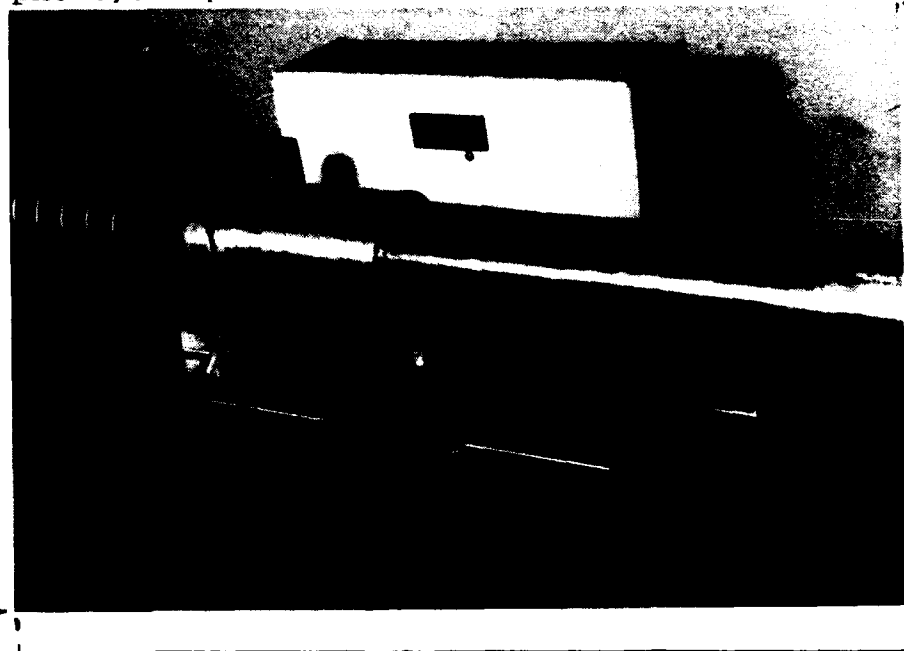
Figure 8. Axial Loading Device Installed at the Far End of the Transmitter Bar. Force is applied through a phenolic shear pin and measured using an instrumented aluminum yoke and the readout device shown in the background. The shock absorber is at the extreme left.
