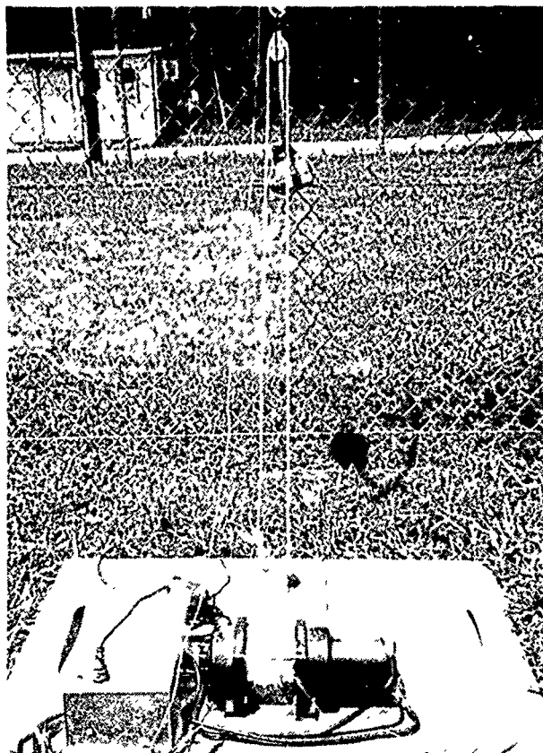
Figure 9. The winch and solenoid switch box attached to baseplate
