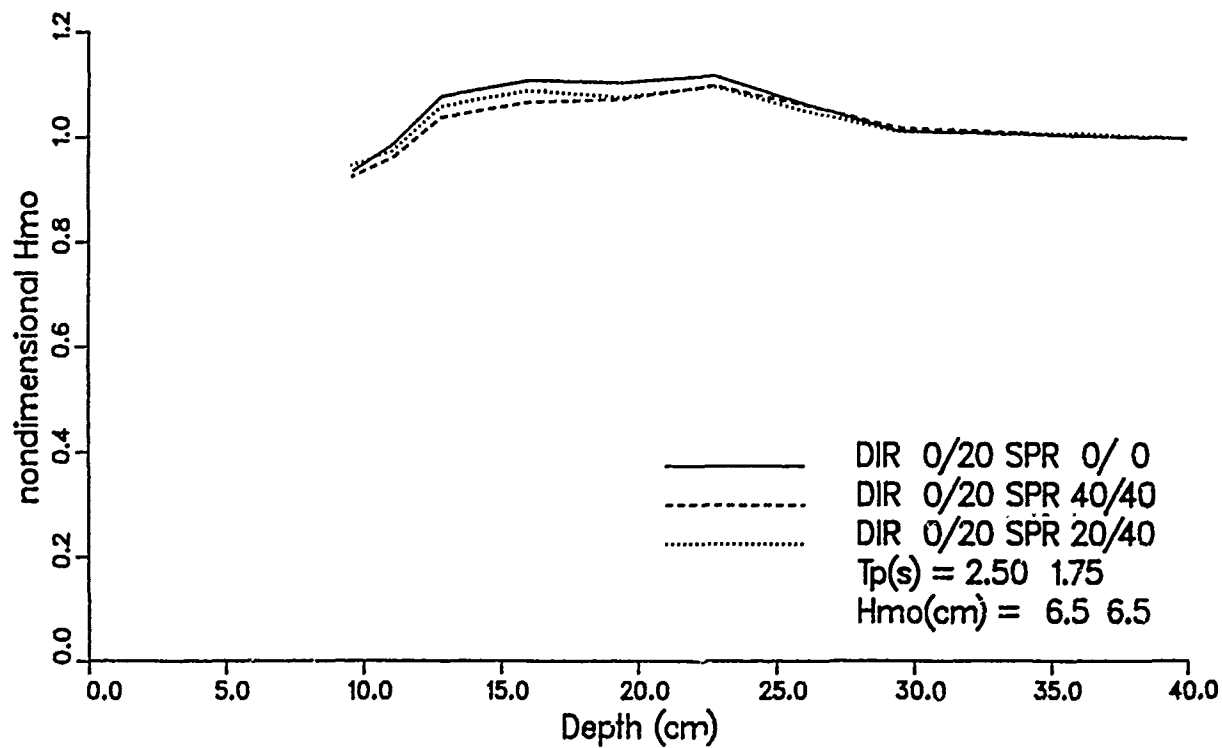
Figure 21. Initial height effect on wave height, bimodal spectra (Continued)
