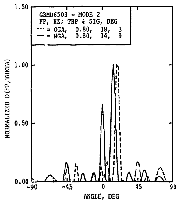
Figure 36. Formation of secondary directional peak, bimodal case D65
