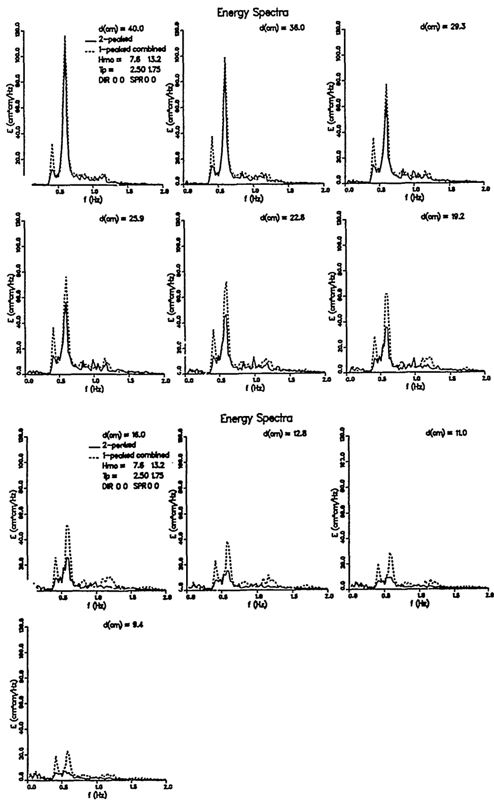
Figure 23. Linear superposition assumption effect on wave spectra (Sheet 1 of 3)
