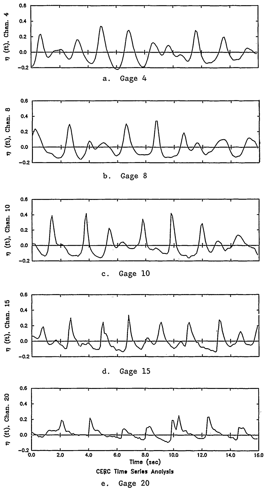
Figure 16. Measured wave profile, bimodal case D29
