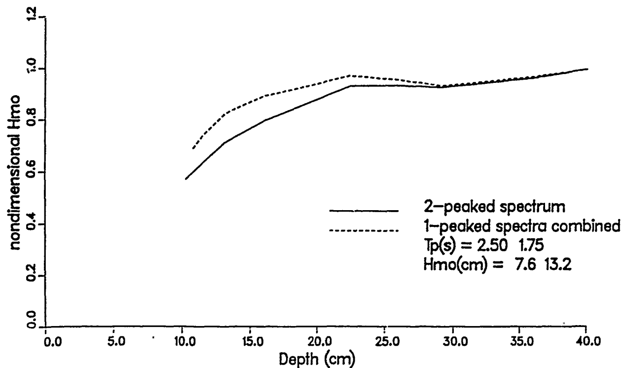
Figure 22. Linear superposition assumption effect on wave height (Sheet 1 of 3)
