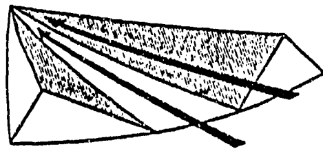
Figure 2-32d. LATE AFTERNOON. East-facing slopes begin to cool; upslope flow weakens.
