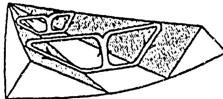
Figure 2-32f. LATE EVENING. Downslope winds dominate.
