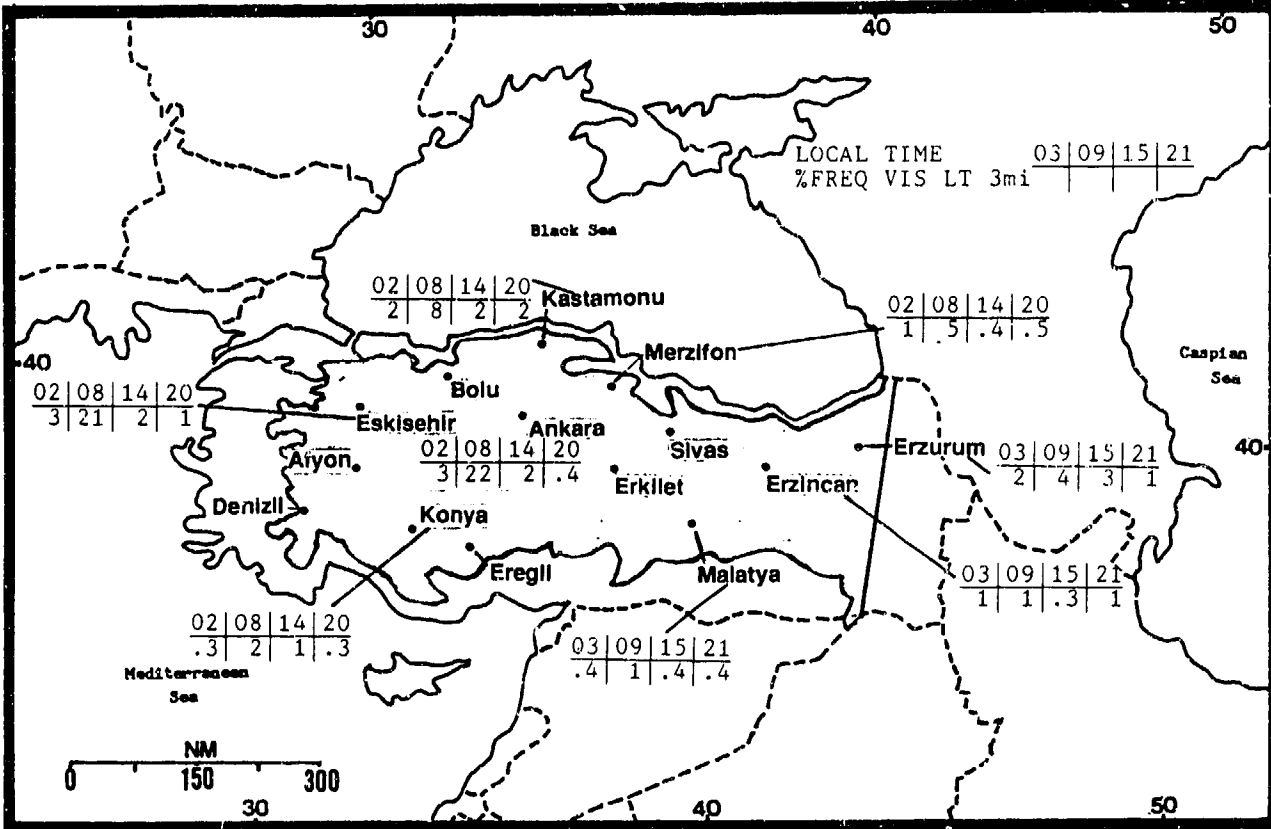
Figure 6-24a. Mean Fall Frequencies of Visibilities Below 3 Miles, Anatolian Plateau.
