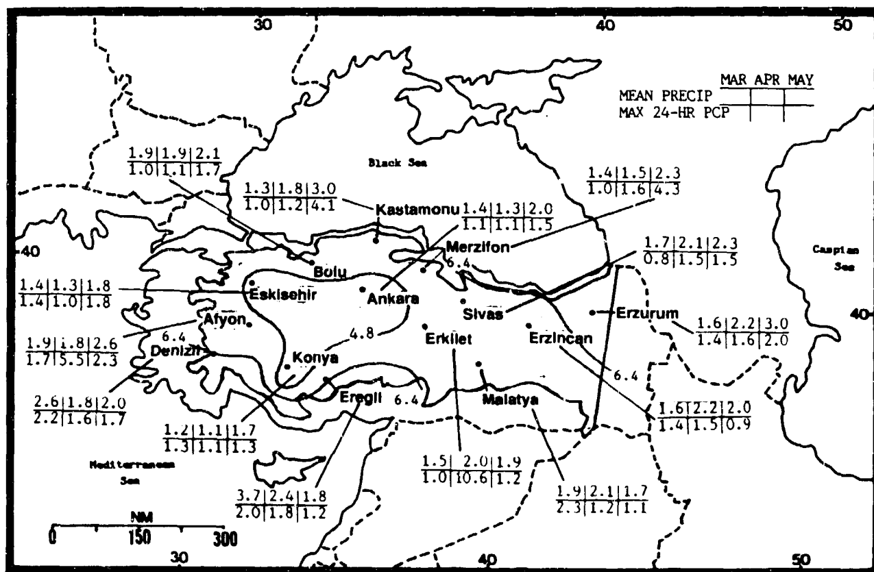
Figure 6-14a. Mean Spring Monthly/Maximum 24-Hour Precipitation (inches), Anatolian Plateau. Isoyets represent mean seasonal precipitation (water equivalent).
