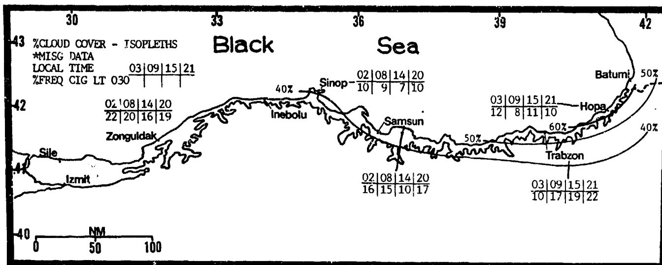
Figure 8-14. Mean Summer Cloudiness (isopleths) and Frequencies of Ceilings Below 3,000 Feet (915 meters), Black Sea Plain.
