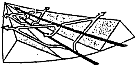
Figure 2-32c. MIDDAY. Sunshine covers the entire valley floor, and upslope flow feeds valley circulation.
