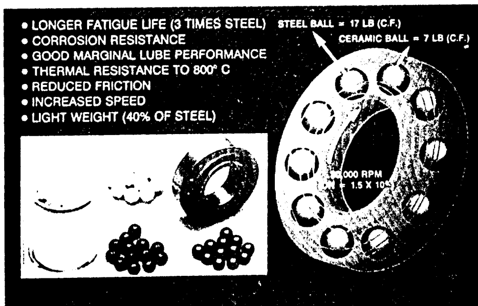
Figure 14.—Hybrid (ceramic) bearing.
