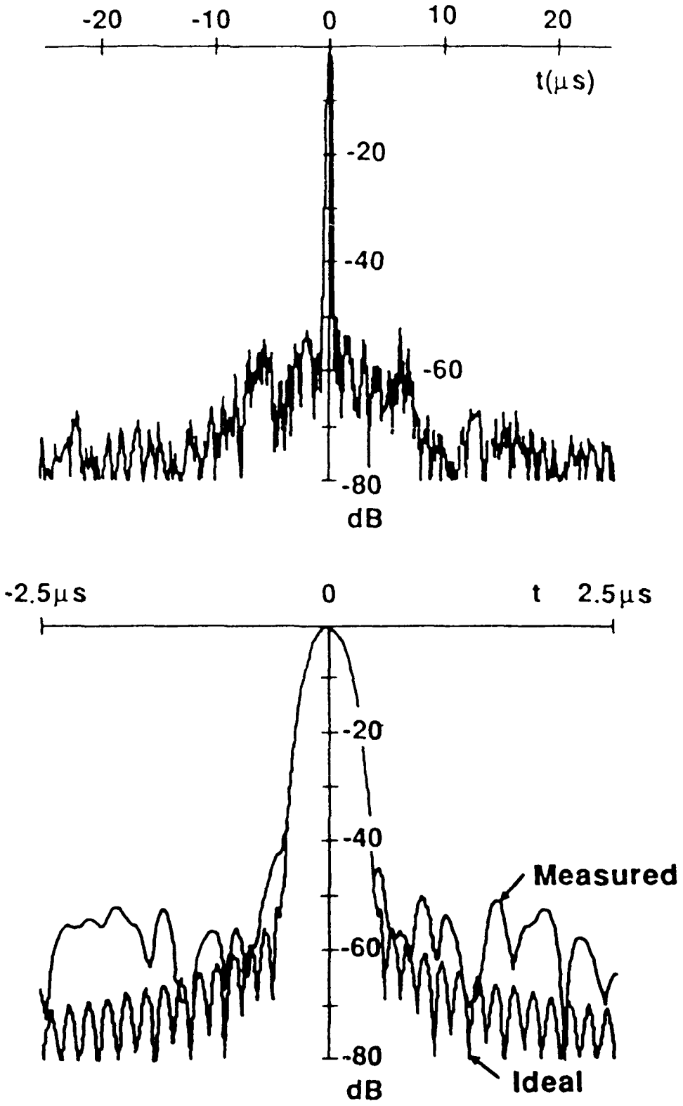
Fig.12 Response from a Kaiser-Bessel weighted line in a simulated pulse compression experiment with the direct feedthrough signal excluded. Top: response over \pm 25 \mu\text{s} relative to the main pulse. Bottom: response over \pm 2.5 \mu\text{s} relative to the main pulse for the measured line response ('measured') and the ideal line response ('ideal')
