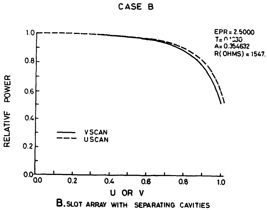
Fig.5 Array transmission factor
