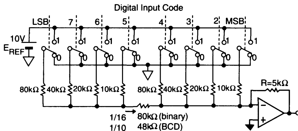
Figure 3. 8-bit digital-to-analog converter (ref. 1; reprinted by permission).
