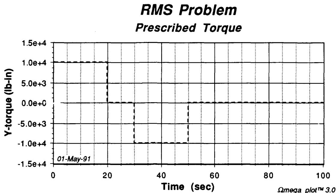
Figure 5.19. Torque time history applied to orbiter.
