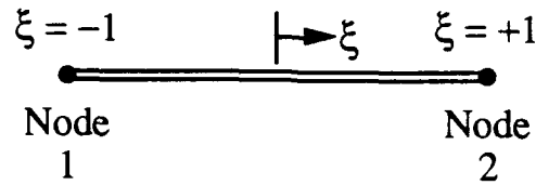
Figure 3.4. Local coordinates for 2 node beam element.
