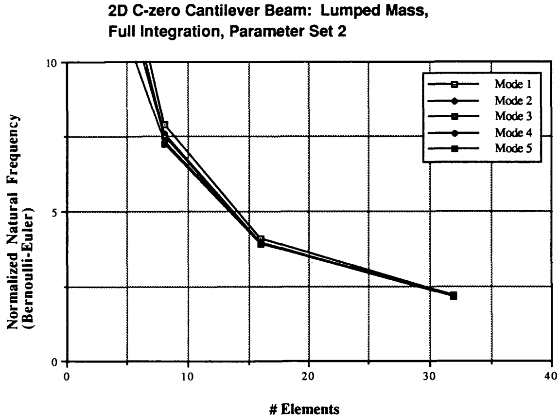
Figure 4.8. Convergence for C^0 beam, lumped mass, full integration.
