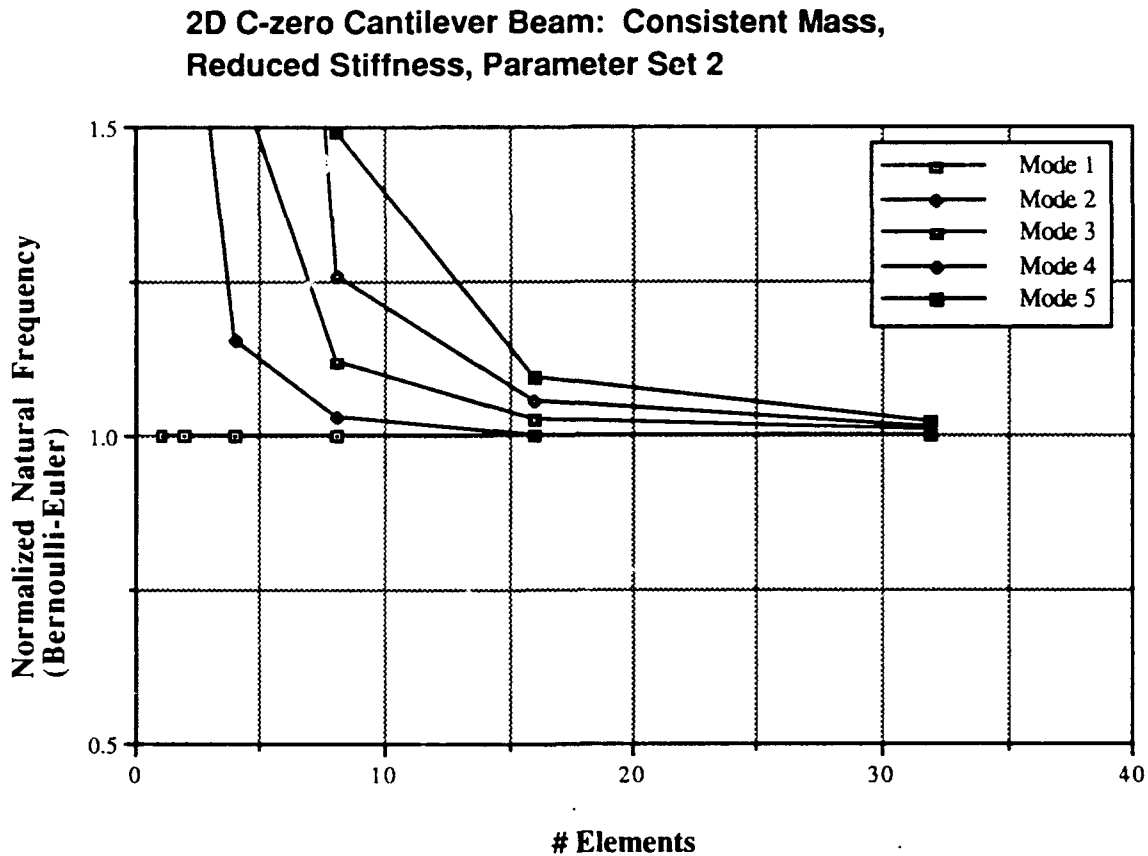
Figure 4.4. Convergence for C^0 beam, consistent mass, reduced stiffness.
