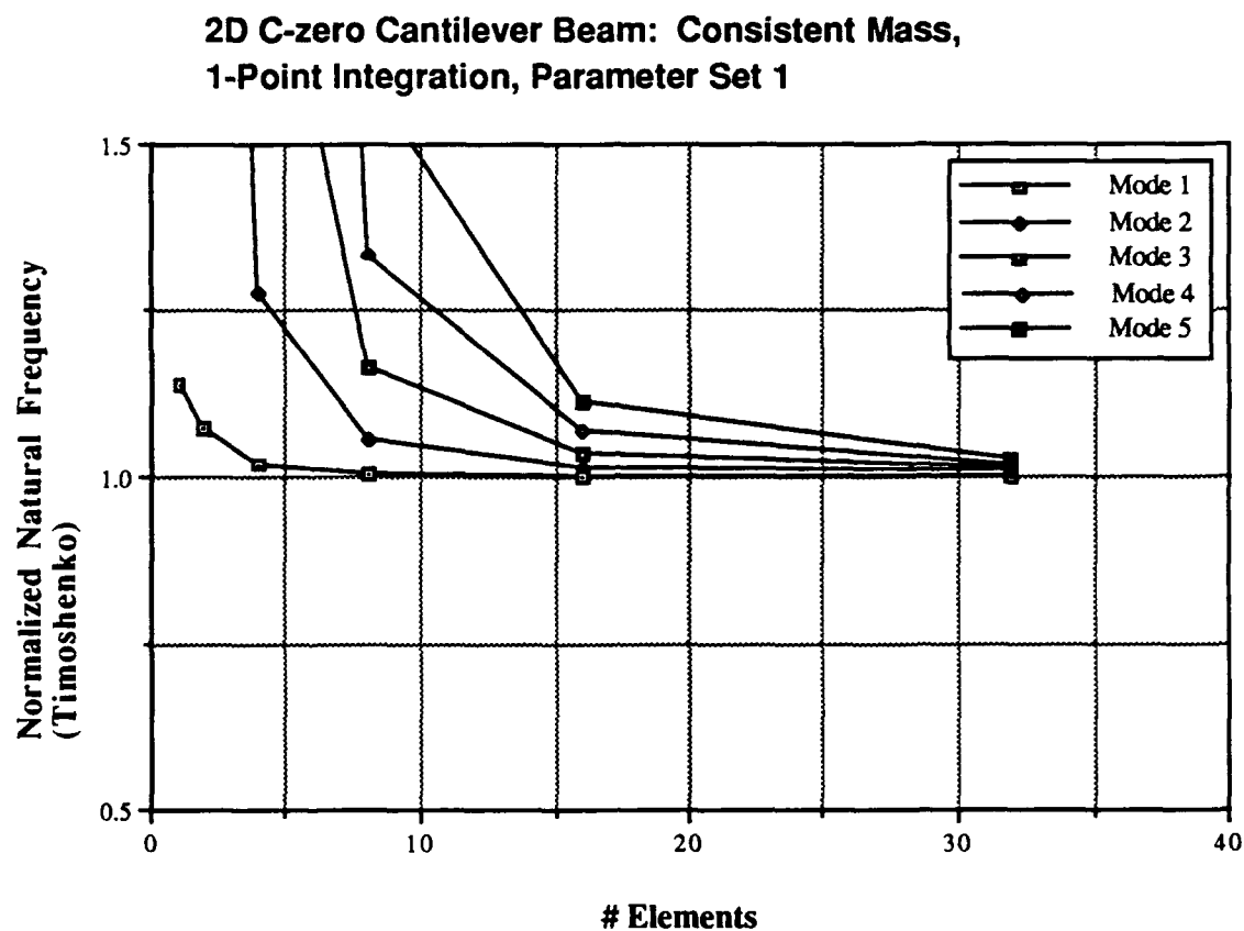
Figure E.3. Convergence plot normalized by Timoshenko frequencies; analogous to figure 4.5.
