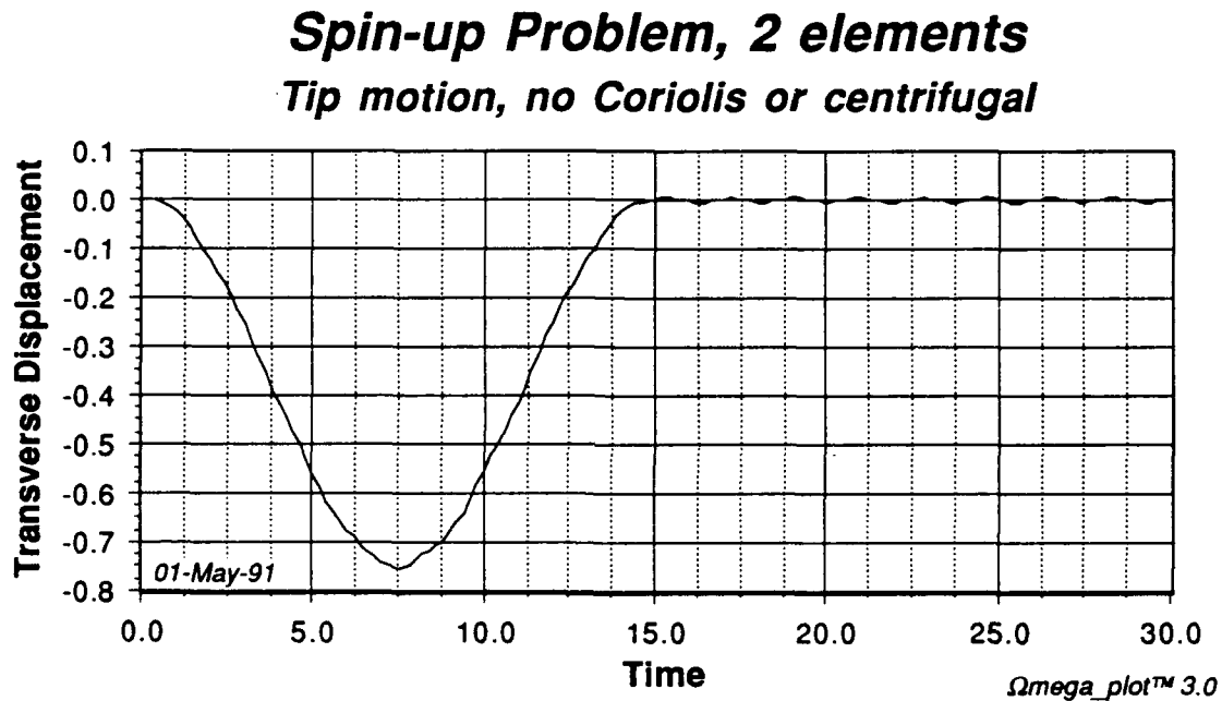
Figure 5.15. Transverse displacement of beam tip for case 3, 2 elements.
