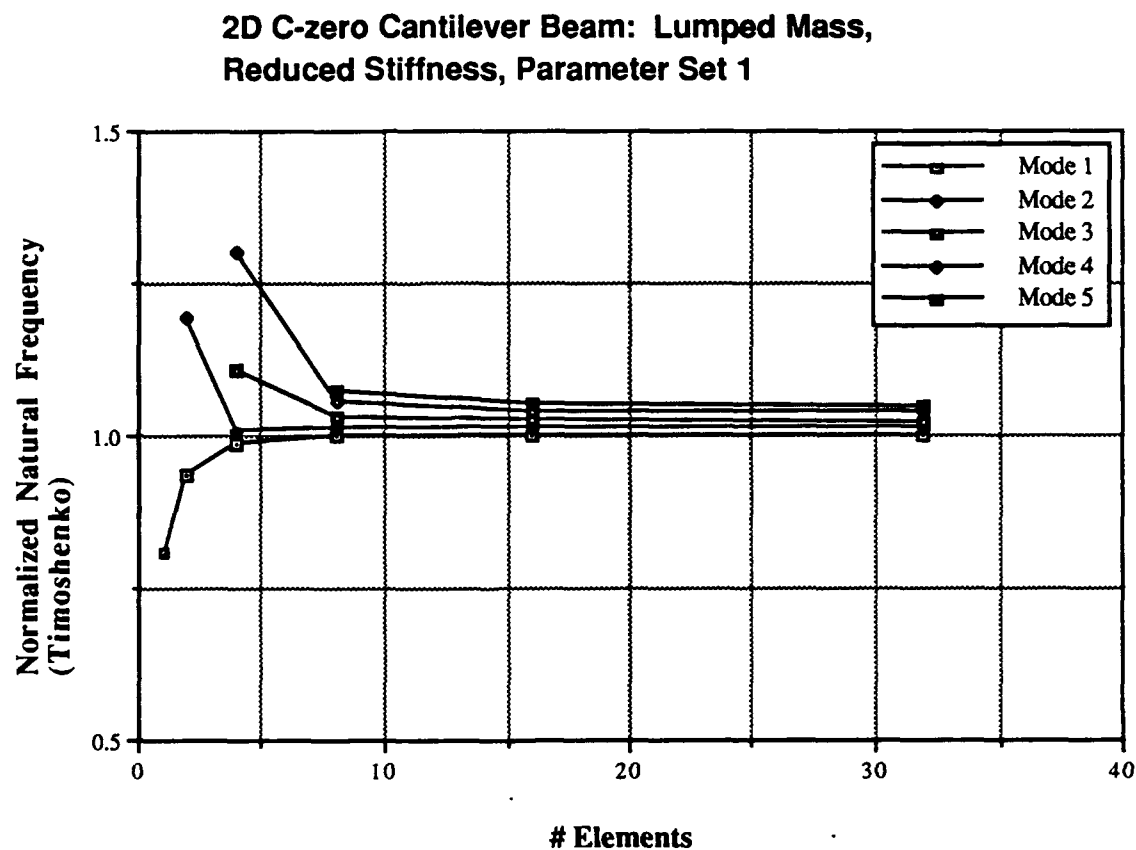
Figure E.5. Convergence plot normalized by Timoshenko frequencies; analogous to figure 4.9.
