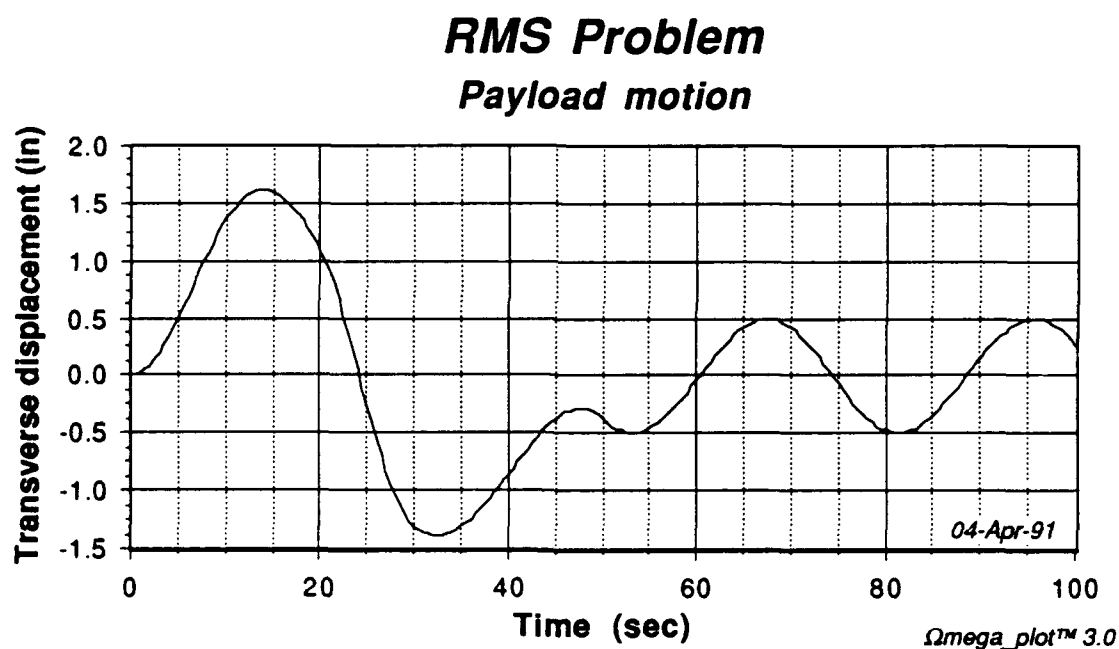
Figure 5.23. End effector response to pulse torque.
