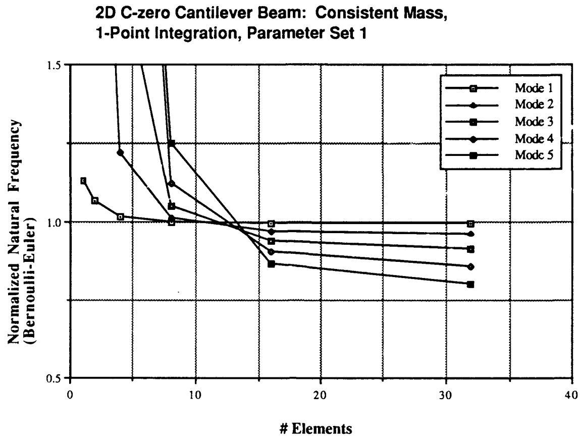
Figure 4.5. Convergence for C^0 beam, consistent mass, uniform 1-point integration.
