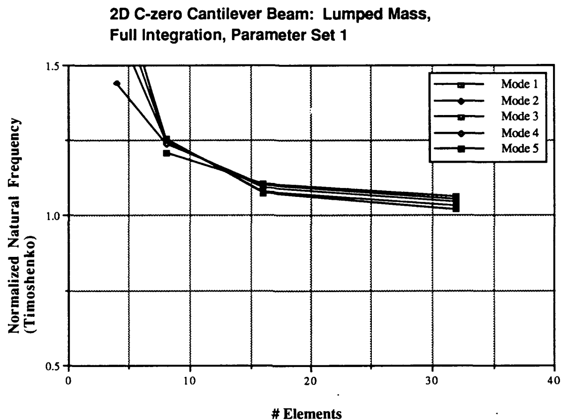
Figure E.4. Convergence plot normalized by Timoshenko frequencies; analogous to figure 4.7.
