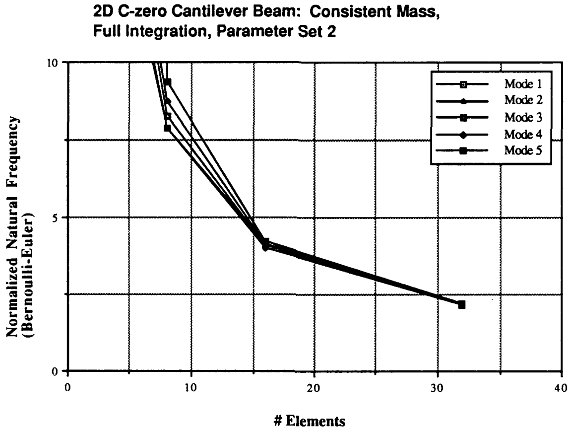
Figure 4.2. Convergence for C^0 beam, consistent mass, full integration.
