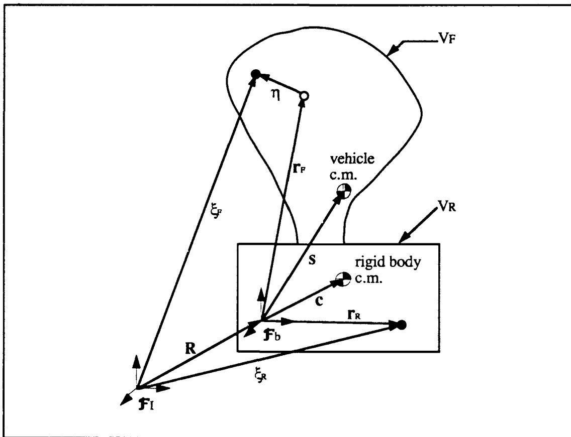
Figure 2.1. Rigid body with flexible appendage.
