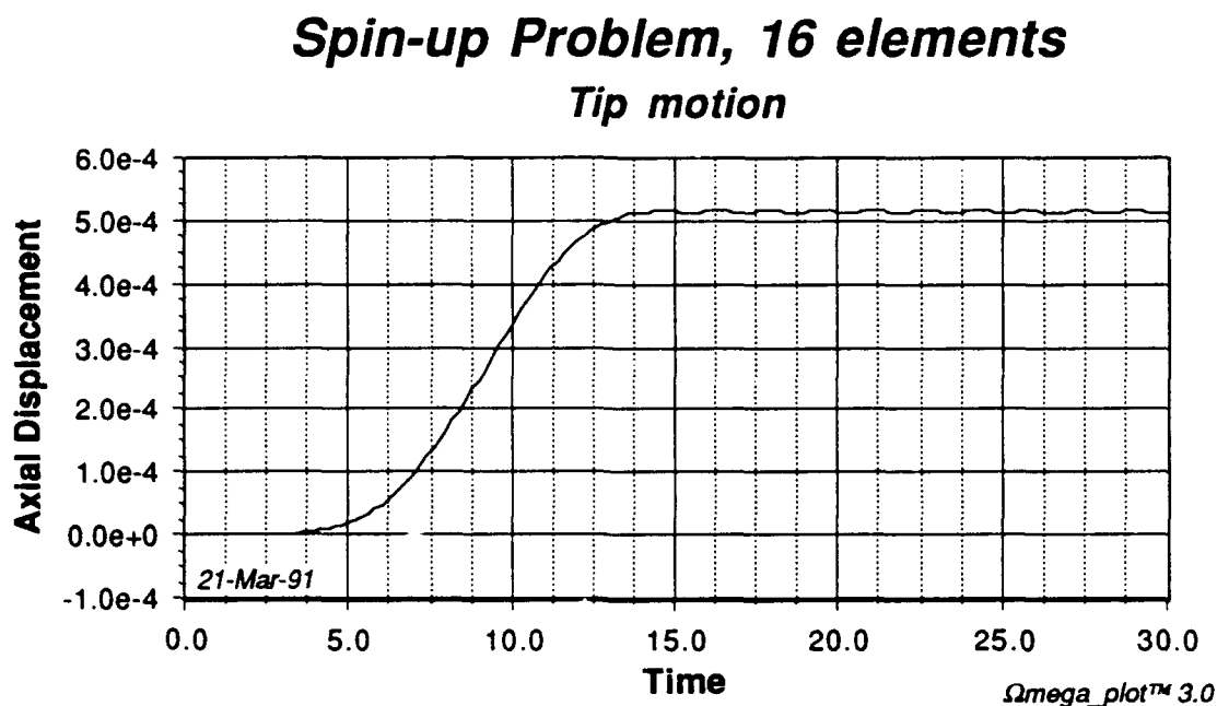
Figure 5.11. Axial displacement of beam tip for case 1, 16 elements.
