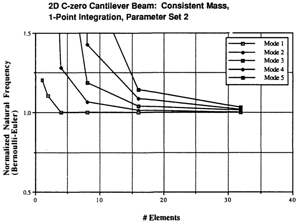
Figure 4.6. Convergence for C^0 beam, consistent mass, uniform 1-point integration.
