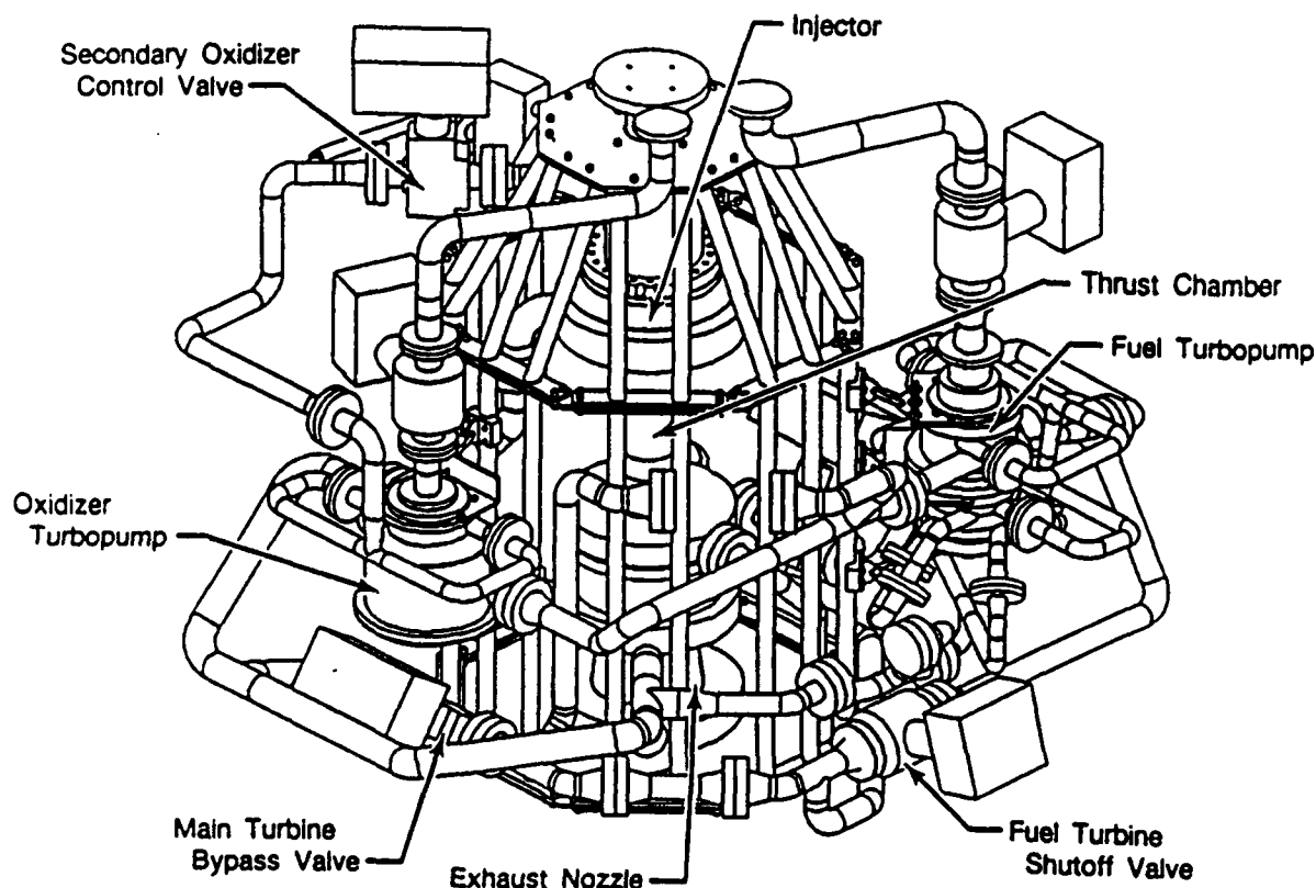
Figure 7. AETB Assembly
