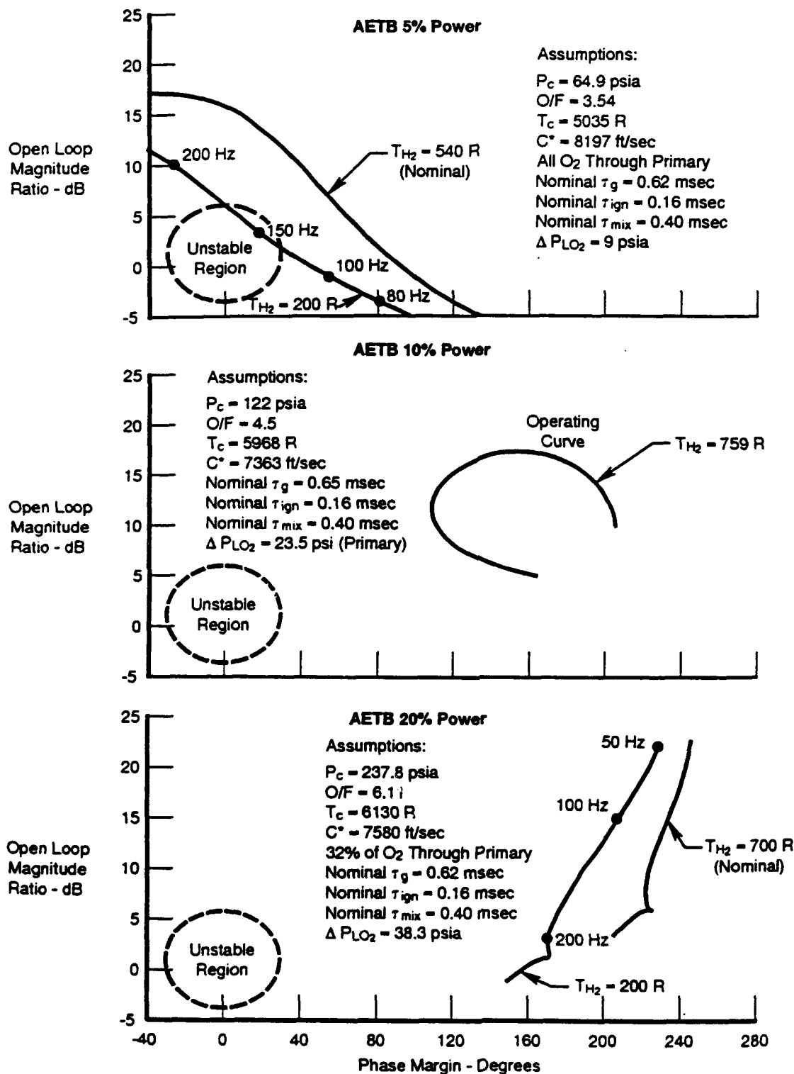
Figure 133. L-R-C Stability Curves at Power Levels of 5%, 10%, and 20%
