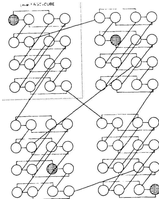
Figure 3.5 A 64-node example of a 2-RGC-CUBE. Shaded nodes (PE's) are available for expansion to higher level network.
