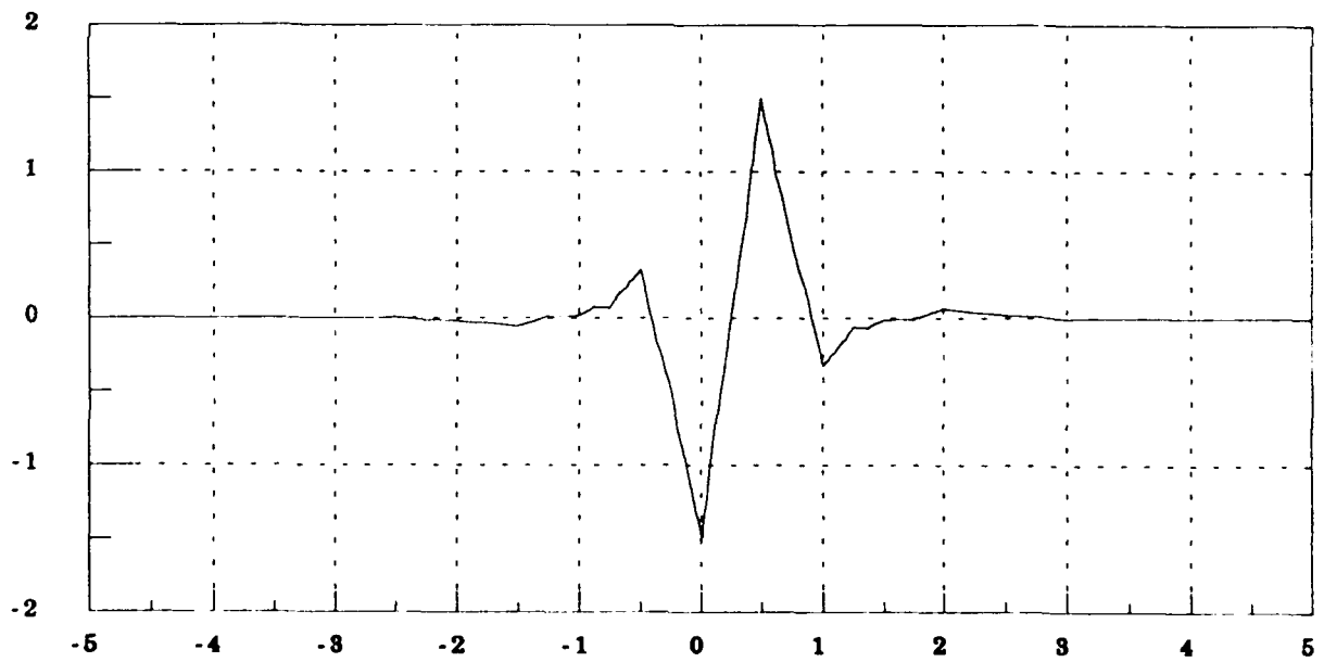
(b) \psi(x)
