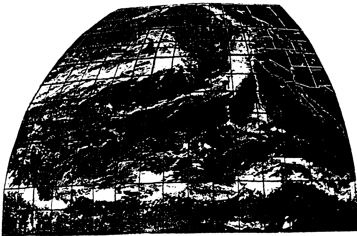
Figure 7. GOES-W visible image used to test the HSWO algorithm. Dark lines define 5°x5° squares from which cloudiness percentages are estimated.
