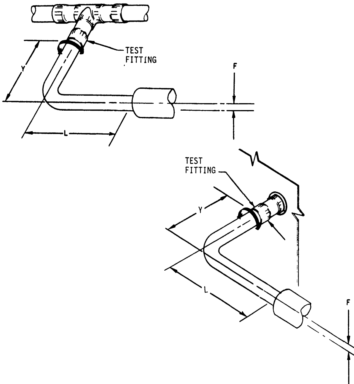
FIGURE 5. TORSION METHOD
