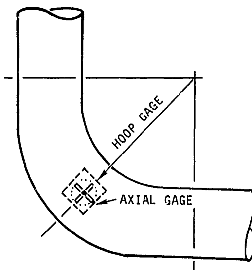
FIGURE 39: TUBE INSTRUMENTATION
