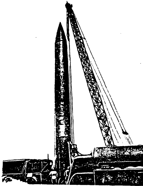
Fig. 2.6. Installation of rocket "Redstone" to vertical position.
