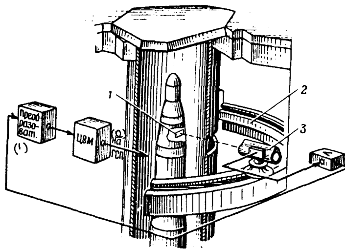
Fig. 2.14. Schematic of aiming rocket "Minuteman" during launch from silo: 1 - control mirror; 2 - live ring; 3 - azimuth scale protractor.
