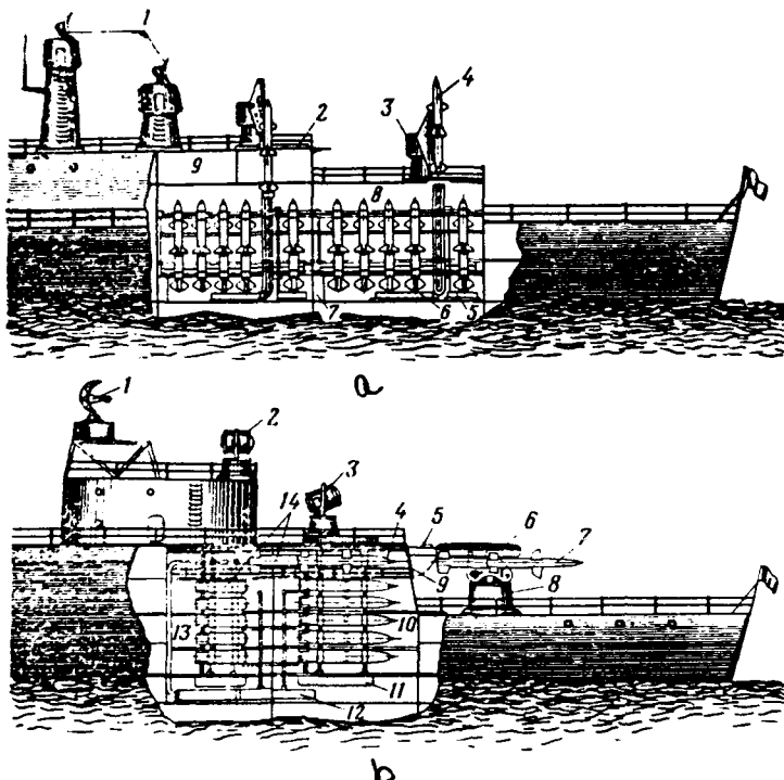
Fig. 4.8. Approximate diagram of arrangement of ZUR aboard ships: a) vertical: 1 - guidance station of ZUR; 2 - hoist system hatch-door; 3 - launcher; 4 - ZUR; 5 - mechanism of system of cross feed; 6 - mechanism of system of vertical supply; 7 - mechanism of system of longitudinal feed; 8 - magazine for storage of ZUR; 9 - post of prelaunch inspection; b) horizontal: 1 - station of target detection; 2 - tracking station of target; 3 - guidance station of ZUR; 4 - post of prelaunch servicing procedure; 5 - operational position of reversing beam; 6 - guiding; 7 - AA guided missile; 8 - launcher; 9 - cover of post of prelaunch servicing procedure; 10 and 13 - magazine; 11 - mechanism of vertical feed; 12 - mechanism of longitudinal feed; 14 - booster engines.
