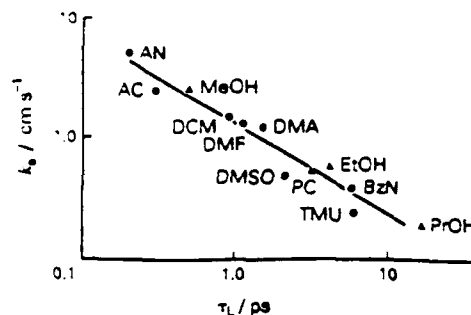
Fig. 1. Plot of the logarithm of the standard rate constant for the electroreduction of cobaltacenium cation at Hg in 12 solvents against the logarithm of the solvents' longitudinal relaxation time. Debye solvents are designated by (●) and non-Debye solvents by (▲). The abbreviations for the solvents are listed in Tables 1 and 3.
