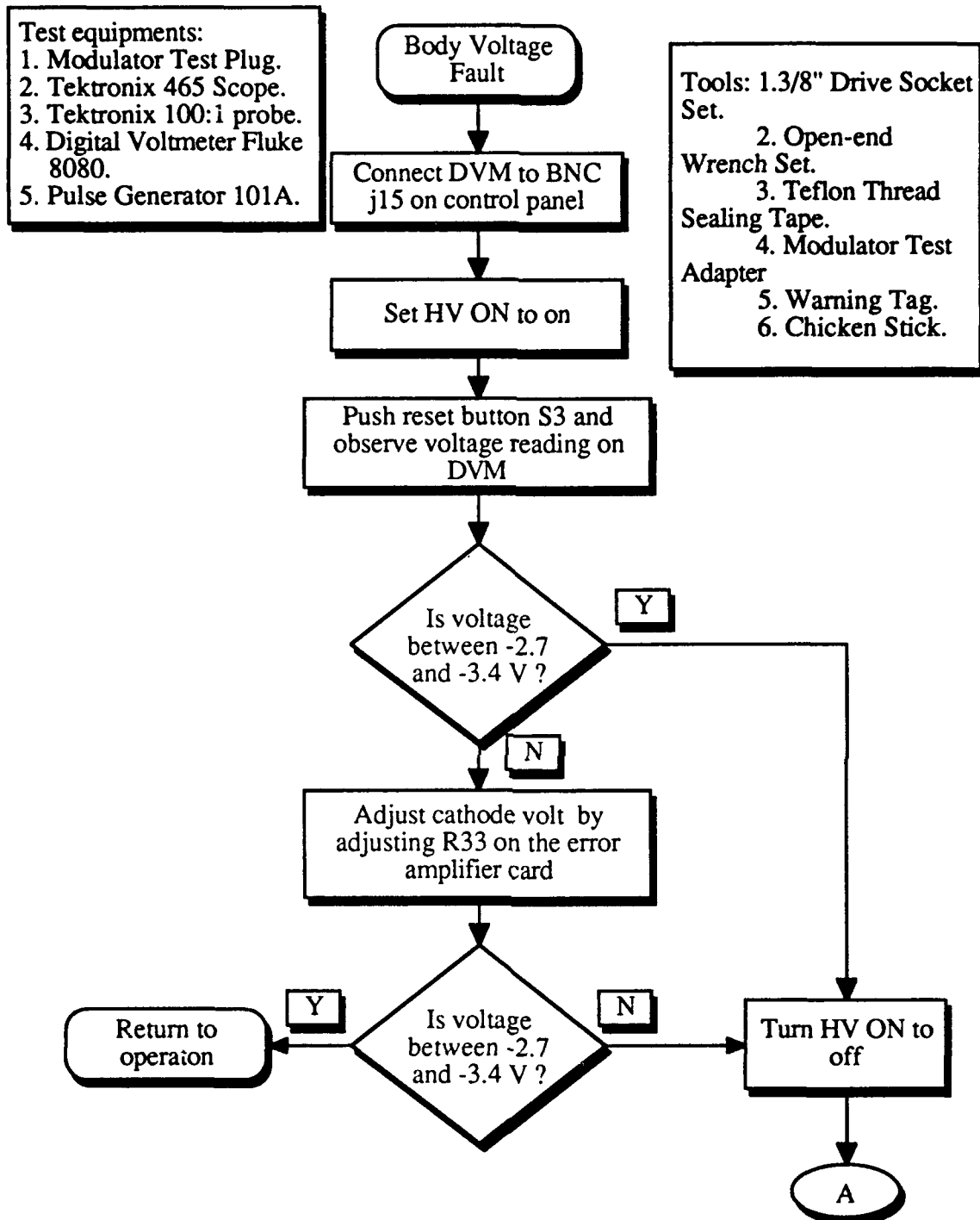
Figure B.18 Body Voltage Fault Troubleshooting Flowchart
