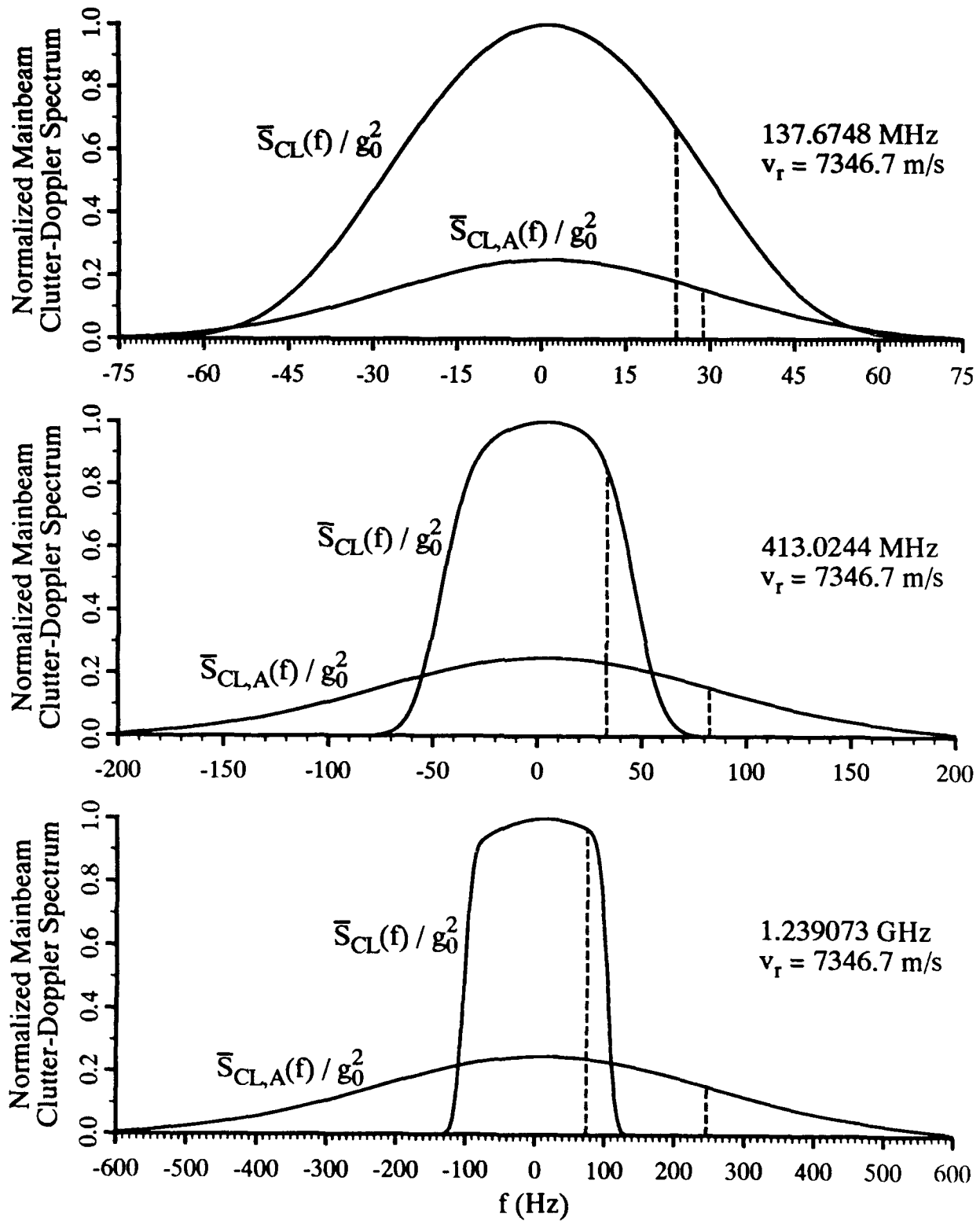
Fig. 10 — Exact and approximate mainbeam clutter-Doppler spectra for set #3 at VHF, UHF, and L-band. Both spectra are normalized to the maximum value of the exact spectrum. Twice the horizontal distance between the frequency of the maximum value of each spectrum and the vertical lines to both curves correspond to the clutter spread for each function.
