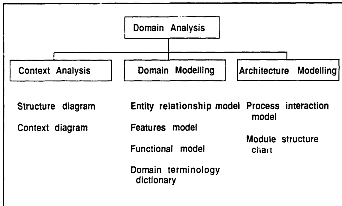
Figure 1-3: Phases and Products of Domain Analysis
