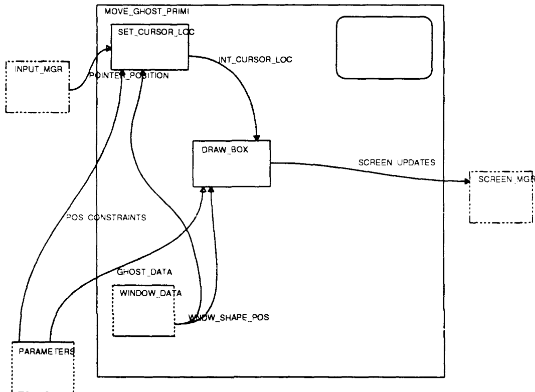
Figure 7-13: Activitychart Illustrating MOVE_GHOST Activities
