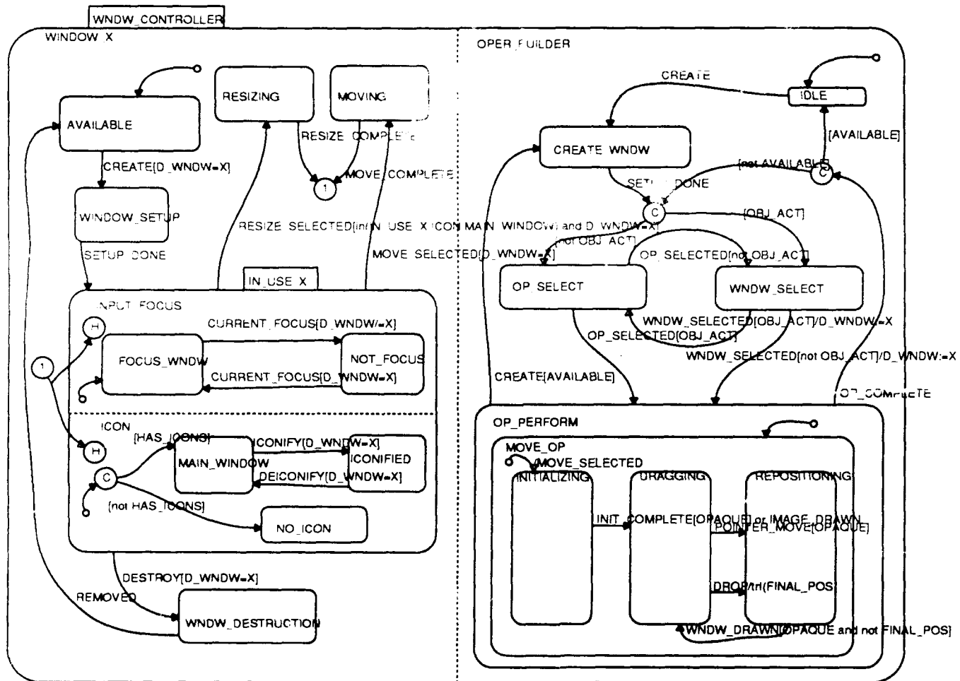
Figure 7-9: Statechart Illustrating Behavioral View of Window Manager
