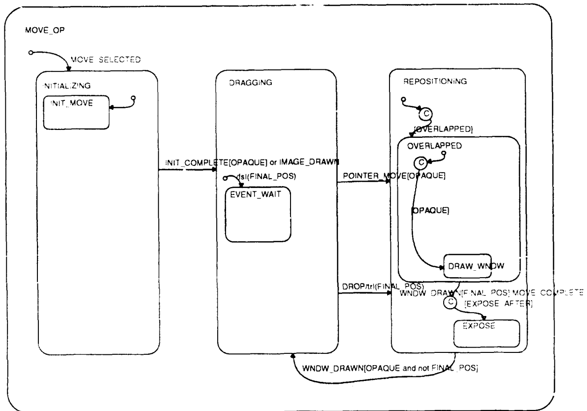
Figure 7-15: Statechart Illustrating X10/uwm Specification
