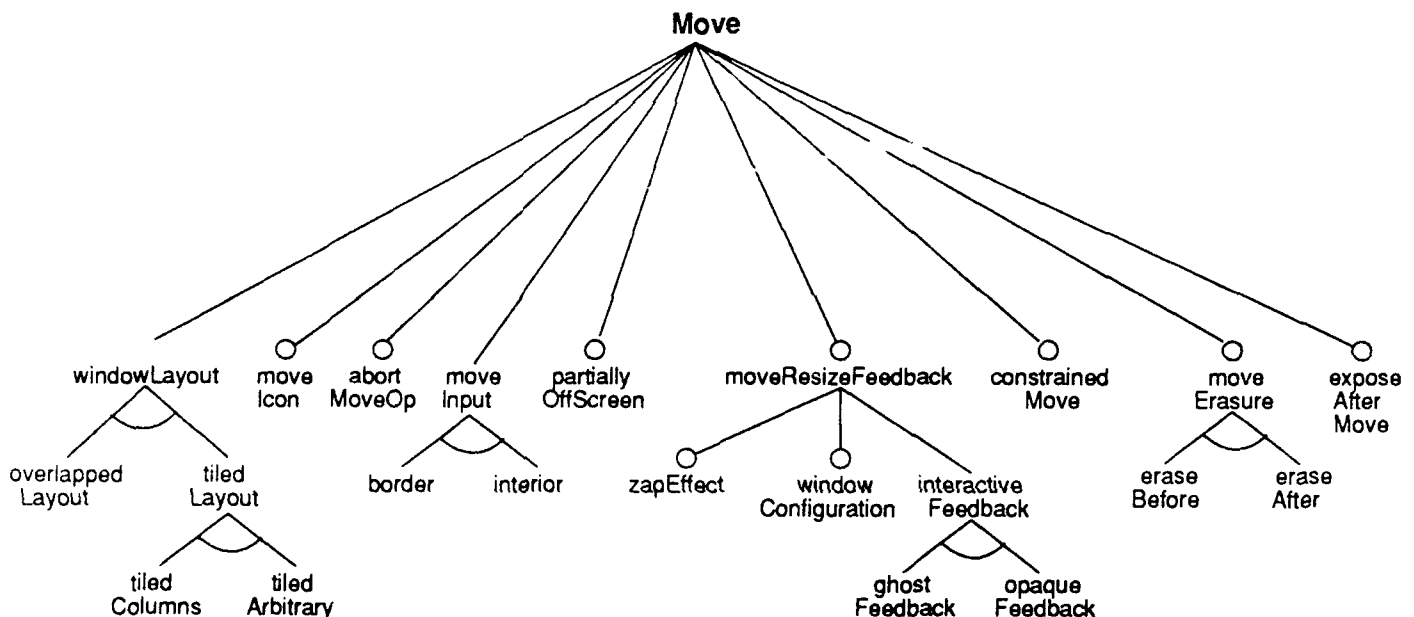
Figure 7-6: Features for the Window Manager Move Operation
