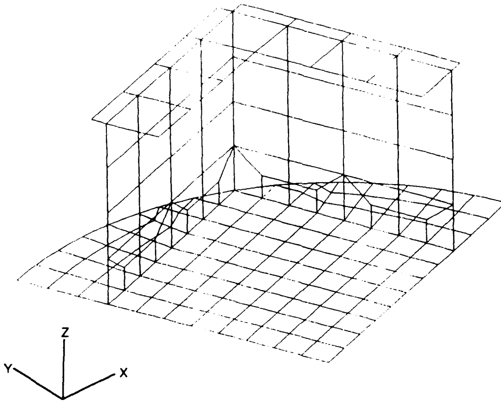
Fig. 4 — Finite element model of bulkhead test panel geometry utilizing symmetry about x and y axes
