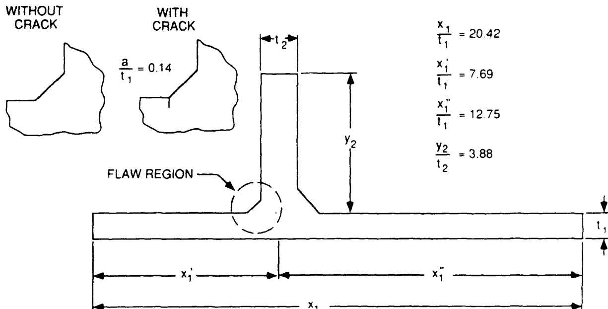
Fig. 2 — Detail of T-frame stiffener and plate intersection geometry. Displacement loading, generated from bulkhead test panel model results, was applied at material boundaries of the detail model.
