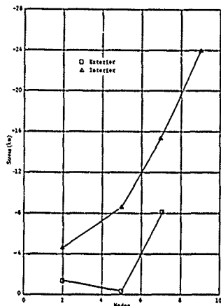
Figure 17a Hoop stresses on bottom steel plate under 500 psi hydrostatic loading
