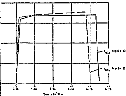
Figure 25a. Comparison of minimum strain for cycles 1 and 5 on the exterior surface of the acrylic ball in equatorial region, Rosette 10A under pressure cycles of 500 psi magnitude and 6-hour duration.
