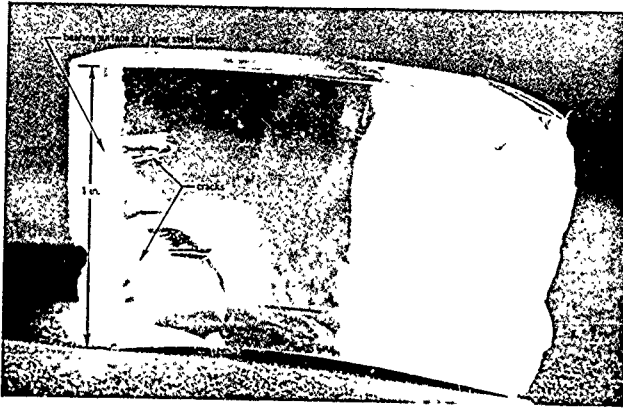
Figure E-3. Cracks in the beveled bearing surface of the polar acrylic plastic pentagon viewed at a right angle to the cut through the bearing surface. Capsule failed after 1,575 minutes of sustained loading at 3,000 psi.
