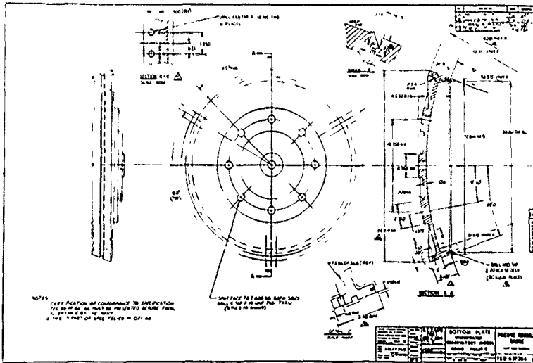
Figure 7a. Detailed dimensions of the bottom steel plate for prototype NEMO fabricated from 316 Type stainless steel
