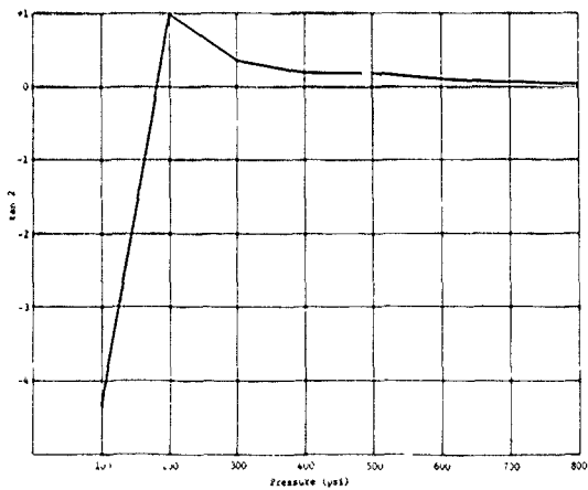
Figure 20c Change in orientation of principal strains on the interior surface of the bottom steel plate, Rosette 3A under short-term loading to 800 psi
