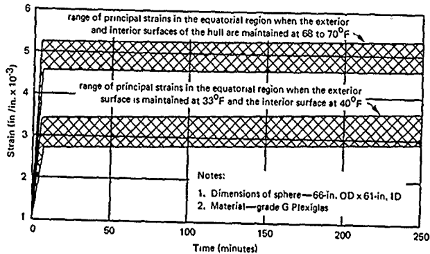
Figure 111. Effect of temperature on viscoelastic strains on interior surface of equatorial region in 66-inch-diameter capsule under 500-psi sustained hydrostatic loading.
