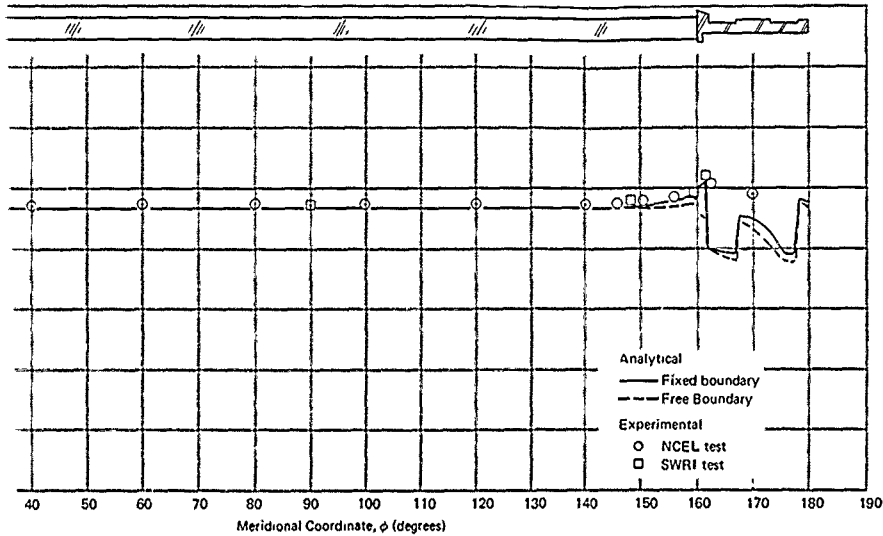
Comparison of experimental and analytical hoop stress results for external surface of acrylic plastic spherical hull.
