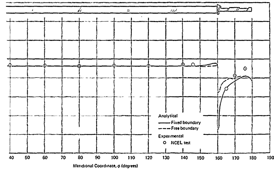
Comparison of experimental and analytical hoop stress results for internal surface of acrylic plastic spherical hull.
