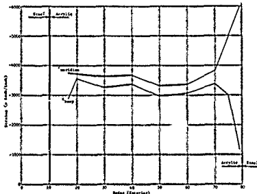
Figure 21a Distribution of long and maximum stresses on the anterior surface of sapphire ball at the beginning of the second 1-hour pressure cycle at 500 psi
