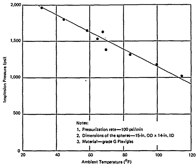
Figure 78. Implosion pressure of acrylic plastic capsule models as a function of ambient water temperature under short-term loading.
