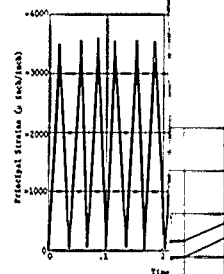
Figure 20. Cyclic strains on the inner surface of barrel; 100 psi amplitude and 1000 cycles.
