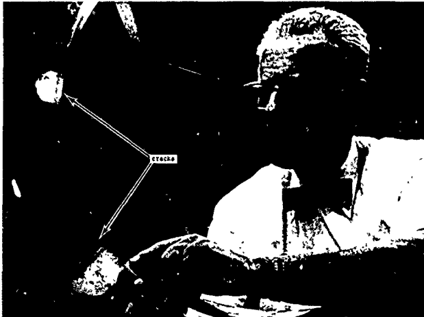
Figure 15. Typical cracks in the acrylic plastic bearing surface in contact with the hatch ring at the conclusion of Phase 4 cyclic tests; view parallel to the bearing surface.
