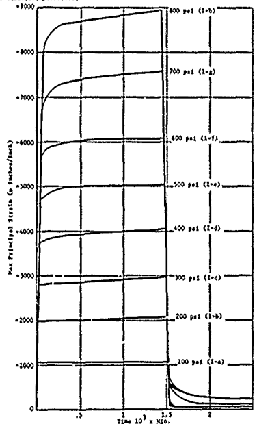
Figure 23c. Time dependent strain on the exterior surface of the acrylic hull near polar penetration; Rosette 12a under long-term hydrostatic loadings to different pressures.
