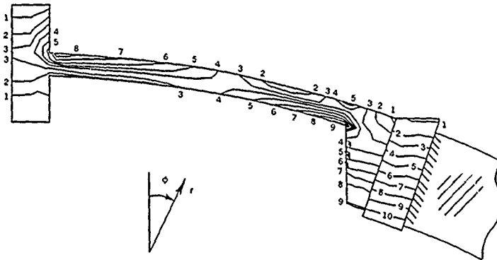
Figure 16. Effective stress contour and surface plots for top hatch for fixed boundary condition.
