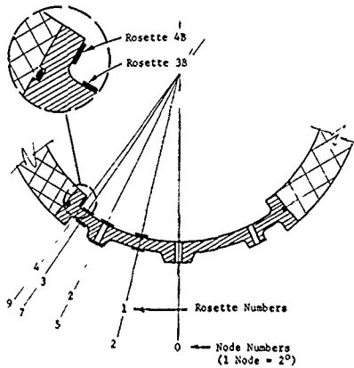
Figure 7. Location of and numbering system for rosettes on the stainless steel plate portion of the capsule.
