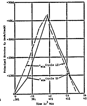
Figure 32b. Comparison of maximum and minimum strains for cycles 1 and 2 on the interior surface of the acrylic hull in equatorial region; Resette 12B under pressure cycles of 500 psi magnitude and 2-minute duration.
