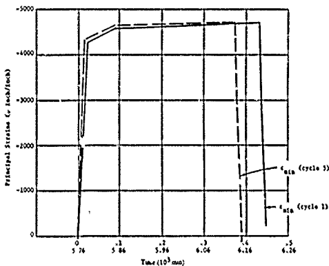
Figure 25f. Comparison of minimum strain for cycles 1 and 5 on the interior surface of the acrylic ball in equatorial region, Rosette 10B under pressure cycles of 500 psi magnitude and 6-hour duration.
