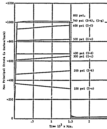
Figure 24a. Time dependent strain on the internal surface of the bottom steel plate; Rosette 38 under long-term hydrostatic loadings to different pressures.
