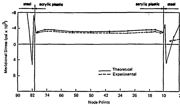
(a) Meridional stresses on the exterior surface.
