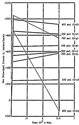
Figure 24b. Time dependent strain on the internal surface of the bottom steel plate flange; Rosette 49 under long-term hydrostatic loadings to different pressures.
