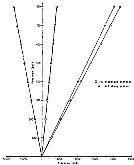
Figure 19a Typical stresses on the exterior of acrylic hull in the equatorial region, Rosette 12A under short-term loading to 800 psi
