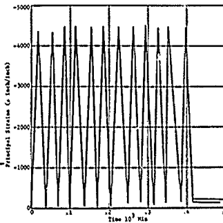
Figure 31b. Cyclic strains on the interior surface of the acrylic hull in equatorial region; Resette 12B under pressure cycles of 500 psi magnitude and 2-minute duration.
