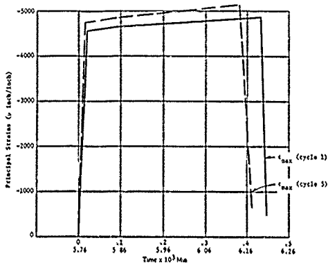
Figure 25c. Comparison of maximum strain for cycles 1 and 5 on the interior surface of the acrylic ball in equatorial region, Rosette 10B under pressure cycles of 500 psi magnitude and 6-hour duration.
