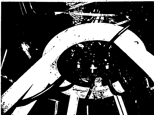
Figure 76. Cables and cable feedthroughs in the steel polar penetration closure for the strain gage instrumentation on the 66-inch-diameter capsule.
