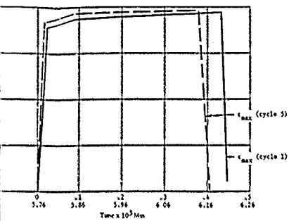
Figure 22c. Comparison of maximum strain for cycles 1 and 5 on the exterior surface of the acrylic ball in equatorial region, Rosette 10A under pressure cycles of 500 psi magnitude and 6-hour duration.
