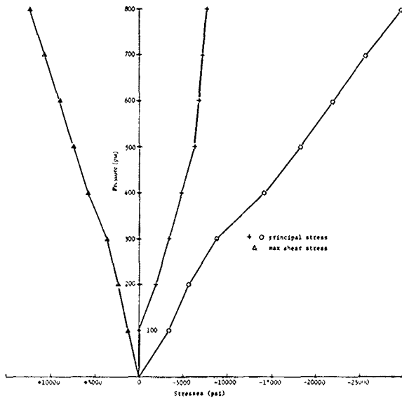
Figure 20a Stresses on the highest stressed location on the interior surface of bottom steel plate, Rosette 3B under short-term loading to 800 psi
