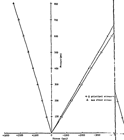
Figure 19b Typical stresses on the interior of acrylic hull in the equatorial region, Rosette 12B under short-term loading to 800 psi
