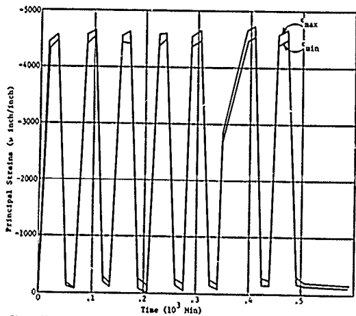
Figure 29c. Cyclic strains on the interior surface of the acrylic hull in equatorial region; Rosette 10B under pressure cycles of 5000 psi magnitude and 15-minute duration.
