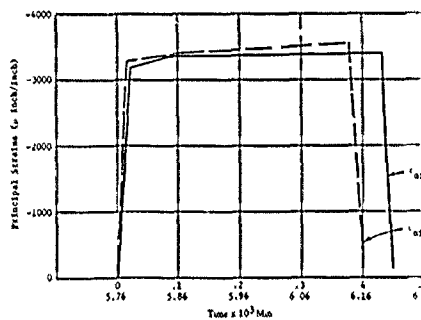
Figure 25d. Comparison of minimum strains for cycles 1 and 5 on the exterior surface of the acrylic hull in equatorial region, Rosette 10A under pressure cycles of 500 psi magnitude and 6-hour duration.
