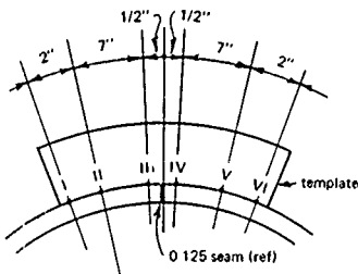
Typical Section Through Joint of Pentagon
