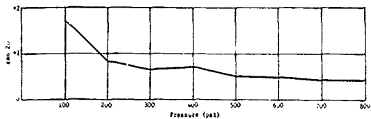
Figure 19c Change in orientation of principal strains on the exterior surface of the acrylic hull in equatorial region, Rosette 12A under short-term loading to 800 psi
