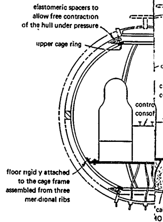
Figure 11. Internal cage restraint inside the acrylic plastic capsule.
