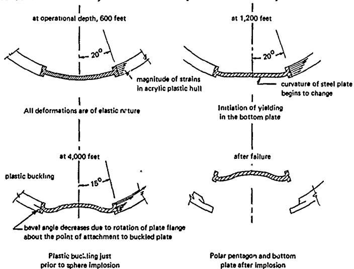
Figure 36b. Mechanism of spalling in the bottom polar acrylic pentagon reconstructed from observation of deformation in the bottom steel plate and fracture in the bottom polar acrylic pentagon.
