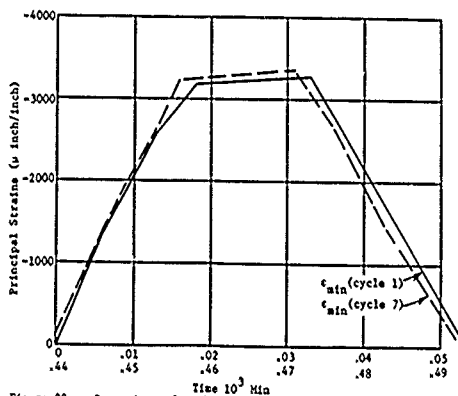
Figure 29b. Comparison of maximum and minimum strains for cycles 1 and 7 on the exterior surface of the acrylic hull in equatorial region; Rosette 10A under pressure cycles of 500 psi magnitude and 15-minute duration.
