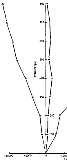
Figure 20b Stresses on the in flange, Rosette 4B
