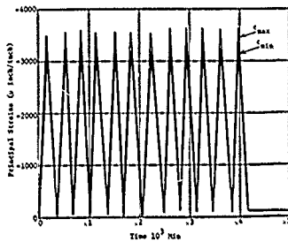
Figure 31a. Cyclic strains on the exterior surface of the acrylic hull in equatorial region; Resette 12A under pressure cycles of 500 psi magnitude and 2-minute duration.
