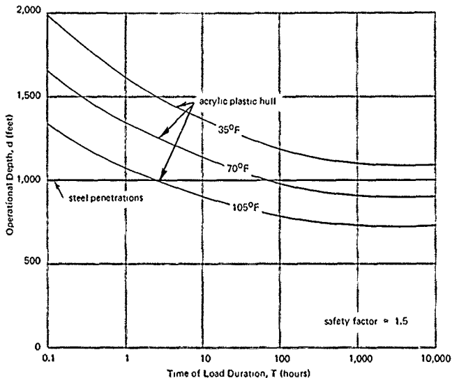
Figure 22. Operating depth curves for the acrylic plastic spherical pressure hull.
