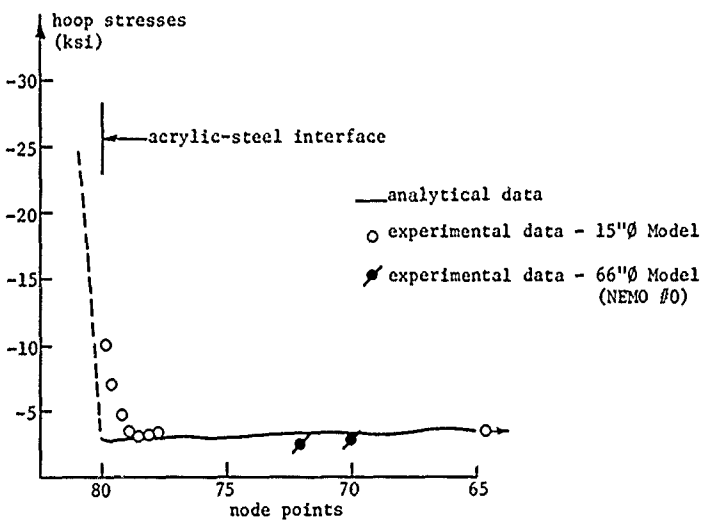
Figure 4. Comparison of Analytically and Experimentally Determined Stresses on Internal Surface of Hull in Immediate Vicinity of Hatch Opening; 500 psi Hydrostatic Pressure.
