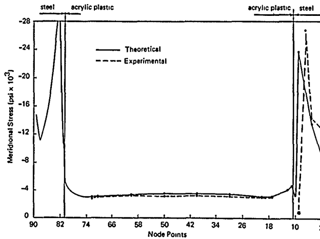
(b) Meridional stresses on the interior surface.
