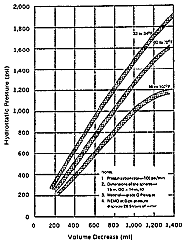
Figure 79. Change in displacement of acrylic plastic capsule models as a function of hydrostatic pressure under short-term loading.
