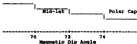
B: The ionospheric polar cap transition at night.
