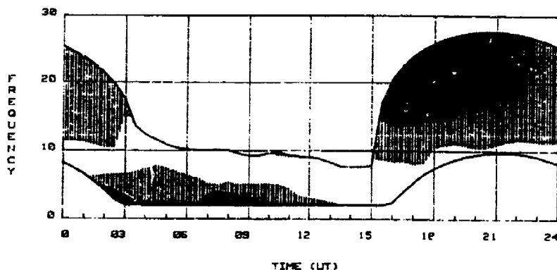
Figure 3.2.2 24-hour secure communications display. Top curve represents the MUF, bottom curve LUF. Solid shading indicates both no direction finding and no intercepts; light shading indicates one or two intercepts; no shading indicates three or more intercepts (permitting direction finding)
