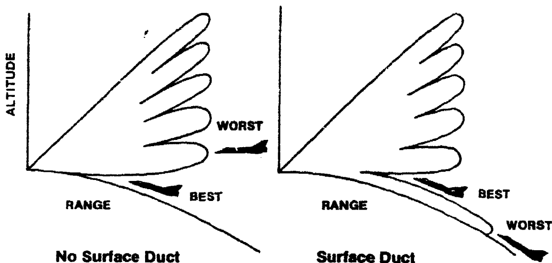
Figure 2.30. Tactical use of radar coverage diagram.
