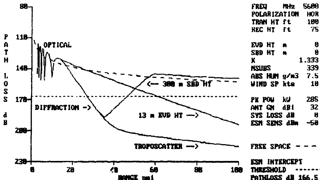
Figure 2.31. Sample PROPR display for a C-band radar showing intercept ranges for a standard atmosphere, a 13 m evaporation duct, and a 300 m surface-based duct.
