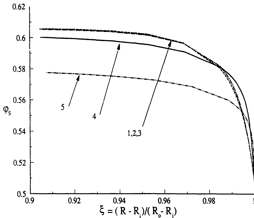
Fig.11 Profile of fiber volume fraction within the outer boundary-layer for the following cases: 1) C_r^o = 1.478 = \text{const kPa} , 2) 1.478 \text{ kPa} \leq C_r \leq 1.476 \text{ MPa} , 3) 1.478 \text{ kPa} \leq C_r \leq 14.76 \text{ MPa} , 4) 1.478 \text{ kPa} \leq C_r \leq 147.6 \text{ MPa} , 5) 1.478 \text{ kPa} \leq C_r \leq 1.476 \text{ GPa} . The number of layers n is held constant at 100.
