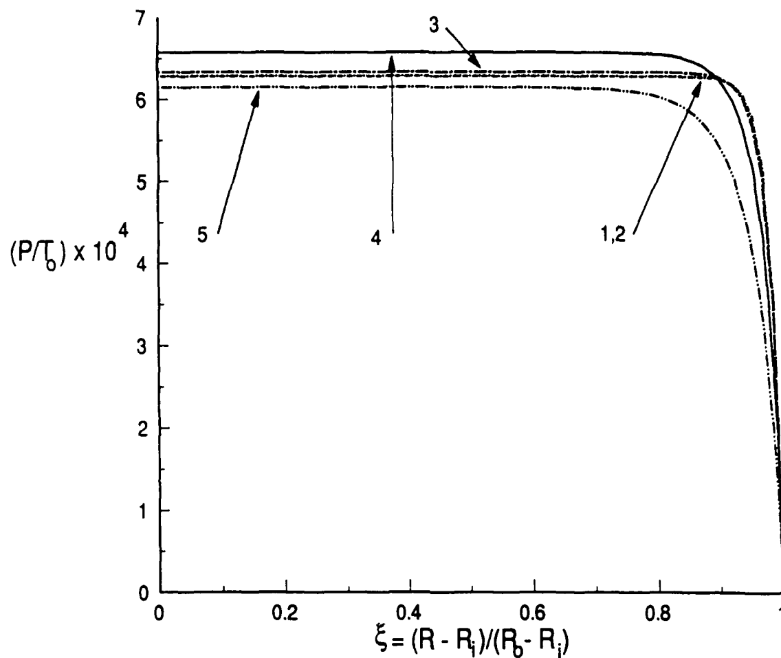
Fig.14 Radial variation of the resin pressure for the following cases: 1) C_r^0 = 1.478 = \text{const kPa} , 2) 1.478 \text{ kPa} \leq C_r \leq 1.476 \text{ MPa} , 3) 1.478 \text{ kPa} \leq C_r \leq 14.76 \text{ MPa} , 4) 1.478 \text{ kPa} \leq C_r \leq 147.6 \text{ MPa} , 5) 1.478 \text{ kPa} \leq C_r \leq 1.476 \text{ GPa} . The number of layers is held constant at 100.
