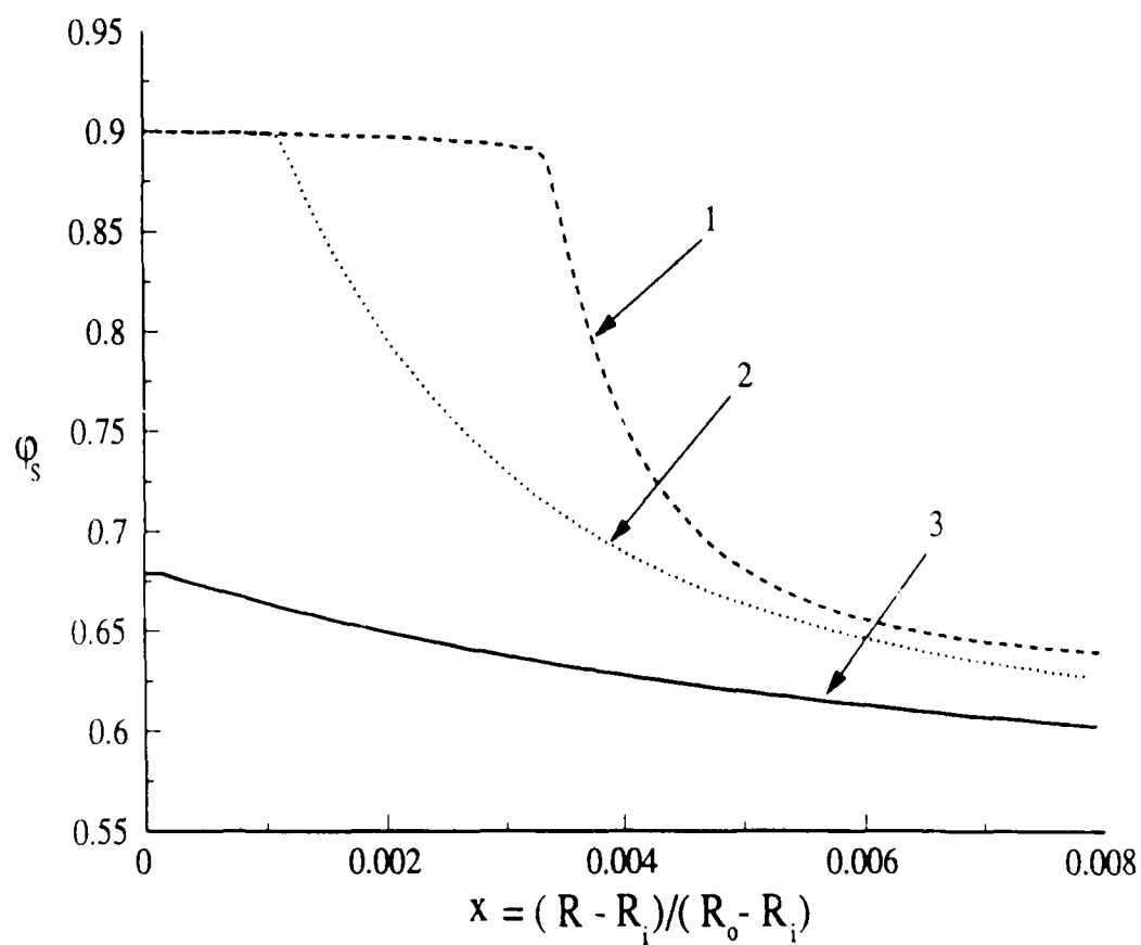
Fig.5 Profile of fiber volume fraction in the boundary-layer at the rigid interface between the mandrel and the composite. C_r = \text{const.}
