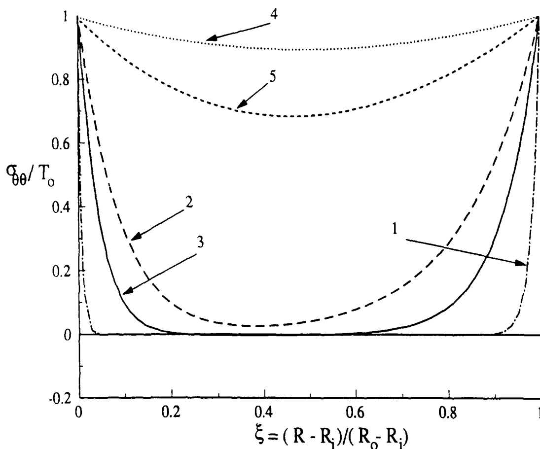
Fig.6 radial variation of the non-dimensional hoop stress for the following cases: 1) C_{rr}^o = 14.75 kPa and n = 100 layers, 2) C_{rr}^o = 1.475 MPa and n = 50 layers, 3) C_{rr}^o = 1.475 MPa and n = 100 layers, 4) C_{rr}^o = 0.1475 GPa and n = 50 layers, 5) C_{rr}^o = 0.1475 GPa and n = 100 layers.
