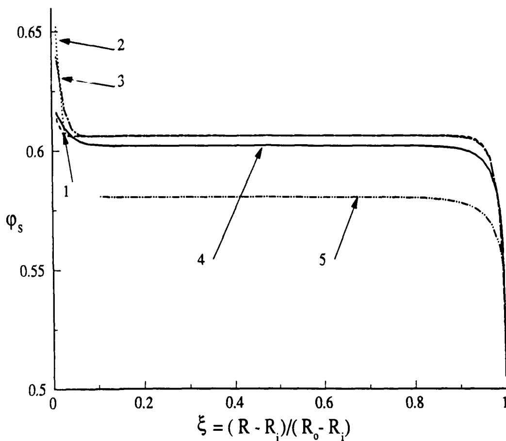
Fig.10 Radial distribution of fiber volume fraction for the following cases: 1) C_r^o = 1.478 = \text{const kPa} , 2) 1.478 \text{ kPa} \leq C_r \leq 1.476 \text{ MPa} , 3) 1.478 \text{ kPa} \leq C_r \leq 14.76 \text{ MPa} , 4) 1.478 \text{ kPa} \leq C_r \leq 147.6 \text{ MPa} , 5) 1.478 \text{ kPa} \leq C_r \leq 1.476 \text{ GPa} . The number of layers is held constant at 100.
