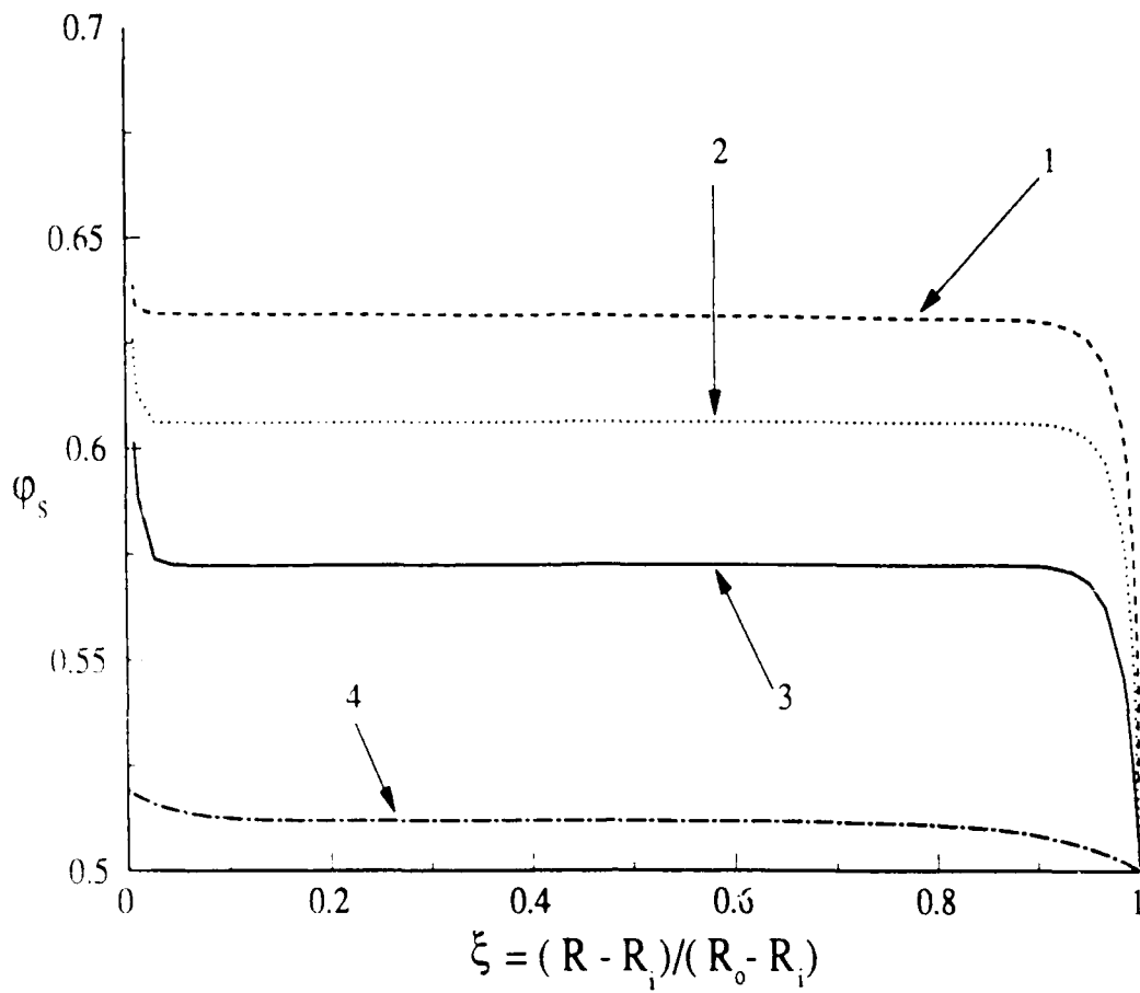
Fig.4 Radial distribution of fiber volume fraction for the following cases: 1) C_{rr}^o = 147.5 \text{ Pa} , 2) C_{rr}^o = 1.475 \text{ kPa} , 3) C_{rr}^o = 14.75 \text{ kPa} , 4) C_{rr}^o = 1.475 \text{ MPa}
