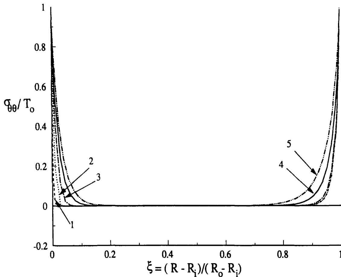
Fig.12 Radial variation of the hoop stress for the following cases: 1) C_r^o = 1.478 = \text{const kPa} , 2) 1.478 \text{ kPa} \leq C_r \leq 1.476 \text{ MPa} , 3) 1.478 \text{ kPa} \leq C_r \leq 14.76 \text{ MPa} , 4) 1.478 \text{ kPa} \leq C_r \leq 147.6 \text{ MPa} , 5) 1.478 \text{ kPa} \leq C_r \leq 1.476 \text{ GPa} . The number of layers is held constant at 100.
