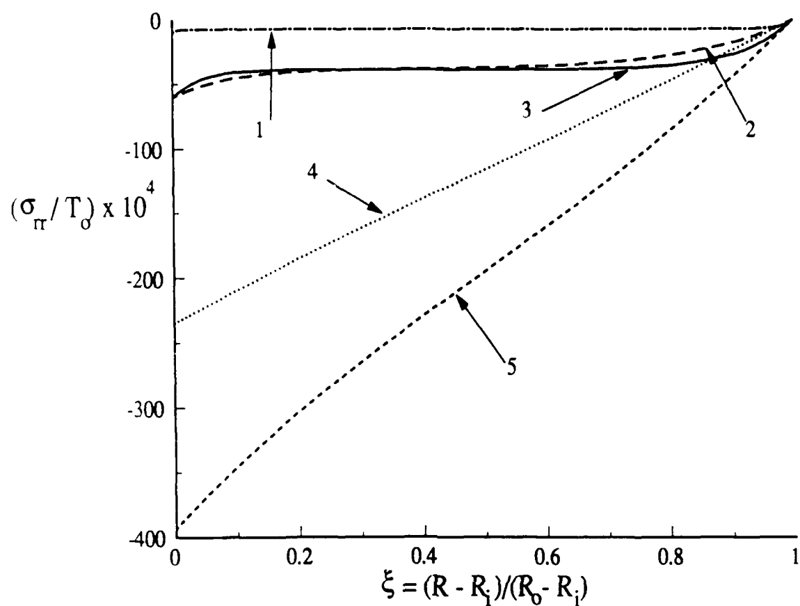
Fig.7 radial variation of the non-dimensional \sigma_r for the following cases: 1) C_r^o = 14.75 kPa and n = 100 layers, 2) C_r^o = 1.475 MPa and n = 50 layers, 3) C_r^o = 1.475 MPa and n = 100 layers, 4) C_r^o = 0.1475 GPa and n = 50 layers, 5) C_r^o = 0.1475 GPa and n = 100 layers.
