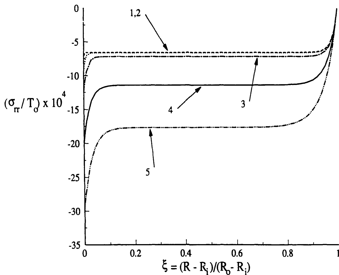
Fig.13 Radial variation of \sigma_r for the following cases: 1) C_r^0 = 1.478 = \text{const kPa} , 2) 1.478 \text{ kPa} \leq C_r \leq 1.476 \text{ MPa} , 3) 1.478 \text{ kPa} \leq C_r \leq 14.76 \text{ MPa} , 4) 1.478 \text{ kPa} \leq C_r \leq 147.6 \text{ MPa} , 5) 1.478 \text{ kPa} \leq C_r \leq 1.476 \text{ GPa} . The number of layers is held constant at 100.
