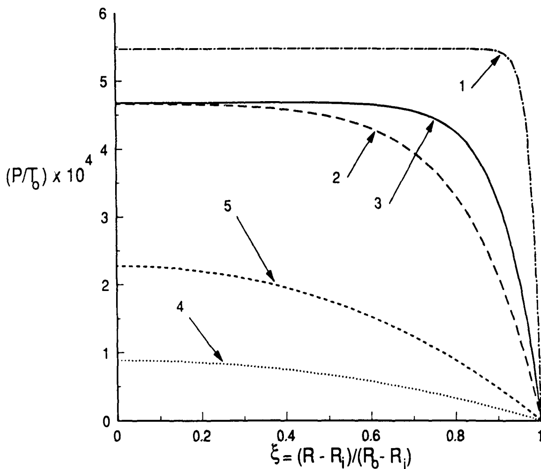
Fig.8 radial variation of the non-dimensional pressure for the following cases: 1) C_r^0 = 14.75 kPa and n = 100 layers, 2) C_r^0 = 1.475 MPa and n = 50 layers, 3) C_r^0 = 1.475 MPa and n = 100 layers, 4) C_r^0 = 0.1475 GPa and n = 50 layers, 5) C_r^0 = 0.1475 GPa and n = 100 layers.
