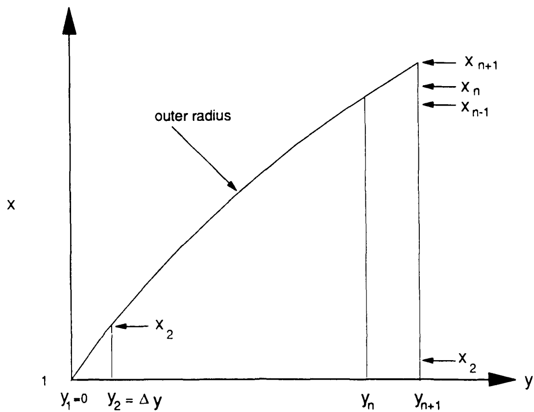
Fig.2 Schematic of the finite difference mesh.
