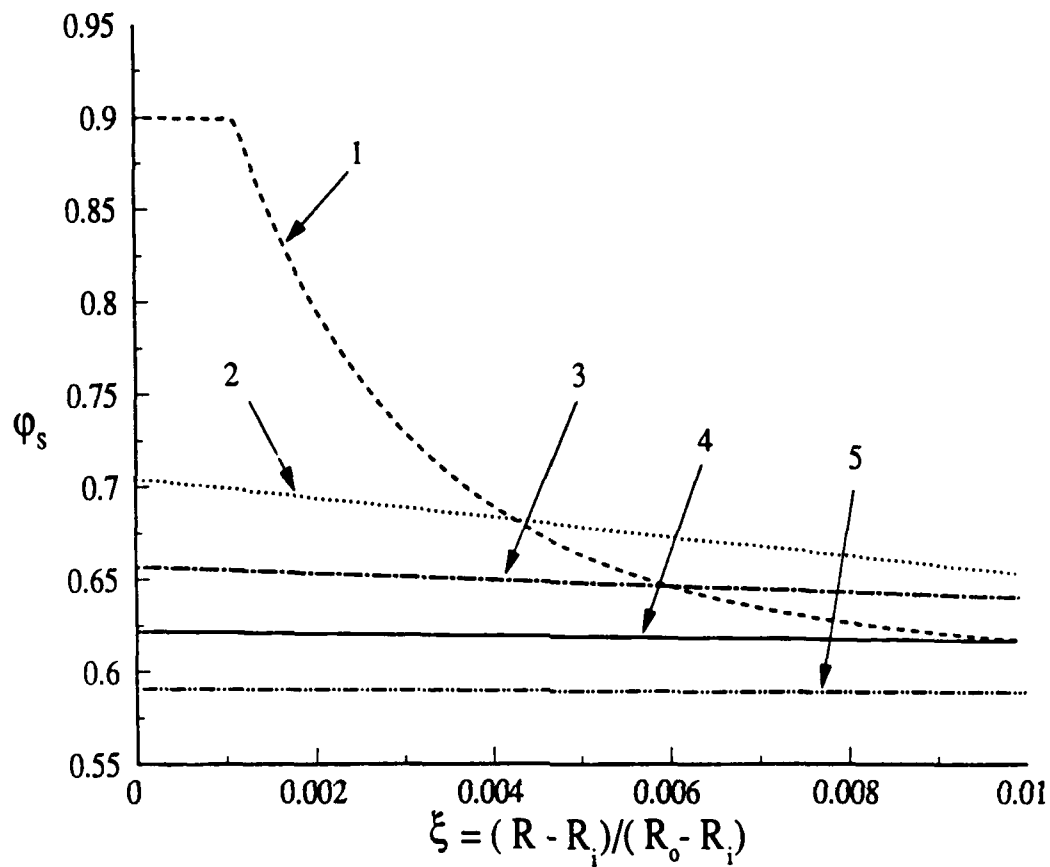
Fig.9 Profile of fiber volume fraction within the inner boundary-layer for the following cases: 1) C_{rr}^o = 1.478 = \text{const kPa} , 2) 1.478 \text{ kPa} \leq C_{rr} \leq 1.476 \text{ MPa} , 3) 1.478 \text{ kPa} \leq C_{rr} \leq 14.76 \text{ MPa} , 4) 1.478 \text{ kPa} \leq C_{rr} \leq 147.6 \text{ MPa} , 5) 1.478 \text{ kPa} \leq C_{rr} \leq 1.476 \text{ GPa} . The number of layers n is held constant at 100.
