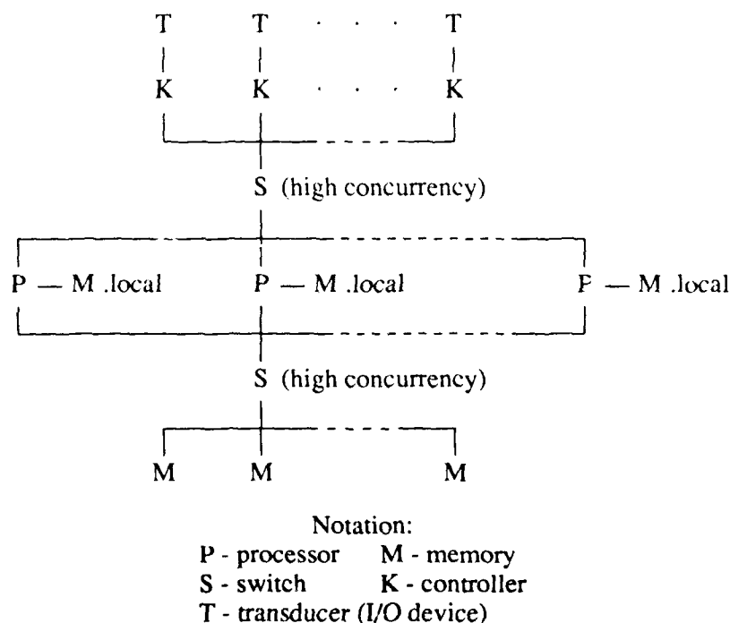
Figure 3. Shared plus private memory architecture.
