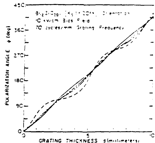
Fig. 9. Evolution of the polarization angle for diffraction in the \{K_C \parallel \langle 001 \rangle\} orientation, as shown in Fig. 7, but for a higher bias field of 10 kV/cm and a lower grating spatial frequency of 70 cycles/mm, which combine to give almost a threshold increase in the coupling strength.
