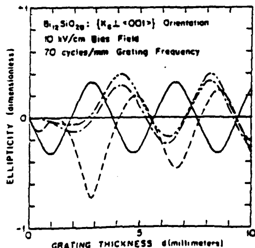
Fig. 14. Evolution of the ellipticity for recording conditions considered in Fig. 13.
