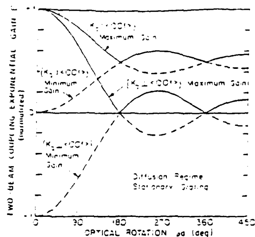
Fig. 15. Degradation of energy coupling gain \Gamma as defined in (30) with increasing levels of optical rotation \rho d , in which \rho is the optical rotatory power and d is the crystal thickness, for the two principal recording orientations. These curves are based upon analytic solutions derived by Foote and Hail for diffusion regime recording [30].
