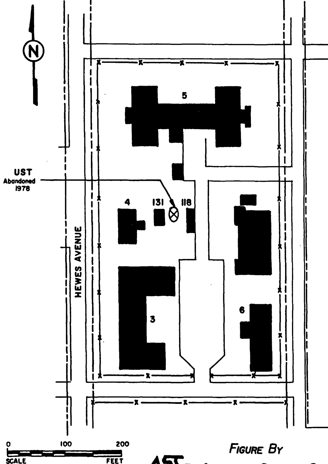
Figure 10 . Location Map of Abandoned UST East of Building 131 at the Air National Guard Field Training Site, Gulfport, Mississippi (1988).
