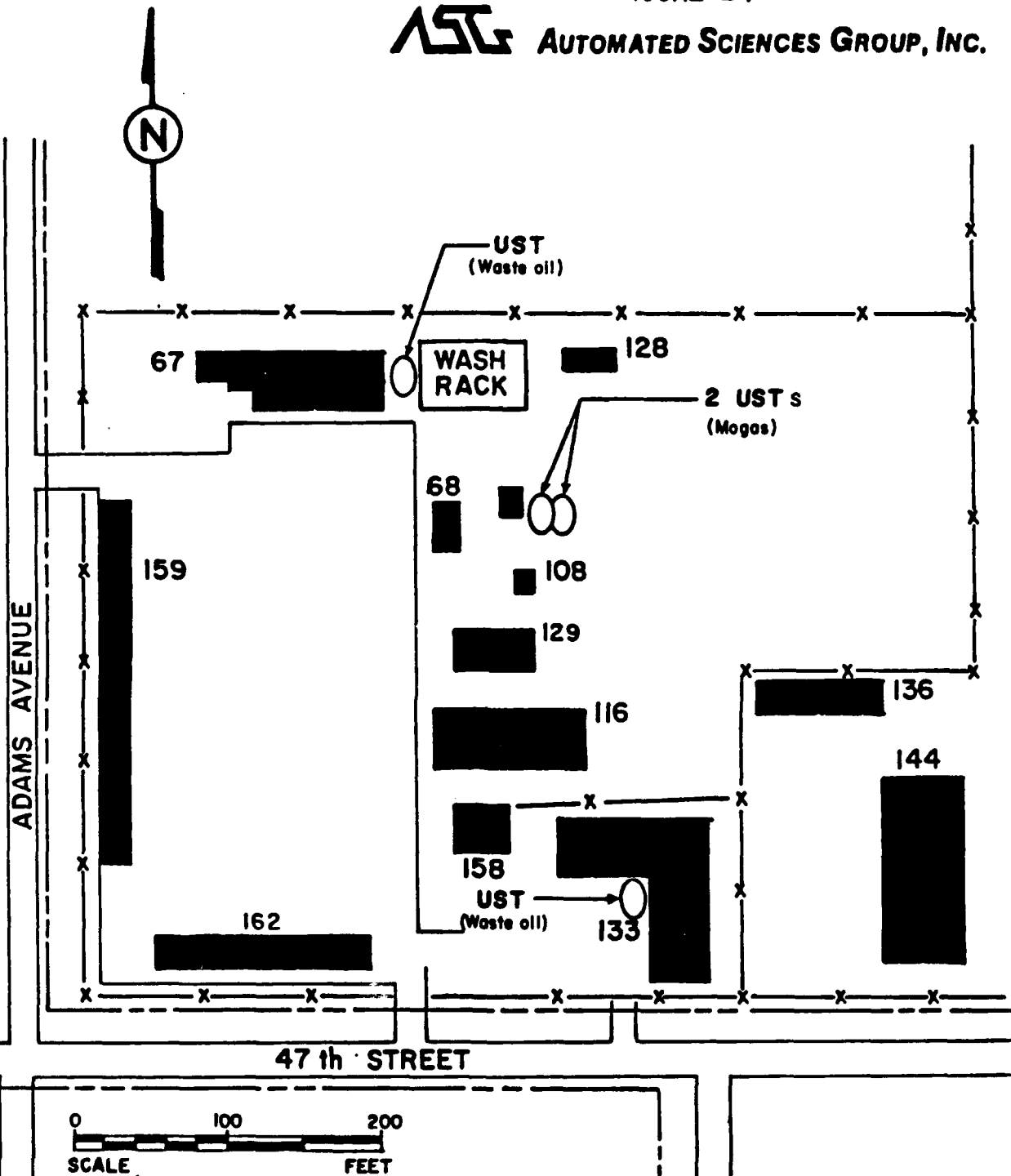
Figure 11. Location Map of USTs In Use at the Air National Guard Field Training Site, Gulfport-Biloxi Regional Airport, Gulfport, Mississippi (1988).
