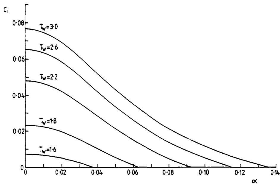
Fig 2j Variation of c_i with \alpha , M_\infty=3.8 , \zeta=0.05 , n=3 , Mode I.
