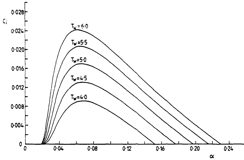
Fig 3c Variation of c_i with \alpha , M_\infty=3.8 , \zeta=0.05 , n=0 , Mode I.
