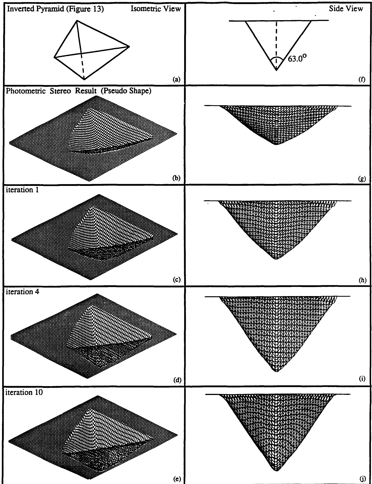
Figure 14: Shape recovery results for the inverted pyramid shown in Figure 13.
