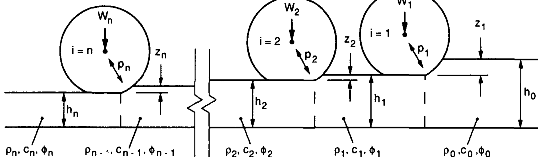
Figure A3. Depiction of progressive change in snow parameters with tire or track passage.
