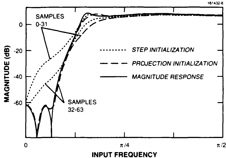
Figure 8. The average-output-magnitude frequency response of a four-pole elliptic IIR filter—projection-initialized results: the example of Figure 1 is completed with the results for projection-initialized filtering. The figure description is the same as in Figure 1, except that the zero-initialized results are not repeated and dotted lines are now used for the step-initialized results. The projection-initialized results, dashed lines, follow the steady-state stop-band performance. The response near filter resonance is more rounded, however, due to a larger transient response and cancellation at these frequencies (see Figure 6).
