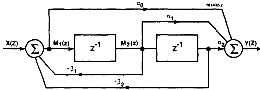
Figure 2. Conventional direct-form implementation of a second-order IIR digital filter: selecting starting values for the filter memory registers m_1(n) \{ \tilde{z} M_1(z) \} and m_2(n) \{ \tilde{z} M_2(z) \} , the object of IIR initialization.
