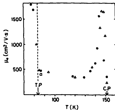
Fig. 9. Temperature dependence of electron mobility in liquid and solid argon. Earlier results ( \blacktriangle , \triangle , and \square ) are shown for comparison (Shinsaka et al., 1988).
