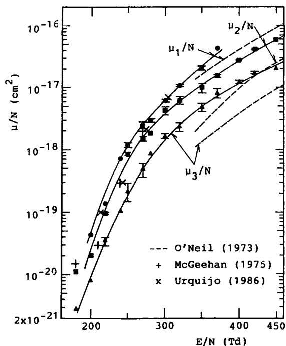
Fig. 11. Negative ion-molecule reaction coefficients in SF 6 . The present results are shown by circle ( \mu_1 ), square ( \mu_2 ) and triangle ( \mu_3 ).
