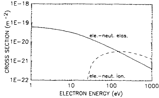
Fig. 7. Model cross sections for elastic and ionization electron-neutral collisions used in PIC simulation.
