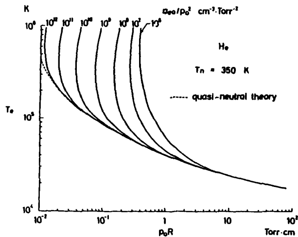
Fig. 1. Characteristics of T_e versus p_0 R for values of n_{e0}/p_0^2 at T_n = 350 K for He.
