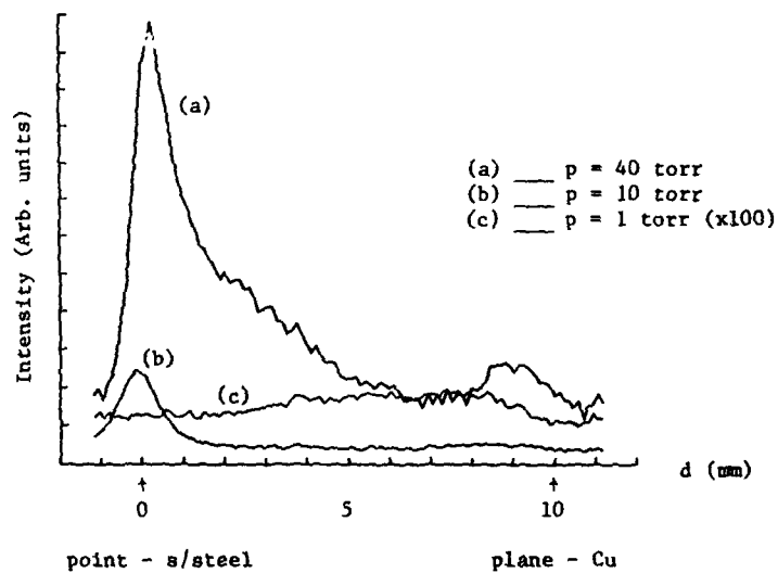
Fig. 2. Comparison of H_{\alpha} ( \lambda = 656.3 nm) intensities for point-plane geometry at various pressures. ■ 40 torr, □ 10 torr, ◇ 1 torr (x 100).
