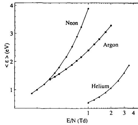
Fig. 2. Mean energy as a function of E/N.
