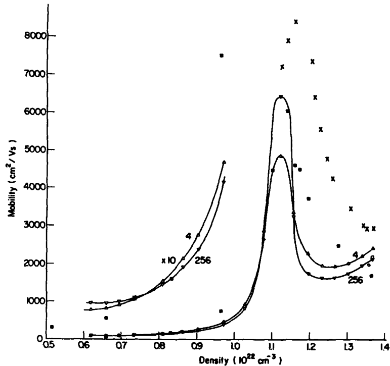
Fig. 12. Calculated drift mobility of electrons in xenon using m^* = 0.27m_0 . On average \Omega_{\min} contains either 4 ( \Delta ) or 256 ( \nabla ) atoms. Experimental TOF data: \blacksquare Huang and Freeman, 1978, \times Gushchin et al., 1982, \square Yoshino et al., 1976, \circ Miller et al., 1968.
