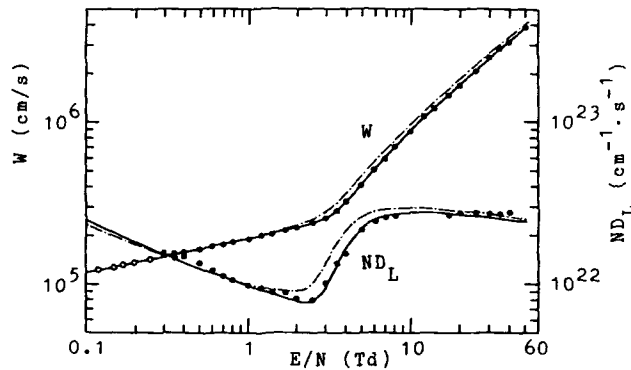
Fig. 1. The electron drift velocity W and ND_L as a function of E/N in krypton. Curves show the swarm parameters calculated with the momentum transfer cross sections shown in Fig. 2. Symbols: \bullet , present; \circ , Hunter et al., 1988.
