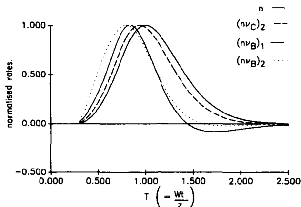
Fig. 9. Values of n , (nv_C)_2 , (nv_B)_1 , (nv_B)_2 calculated for the conditions given in Fig. 7.
