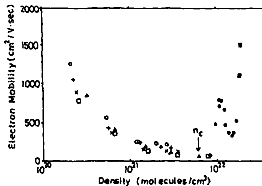
Fig. 4. Density dependence of \mu_e in methane, gas (O, x, +, and □), liquid (●), and solid (■). n_c means the critical density (Nakamura et al., 1983).
