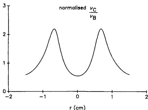
Fig. 5. The observed radial variation of \nu_C/\nu_B+ (normalized) for a steady-state Townsend discharge (see text for the discharge conditions). The large departures from unity indicate a strong radial dependence of the mean energy for the small \lambda_L z value ( \sim 1.0 ) in this example.
