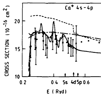
Fig. 3. Figure 1 of Mitroy et al. (1988). Absolute emission cross-section for electron impact excitation of the \text{Ca}^+ 4p_{3/2} state as a function of incident energy. The following calculations are depicted: CCV6 —, CCV3 - - - -, UCBAV6 — · — ·, and CCV6 convoluted with an energy resolution function of full width 0.023 Ryd ·····. The experimental data of (Taylor and Dunn, 1973; Zapesochnyi et al., 1976) are depicted as x and o, respectively.
