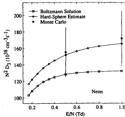
Fig. 7. Same as in Fig. 6, but for neon.
