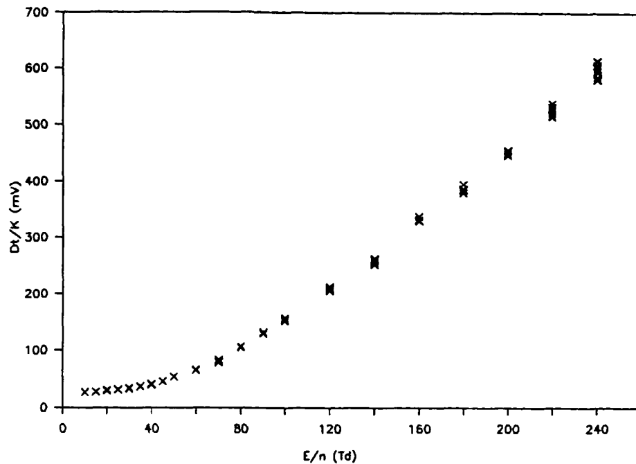
Fig. 1. Ratios of Dt/K for \text{Na}^+ ions in argon.
