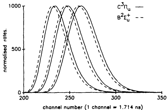
Fig. 2. The time dependent excitation rate n\nu_C and n\nu_B^+ determined from the theoretical results shown in Fig. 1.
