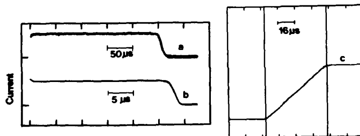
Fig. 8. Negative ion transients in SF_6 . (a), (b), from the differentiated pulse condition (de Urquijo-Carmona, 1983), and (c) from the integrated pulse condition (Cornell and Littlewood, 1986). (a) 45.5 Td, 25.7 kPa; (b) 242 Td, 9.3 kPa, (c) 135 Td, 26.7 kPa.
