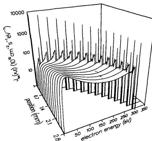
Fig. 3. Energy distribution of fast electron flux as a function of position at 300 V and 0.6 torr from the multibeam model solution.
