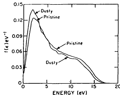
Fig. 9. Electron energy distributions in pristine and dusty argon plasmas ( E/N = 7 Td, \rho = 10^5 \text{ cm}^{-3} ).
