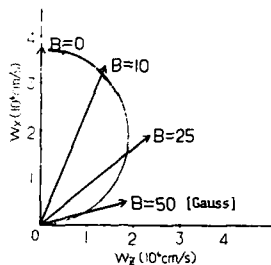
Fig. 1. Rotation of drift velocity vector by increasing B.
