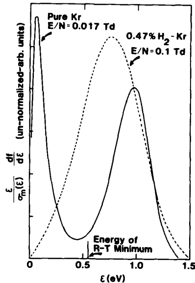
Fig. 5. The integrand in the formula for v_{dr} (Eq. 4) plotted as a function of energy in pure Kr for E/N = 0.017 Td, and in an 0.47 H_2 - Kr mixture for E/N = 0.1 Td. In each case the value of E/N was chosen so that the most probable energy was close to the energy of the R-T minimum.
