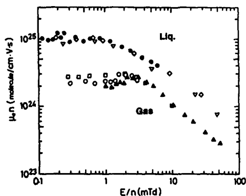
Fig. 10. Electric field dependence of density-normalized electron mobility in liquid ( \bullet ) and gaseous ( \circ and \blacktriangle ) argon. Earlier results ( \diamond , \nabla , and \square ) are shown for comparison (Shinsaka et al., 1988).
