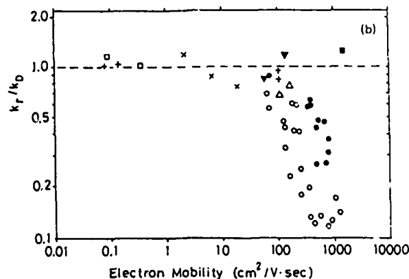
Fig. 8. Plots of k_r/k_D vs \mu_e in several fluids and solids; \blacksquare , solid methane; \bullet , liquid methane; \circ , gaseous methane; \times , liquid mixtures of neopentane and n-hexane; \nabla , liquid and solid neopentane; \Delta , liquid and solid tetramethylsilane; + , liquid n-pentane, n-hexane, and tetramethylsilane; \square , liquid n-hexane and cyclohexane (Tezuka et al., 1983; Nakamura et al., 1983; Shinsaka et al., 1988).
