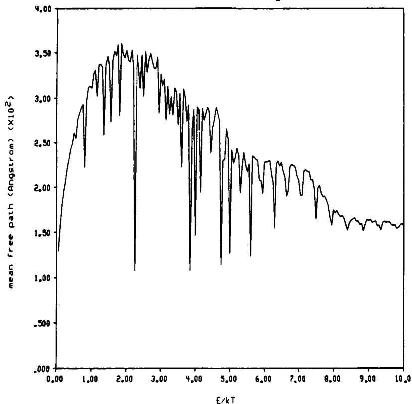
Fig. 7. Same as Fig. 5 for T=150 K, n=1.04 \times 10^{22} \text{ cm}^{-3} , m^*=0.49m_0 .
