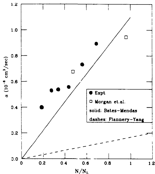
Fig. 7. Recombination coefficients for the reaction, \text{Xe}^+ + \text{F}^- + \text{He} \rightarrow \text{XeF}^* + \text{He} , in helium.
