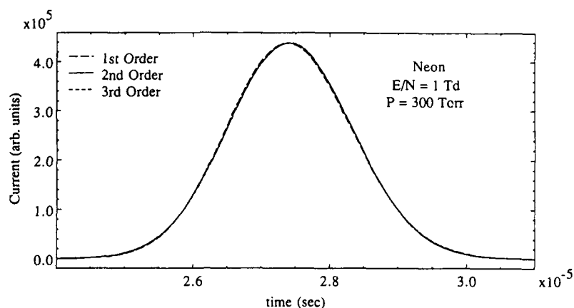
Fig. 13. Same as Fig. 12, but for P = 300 Torr.
