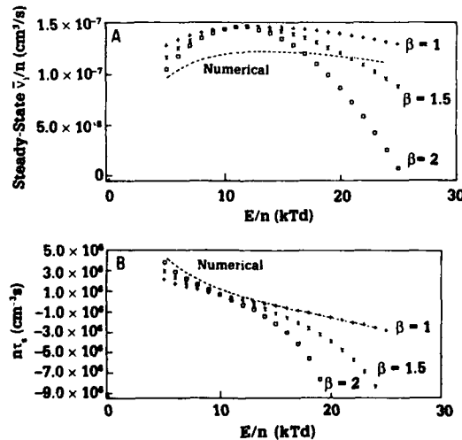
Fig. 8. Comparison between the analytic models of different \beta and the numerical results. A. Steady-state average ionization rate coefficient \bar{v}_1/n . B. Density-normalized induction time n\tau_s as functions of E/n .
