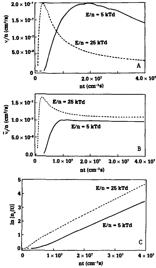
Fig. 7. Numerical results vs. nt for different E/n . A. Ionization rate coefficient of the primary electron v_1/n . B. Average ionization rate coefficient \bar{v}_1/n . C. Natural logarithm of the total number of electron \ln[n_e(t)] and negative induction time obtained for E/n = 25 kTd.
