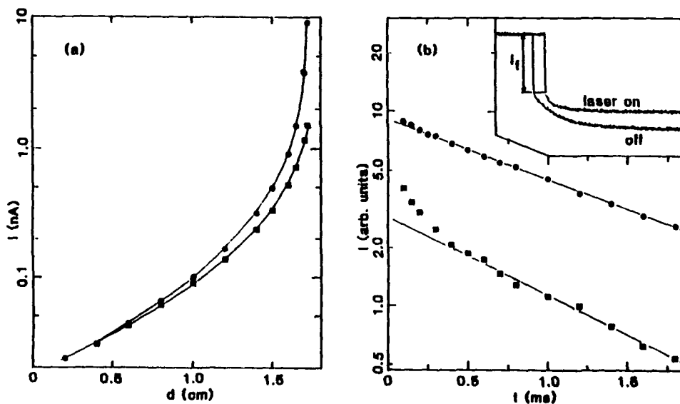
Fig. 1. The effect of laser irradiation on the (a) spatial and (b) temporal ionization growth in Ne [ E/N = 141 \text{ Td} and N = 7.1 \times 10^{16} \text{ cm}^{-3} ]. ● - without laser; ■ - with laser intensity of 33.5 \text{ W m}^{-2} . In (b), d = 1.4 \text{ cm} and the inset shows the signal-averaged data from which the \log I(t) plot was obtained.
