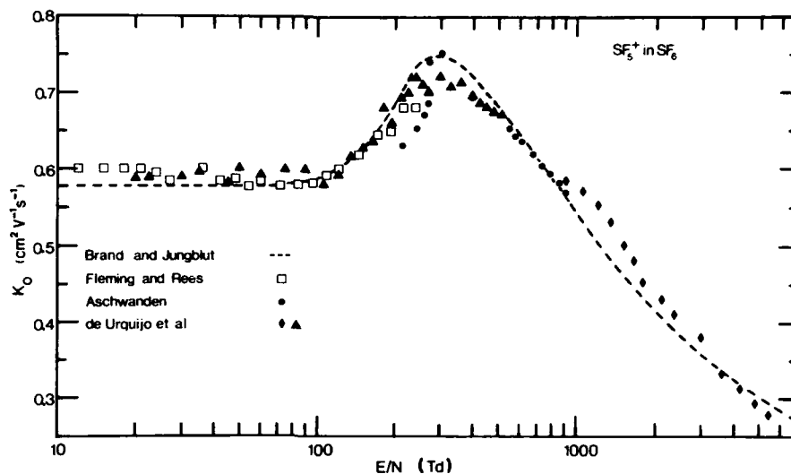
Fig. 12. Reduced mobilities of SF_5^+ in SF_6 as a function of E/N . Diamonds, mass-analyzed data of de Urquijo-Carmona et al. (1990). Triangles, data from de Urquijo-Carmona et al. (1985b).
