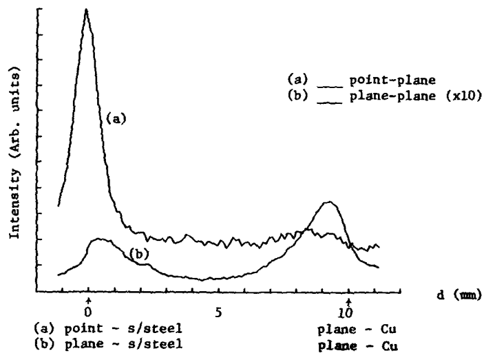
Fig. 1. Comparison of H_{\alpha} ( \lambda = 656.2 nm) intensities of point-plane and plane-plane geometries of P = 10 torr. (a) — point-plane, (b) — plane-plane (x10).
