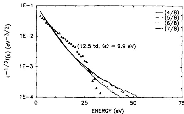
Fig. 10. Electron energy distribution function, averaged from the central 8 mm of the discharge as a function of time in the rf period. Also shown is eefd from a local field simulation at the same mean electron energy as the PIC results.
