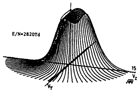
Fig. 3. Velocity distribution g^0(v) .
