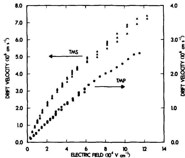
Fig. 7. w versus E for TMS ( \blacktriangle ) and TMP ( \bullet ), Faidas et al. (1989a). The w(E) values of Faidas et al. (1989a) for TMS are \sim 20 percent higher than those of Döldissen and Schmidt (1979). See discussion in Faidas et al. (1989a).
