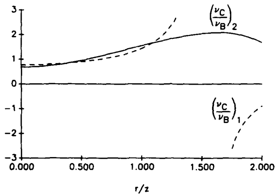
Fig. 11. Calculated values of \nu_C/\nu_B+ for first order and second order terms in the gradient expansion. Only the expansion including second-order terms gives the off-axis maximum in the excitation ratio, as observed experimentally.
