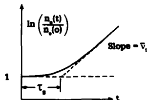
Fig. 6. A schematic of the experimental results from which the ionization rate \bar{v}_i and the induction time \tau_s are determined.
