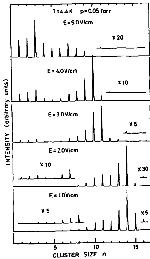
Fig. 1. Mass spectra of \text{He}_n^+ .
