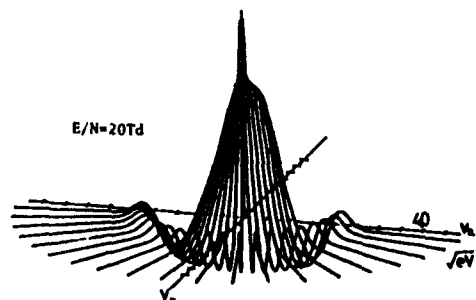
Fig. 6. Velocity distribution g_{LL}(v) .
