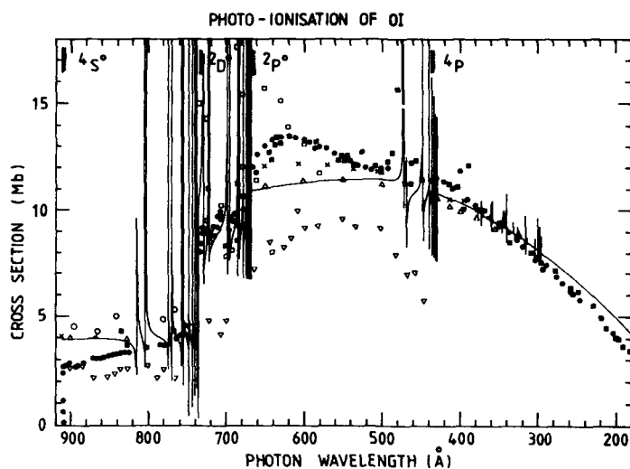
Fig. 7. Figure 1 of Bell et al. (submitted). Photoionization cross-section of the ^3P state of atomic oxygen. Theory: — from Bell et al. (submitted), \Delta Pradhan (1978), \times Taylor and Burke (1976). Experiment: \nabla Comes et al. (1968), \circ Kohl et al. (1978), \square Hussein et al. (1985), \blacksquare Samson and Pareek (1985), \bullet Angel and Samson (1988). Thresholds correspond to experimental values.
