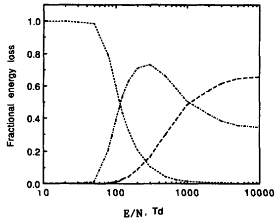
Fig. 6. Calculated fractional electron energy loss to vibrational excitation (-----), dissociation (- · -) and ionization (- - -) versus E/N in CH 4 .
