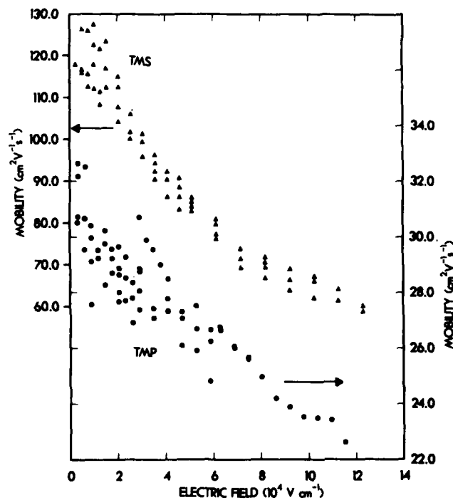
Fig. 8. Mobility of excess electrons versus applied electric field in TMS ( \blacktriangle ) and TMP ( \bullet ), Faidas et al. (1989a).
