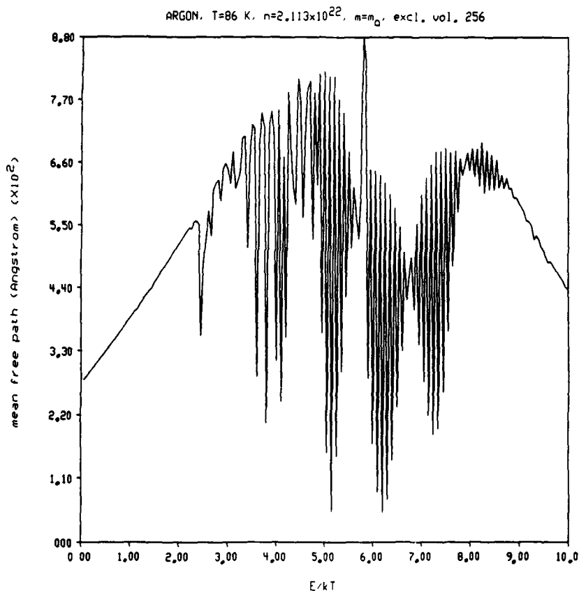
Fig. 5. Static density fluctuation limited mean free path for electrons with m^* = m_0 in argon at 86K and density n=2.11 \times 10^{22} \text{ cm}^{-3} . On average, \Omega_{\text{min}} contains 256 atoms.
