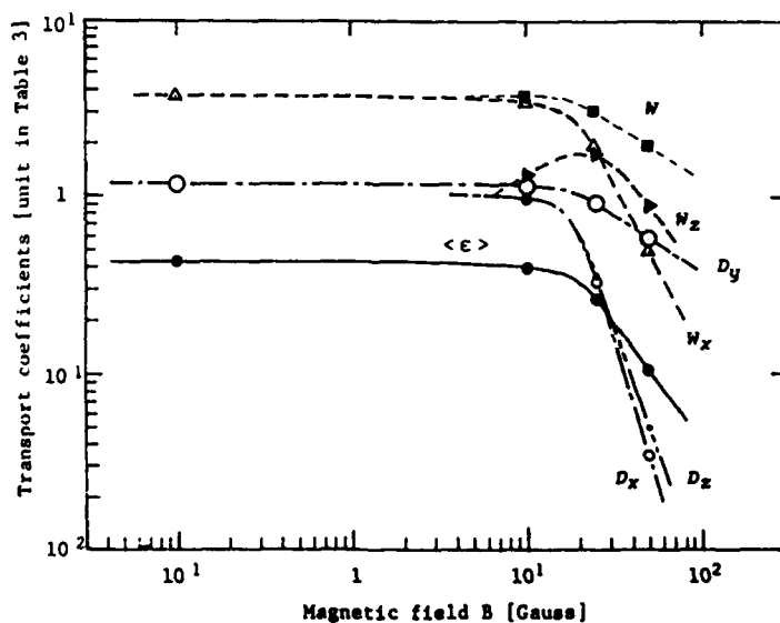
Fig. 2. Variation of transport coefficients for the value B.
