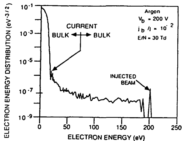
Fig. 1. Electron energy distribution for "Beam-in-a-Box" experiment.
