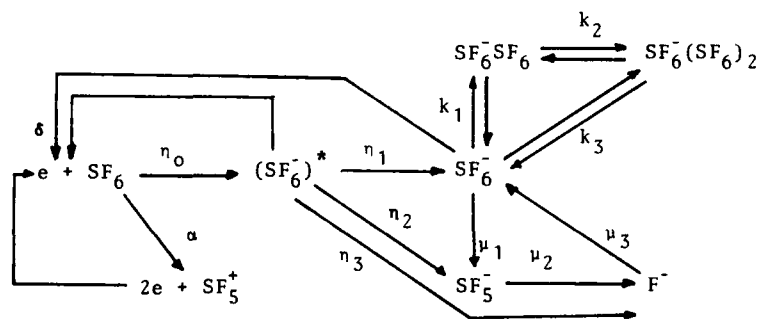
Fig. 1. Simplified reaction scheme for SF_6 . \alpha , \eta , \delta , \mu , ionization, attachment, detachment and charge transfer coefficients; k_1 , k_2 , k_3 , reaction rates.
