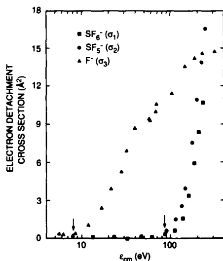
Fig. 1. Collisional electron-detachment cross sections for F^- , SF_5^- , and SF_6^- on SF_6 target gas as a function of center-of-mass energy.
