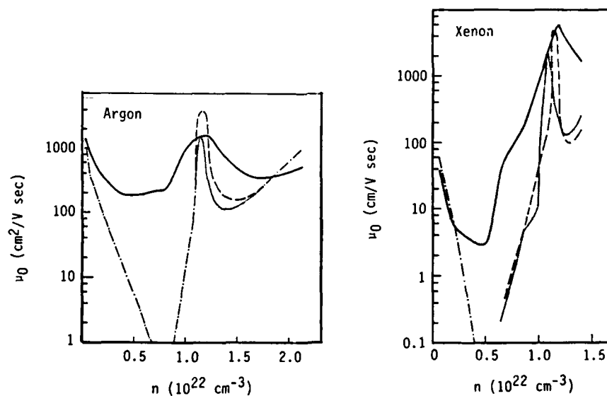
Fig. 3. Zero field mobilities in argon and xenon from Reininger et al., 1983, ..... simplified calculation according to Basak and Cohen, 1979, --- full calculation, -.-.- simplified and full calculation coincide. — experimental TOF data used in Reininger et al., 1983.
