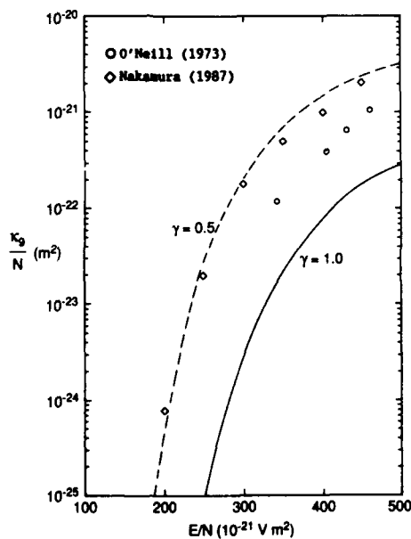
Fig. 6. Calculated reaction coefficients for the reaction \text{F}^- + \text{SF}_6^- \rightarrow \text{F} + \text{SF}_6 using measured cross-section data \sigma_6(\epsilon_L) and a Kagan and Perel ion kinetic-energy distribution. The symbols are previously calculated reaction coefficients for the same process derived from uniform-field drift-tube data.
