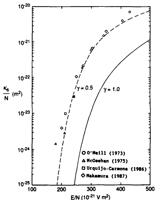
Fig. 4. Calculated reaction coefficients for the reaction SF_6^- + SF_6 \rightarrow SF_5^- + F + SF_6 using measured cross-section data \sigma_6(\epsilon_L) and a Kagan and Perel energy distribution. The symbols are previously calculated reaction coefficients for the same process derived from uniform-field drift-tube data.
