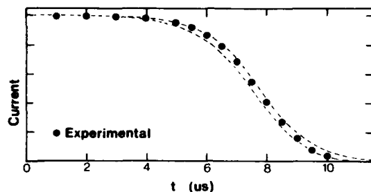
Fig. 5. Positive ion transient in SF_6 at E/N = 1820 Td, p = 40 Pa, from de Urquijo-Carmona et al., 1985b. The broken curves enclose the region of maximum combined uncertainties of the fitting process.
