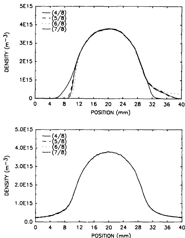
Fig. 8. Solution to PIC model of rf discharge at 0.1 torr, 30 MHz and 800 V_{rf} applied voltage: (a) ion density profiles at four times in the rf period; (b) corresponding electron density profiles, showing sheath modulation.
