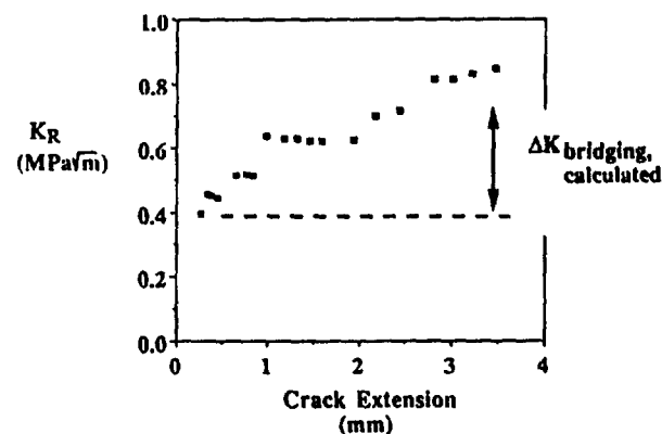
Figure 3. R-curve measured from a copper film laminate C(T) specimen diffusion bonded at 550° C.
