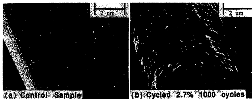
Figure 6. SEM of a control sample and a sample cycled at 2.7% for 1000 cycles at 20,000 X.
