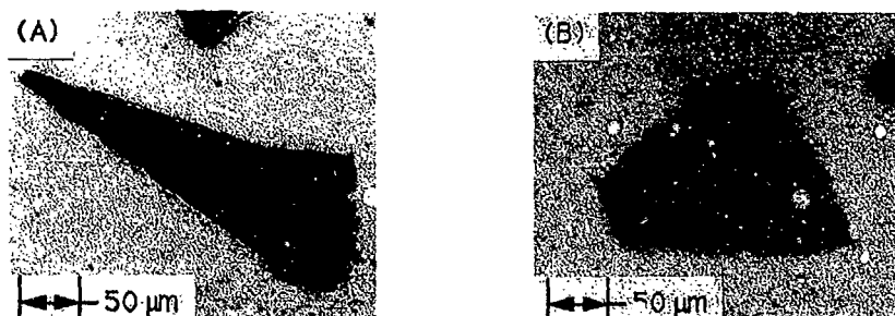
Fig. 3 \text{Al}_2\text{O}_3 particle in Ti-52.1 at% Al-2.0 at% Ta matrix: A) as received, b) heat-treated at 1100^\circ\text{C} for 192 hours.
