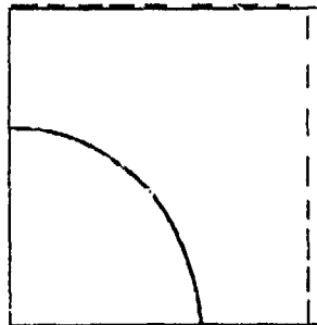
Figure 5 - RVE displacements for well-bonded interface under normal tensile loads transverse to fiber (dashed lines define unloaded shape).
