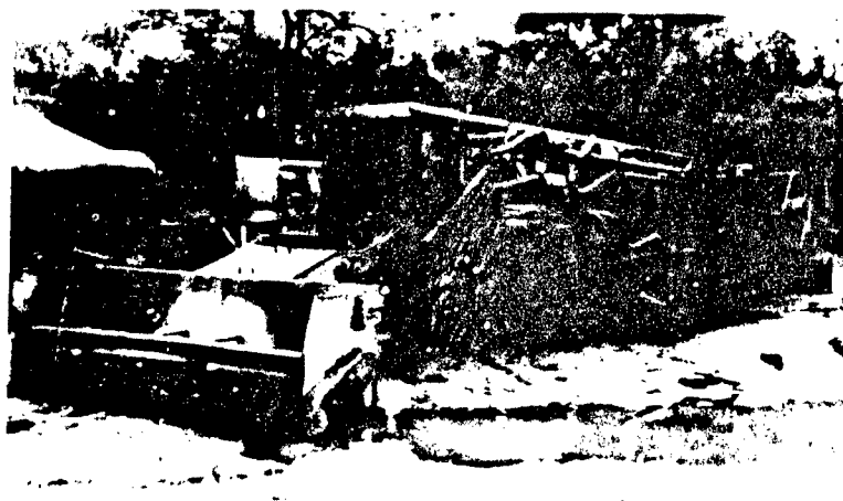
Photo 10. Third machine in recycling train with front trough for new mix, heating section, and milling head at the rear
