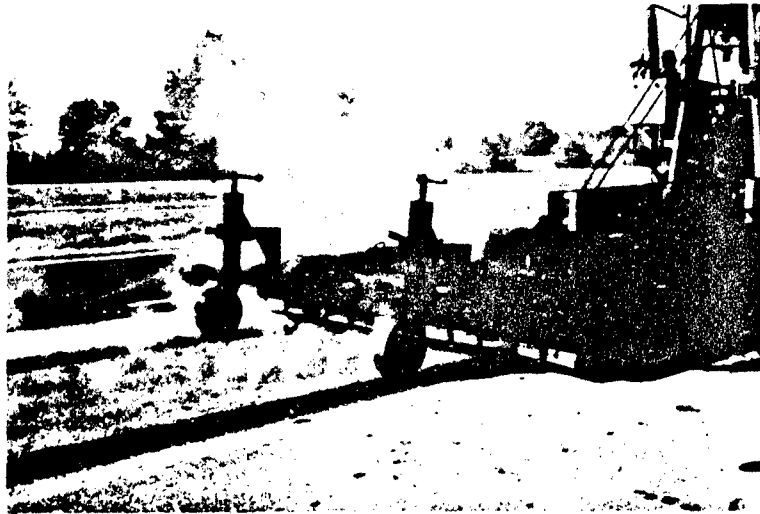
Photo 5. Heated pavement behind second preheater
