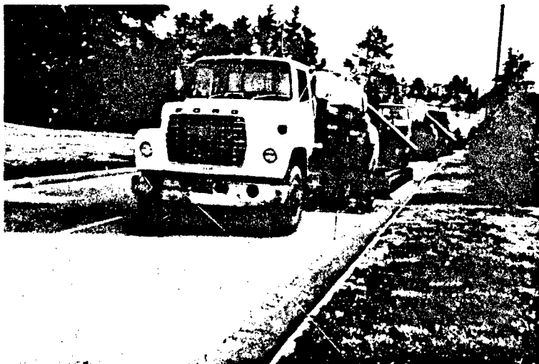
Photo 19. Remotely controlled heater/ scarifying vehicles
