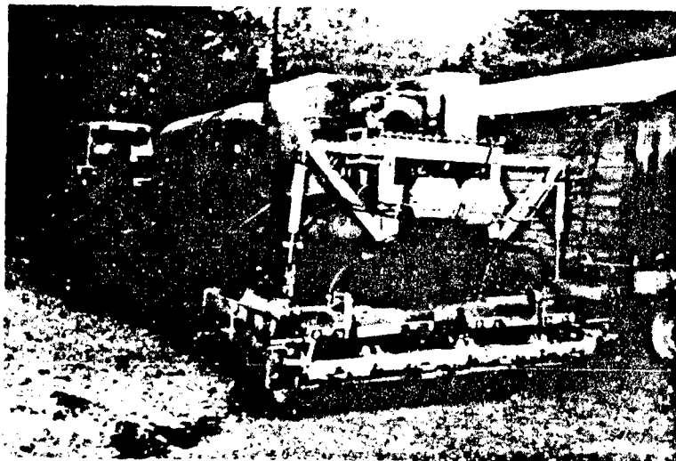
Photo 9. Tractor-towed preheating unit
