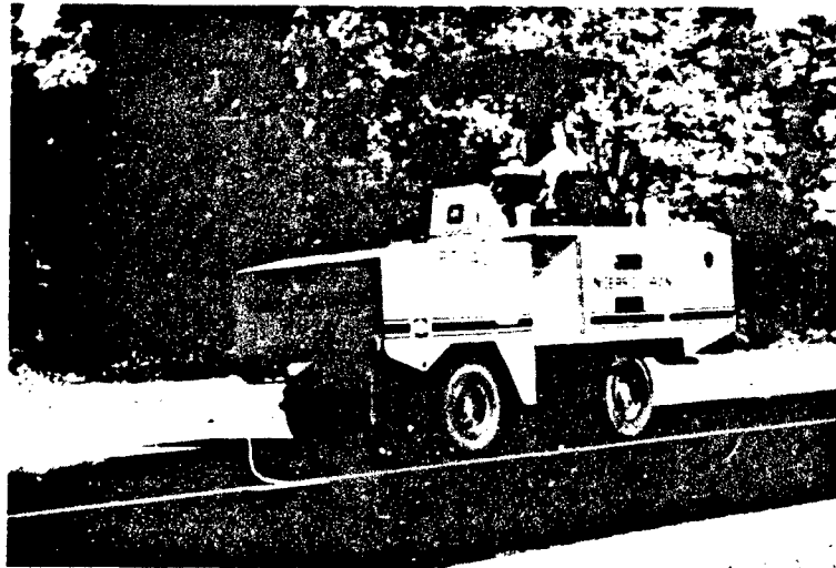
Photo 7. Rubber-tired (pneumatic) roller compacting recycled pavement
