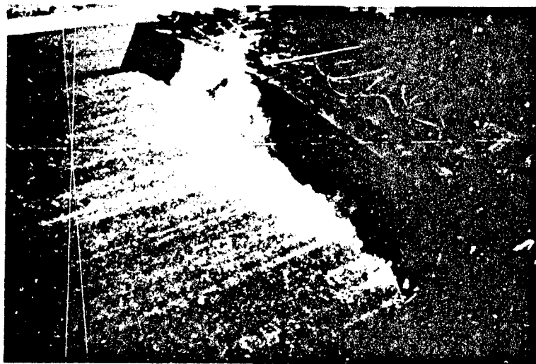
Photo 23. Spray bar applying rejuvenator
