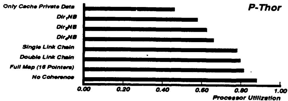
Figure 5-1: Comparison of coherence schemes.
