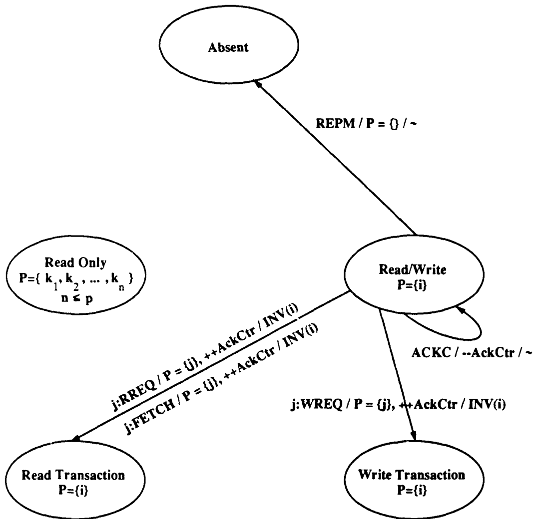
Figure B-11: Memory state transitions for limited directory: Read/Write state.
