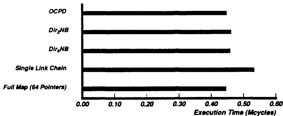
Figure 4-7: Comparison of coherence schemes using coupled simulations.
