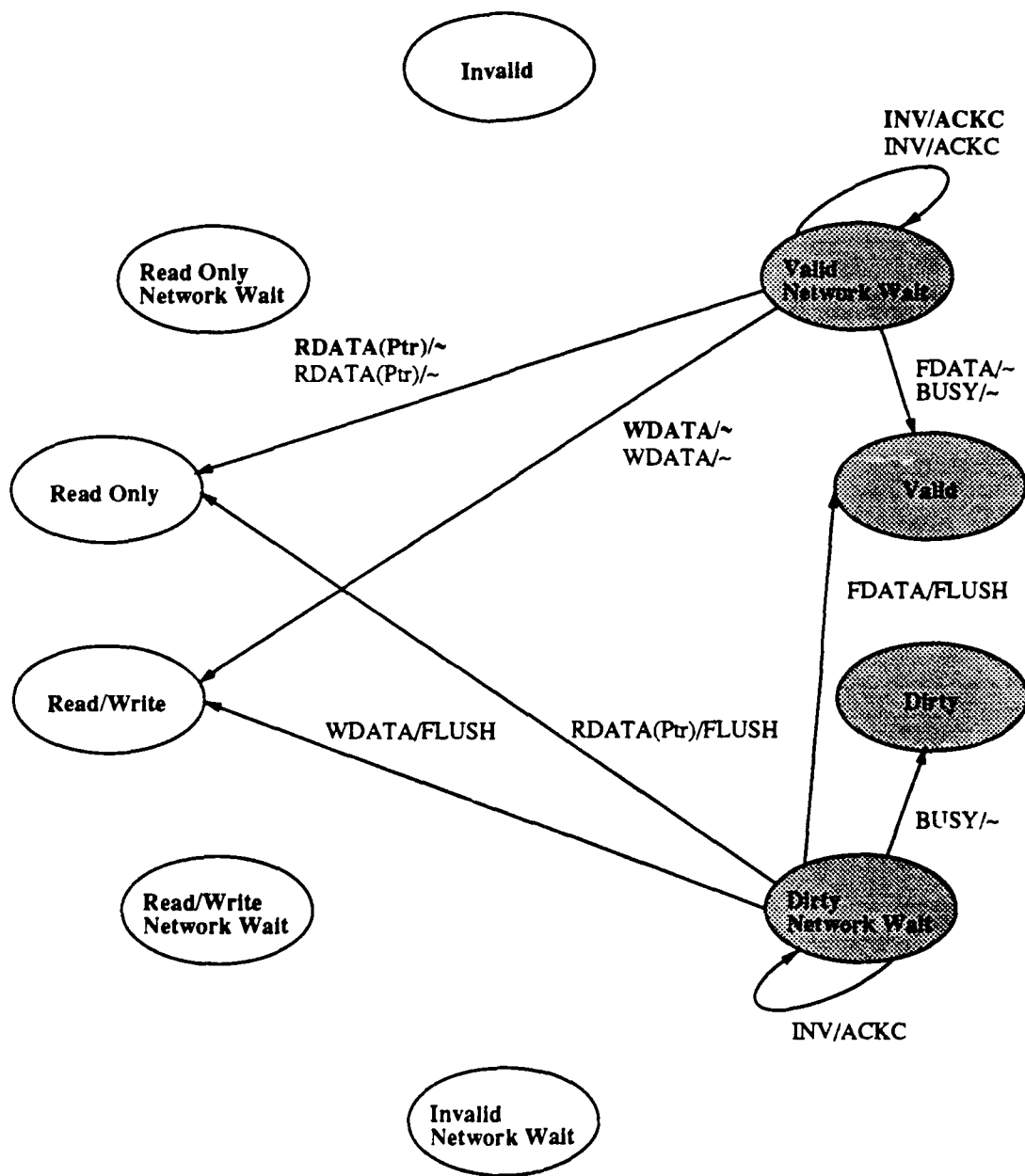
Figure B-5: Cache state transitions for messages: Software coherence Network Wait states.
