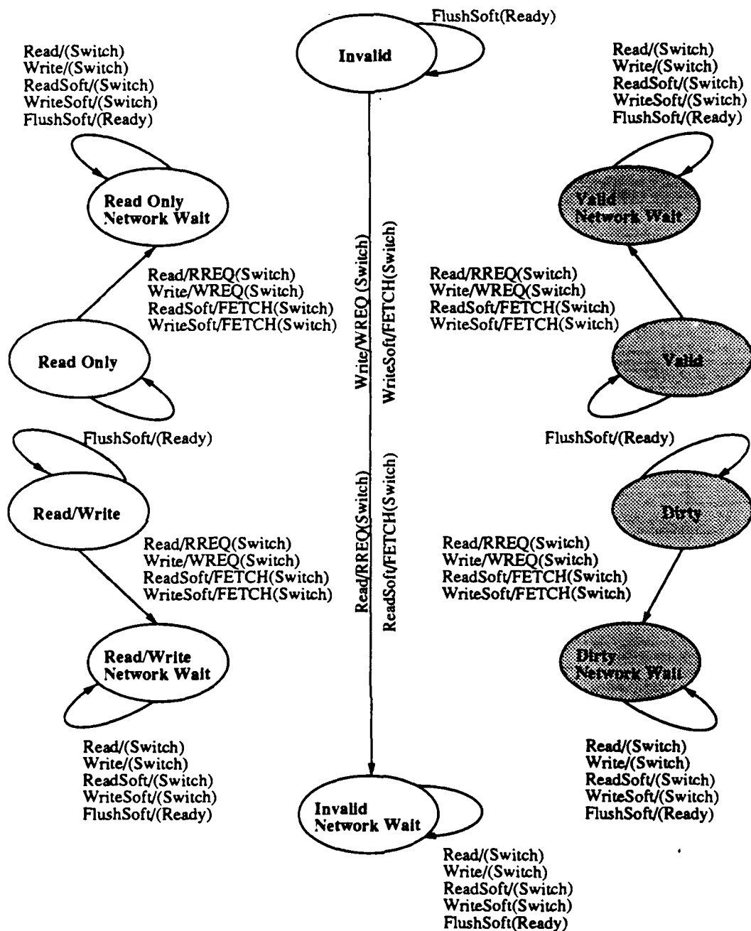
Figure B-3: Cache state transitions for processor requests when the tag does not match.
