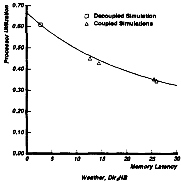
Figure 4-4: Processor utilization versus memory latency. The curve indicates the prediction of the network model. The individual points are data from simulations.
