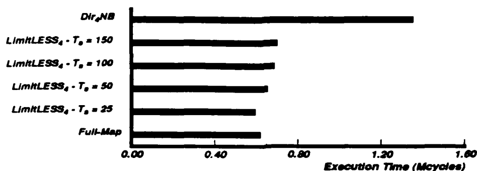
Figure 5-4: Weather, 64 Processors, LimitLESS with 25 to 150 cycle directory emulation latencies.
