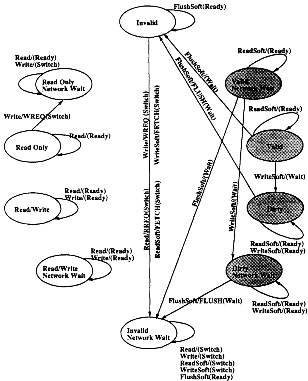
Figure B-1: Cache state transitions for processor requests when the tag matches.
