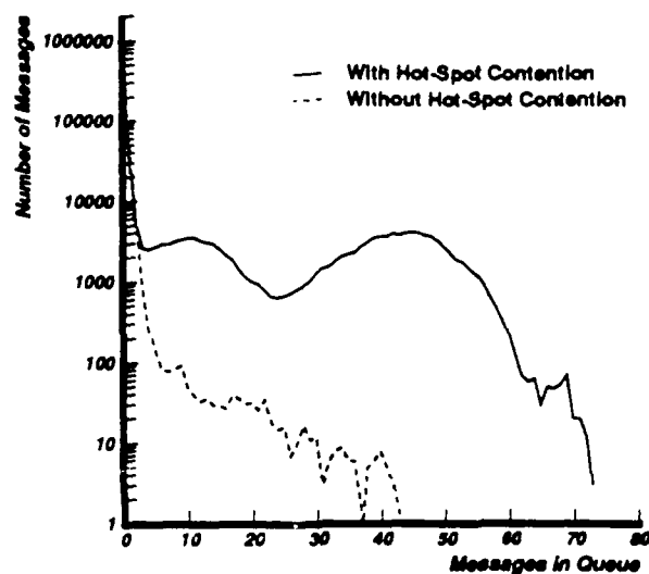
Figure 4-6: Cache controller queue sizes with Dir_4NB protocol.
