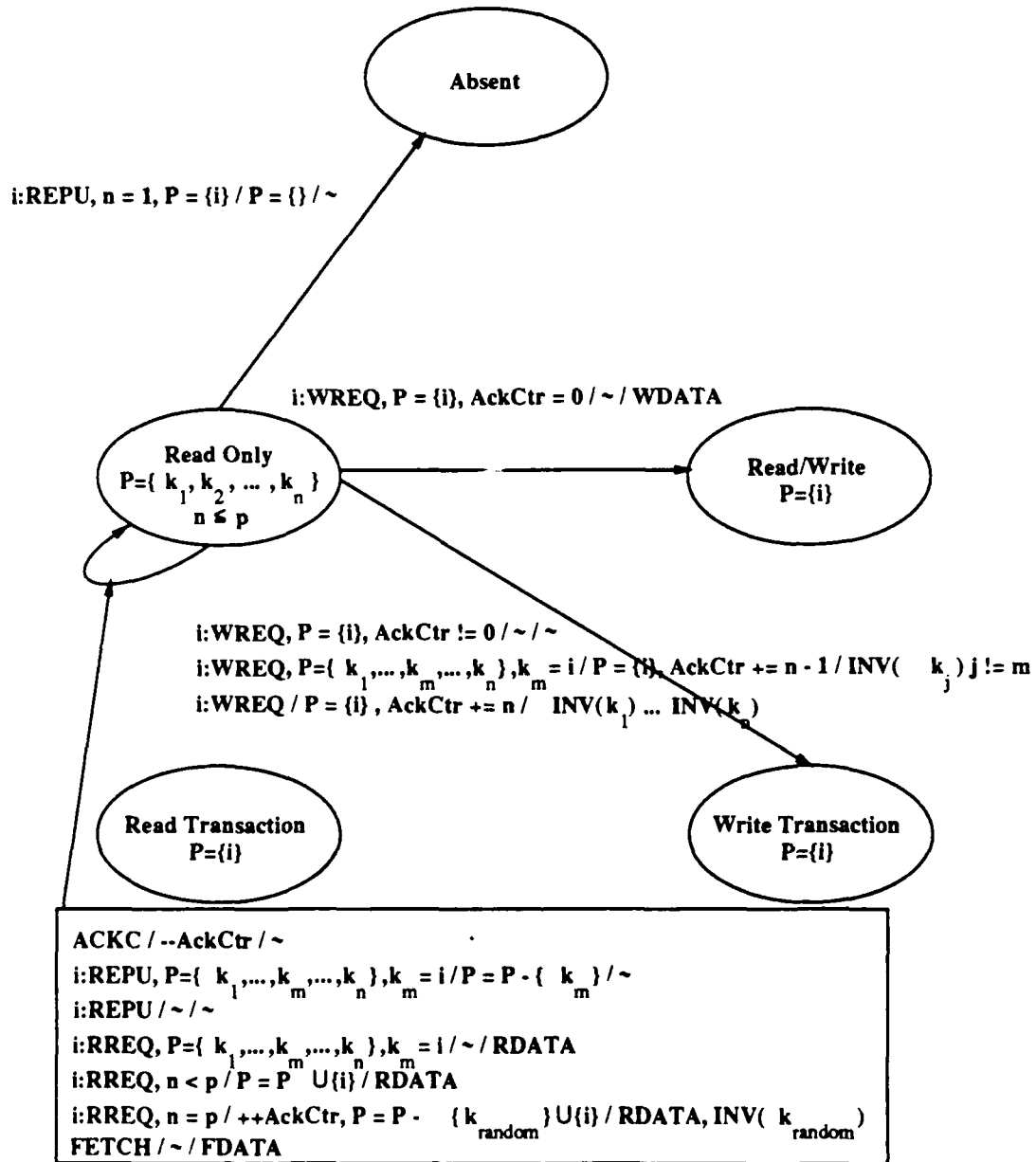
Figure B-10: Memory state transitions for limited directory: Read Only state.
