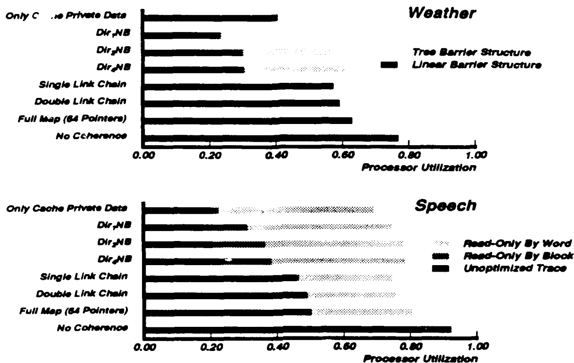
Figure 5-2: System-level optimizations.
