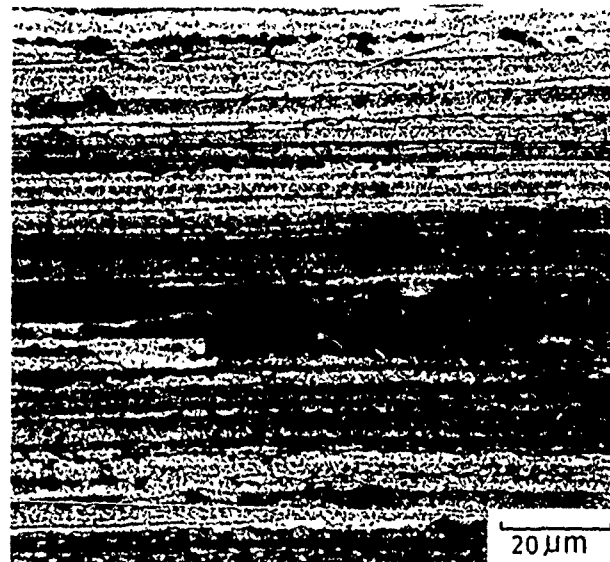
FIGURE 8—The microstructure of the Al-3.7wt%Zn-2.5wt%Mg alloy.
