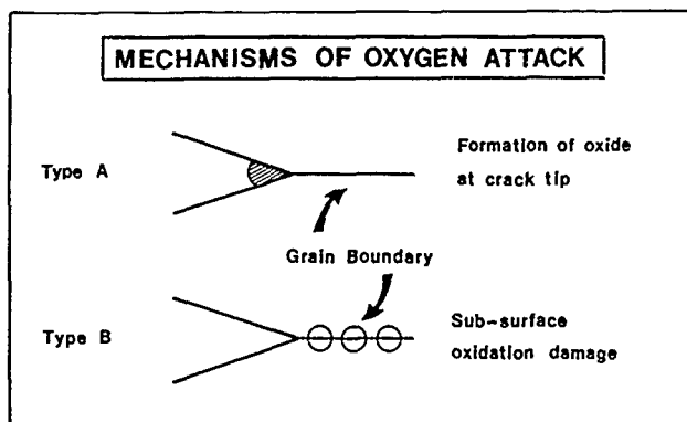
FIGURE 8—Mechanisms of oxygen attack.
