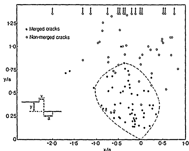
FIGURE 26—Dimensional conditions for the coalescence of adjacent stress corrosion cracks at the surfaces of ferritic steel specimens exposed to a \text{CO}_3\text{-HCO}_3 solution. 61
