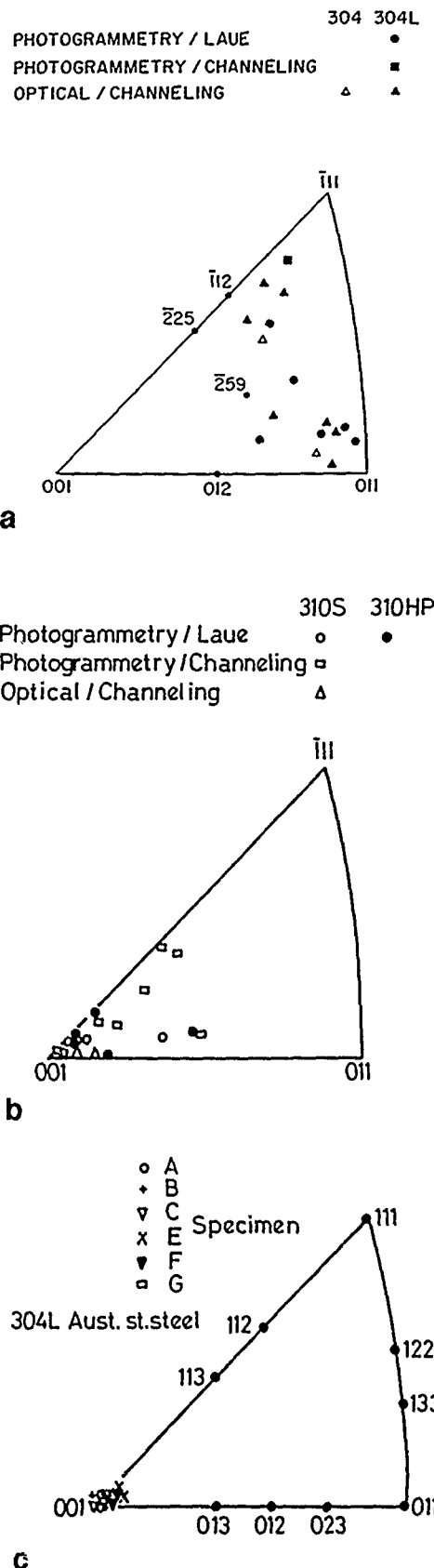
FIGURE 24—Stereographic triangles showing the poles of stress corrosion facets for austenitic stainless steels cracked in hot chloride solutions: (a) and (b) from Liu, et al., showing {100} orientation for type 310 (UNS S31000) SS but varying orientation for types 304 and 304L (UNS S30400 and S30403). (Reprinted with permission. 93 ); (c) from Meletis and Hochman showing {100} orientation for type 304L (UNS S30403) monocrystals. (Reprinted with permission from Pergamon Press. 95 )
