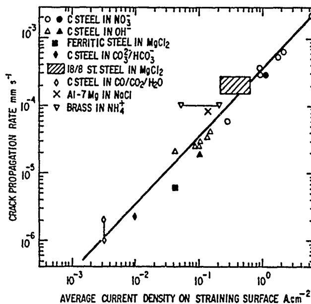
FIGURE 5—Relationship between the average crack propagation rate and the oxidation (i.e., dissolution and oxide growth) kinetics on a straining surface for several ductile alloy/aqueous environment systems. 7,29
