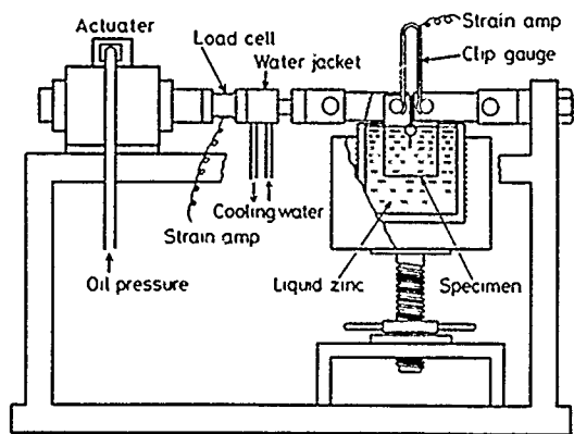
FIGURE 1—Experimental apparatus.
