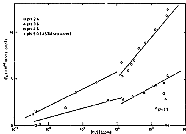
FIGURE 4—Variation of subsurface hydrogen concentration ( C_0 ) with \text{H}_2\text{S} concentration and pH.
