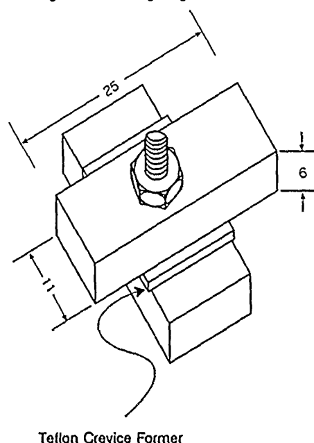
FIGURE 1 —Schematic diagram of an unstressed crevice coupon.
