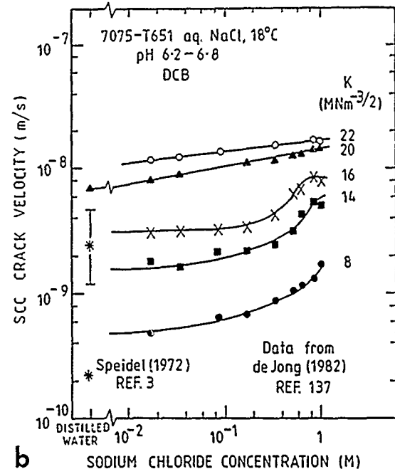
FIGURE 20—Stress corrosion crack velocities for 7XXX series alloys in aqueous solutions containing chloride and iodide ions; (a) Region 2 SCC plateau velocities for various alloys and (b) SCC crack growth rates as a function of sodium chloride concentration for a range of stress-intensity factors.
