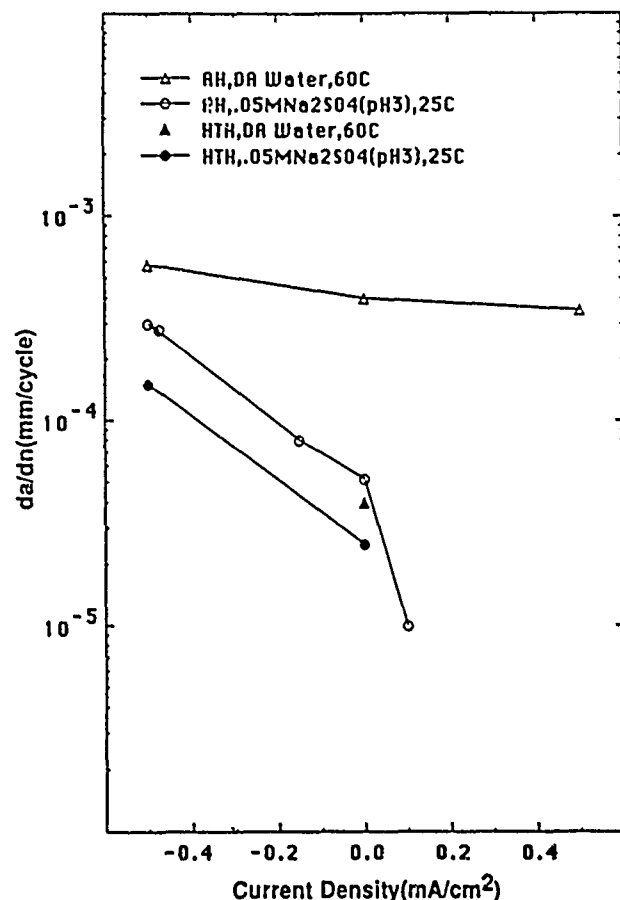
FIGURE 10—Fatigue crack growth rate of the AH and HTH heat treatments as a function of charging current density and environment. Tests conducted at a \Delta K of 25 \text{ MPa}\sqrt{\text{m}} , a frequency of 1.0 Hz, and an R ratio of 0.1.
