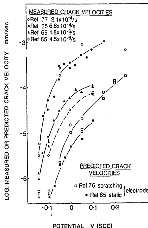
FIGURE 21—Measured and predicted crack velocities from various sources for brasses exposed to \text{NaNO}_2 solution.
