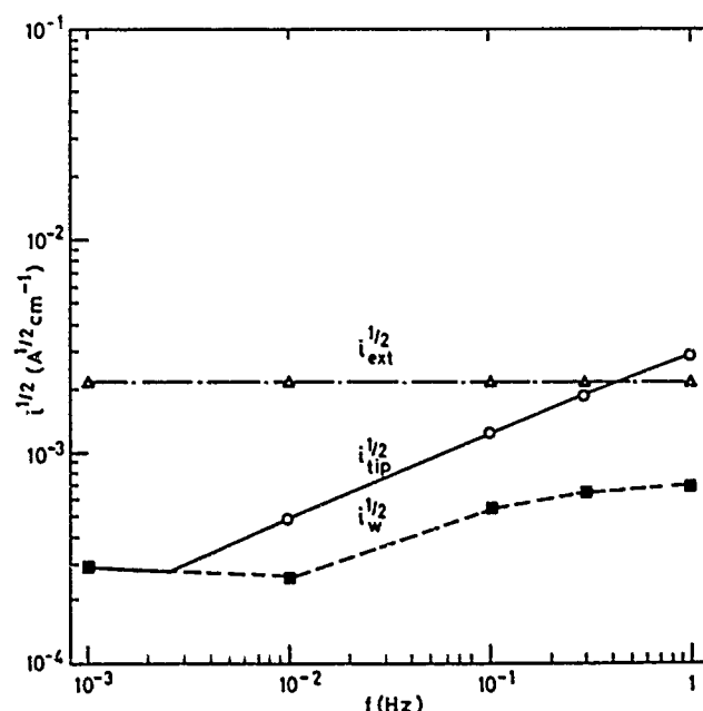
FIGURE 2—Effect of frequency on the square root of the CD for E^{ext} = -900 \text{ mV}_{SCE} , \Delta K = 20 \text{ MPa m}^{1/2} and R = 0.5 .
