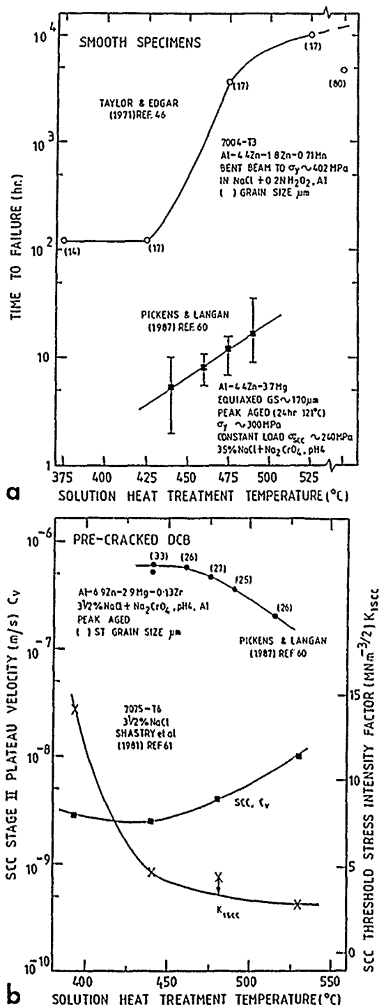
FIGURE 3—Influence of solution heat treatment upon the SCC performance of Al-Zn-Mg alloys in saline environments; (a) time-to-failure from smooth specimens and (b) Region 2 SCC plateau crack velocities from precracked specimens.
