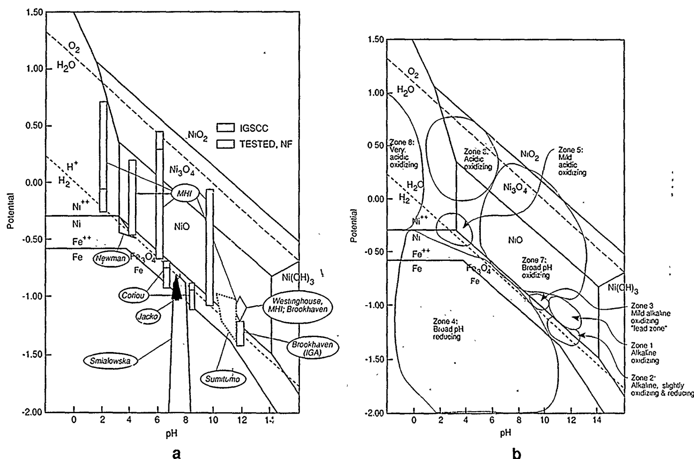
FIGURE 69—Results of plotting data from SCC investigations for Inconel 600 (UNS N06600) on Pourbaix diagram for nickel. (a) Schematic view showing location of data. (b) Suggested locations of zones for different modes of corrosion.
