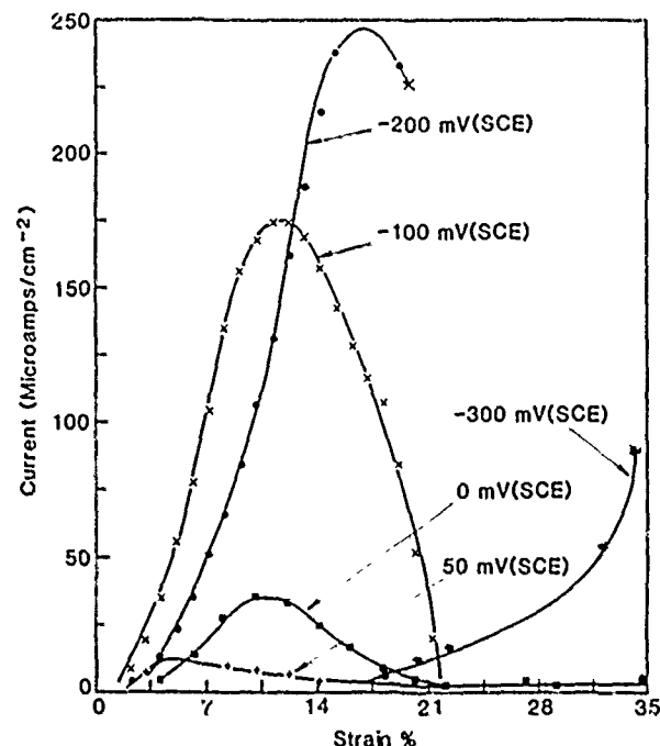
FIGURE 7—Corrosion current measured during slow-strain-rate tests at different electrode potentials.
