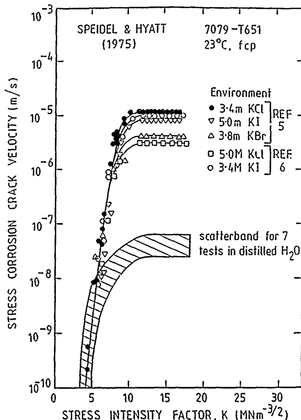
FIGURE 19—Stress corrosion crack velocities as a function of stress-intensity factor for 7079-T651 in distilled water and various aqueous halide ion solutions.
