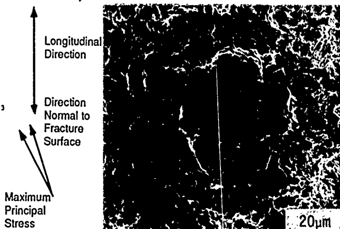
FIGURE 12—Crack Initiated at the bottom of a corrosion pit under multiaxial cyclic-static loads ( \tau_{\max}/\sigma_{\max} = 1/2 , \sigma_{\max} = 1100 MPa, R_{\sigma} = 0 , \tau = 550 MPa, R_{\tau} = 1 ).
