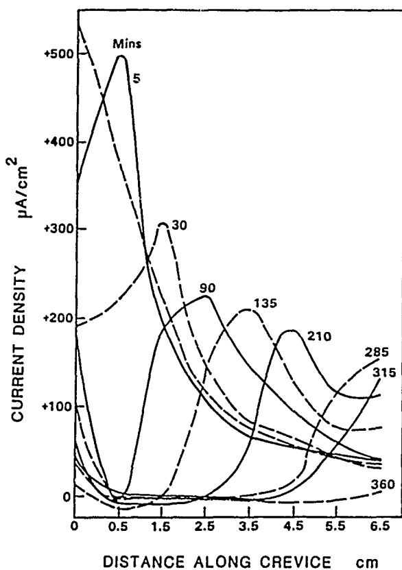
FIGURE 11—Current density-distance curves at various times for C-Mn steel surfaces exposed to \text{CO}_3/\text{HCO}_3 solution in segmented crevice at 75^\circ\text{C} . Well potential -0.65\text{ V} , crevice thickness 0.25\text{ mm} . 60
