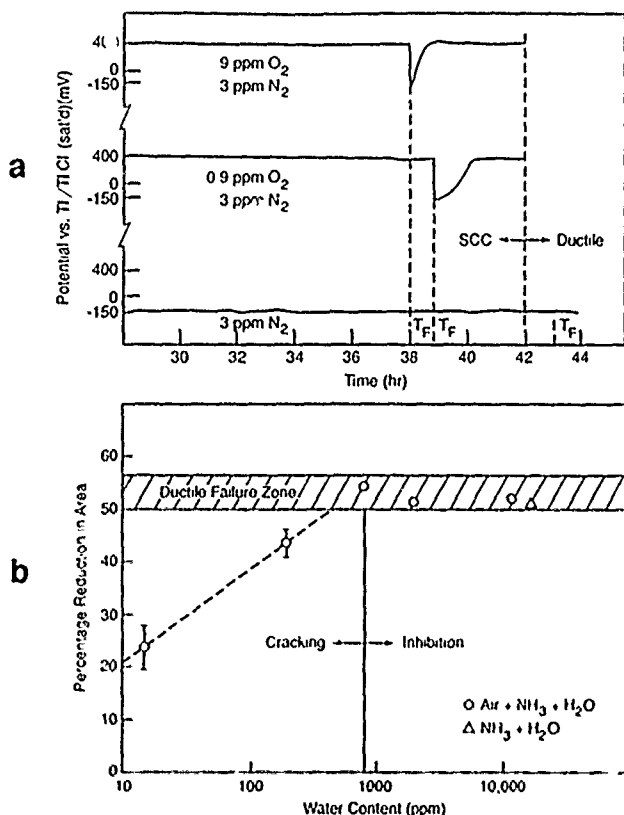
FIGURE 19—Effects of oxygen and water on the SCC of mild steel in anhydrous ammonia from work by Deegan, et al. (a) Effect of oxygen addition on the SCC as shown by potential transients occur corresponding to the occurrence of SCC, and (b) effect of water on SCC. From work of Deegan, et al. 51,52
