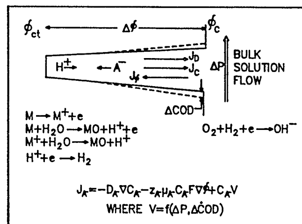
FIGURE 17—Schematic of a crack and the associated mass transport and thermodynamic criteria that govern the crack-tip environment.
