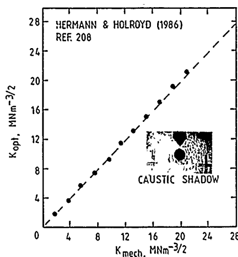
FIGURE 47—Stress-Intensity factor (K) obtained by the shadow method of caustic ( K_{opt} ) as a function of K via conventional linear elastic fracture mechanics ( K_{mech} ). 208 (Insert shows a typical caustic).
