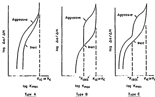
FIGURE 1—Schematic representations of corrosion fatigue crack propagation rate behavior; after McEvily and Wei. 25
