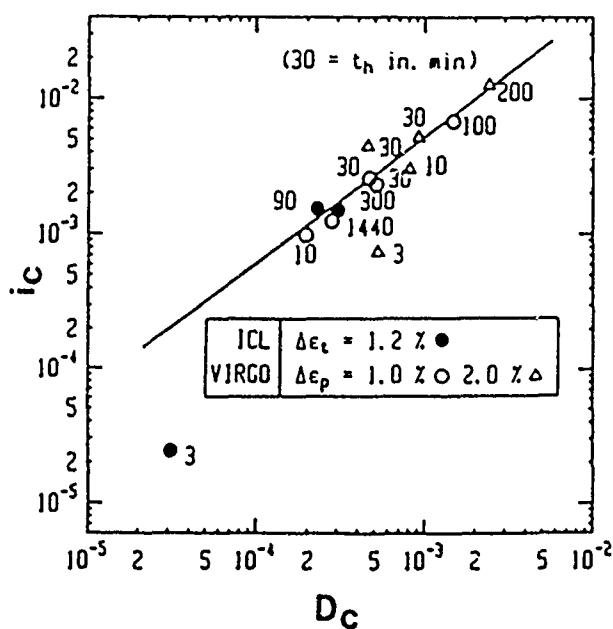
FIGURE 7—Correlation between the relative reduction in fatigue life, measured by i_c parameter and measured intergranular damage per cycle ( D_c ).
