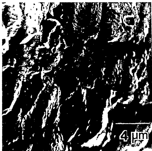
FIGURE 49—SEM fractograph of an IGSCC fracture face of an Al-Zn-Mg alloy, 7018-T76, stressed in an acidified inhibited saline environment (courtesy of G.M. Scamans).
