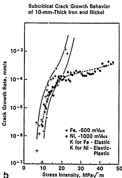
FIGURE 14—Subcritical crack growth (a) for 2-mm-thick Fe and Ni tested in 1 N H 2 SO 4 at 25°C, and (b) for 10-mm-thick Fe and Ni tested in 1 N H 2 SO 4 at 25°C.
