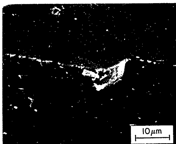
FIGURE 8—Fracture along shear bands in amorphous \text{Fe}_{40}\text{Ni}_{38}\text{B}_{18}\text{Mo}_4 tested in bending in lithium at 200°C. 12
