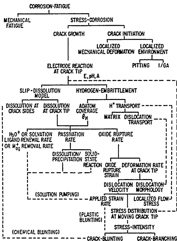
FIGURE 16—Suggested interaction paths between the modes and mechanisms of environmentally controlled fracture in ductile alloy/aqueous environment systems and the various rate-determining steps in crack propagation. Solid lines denote primary interactions, dashed lines denote secondary interactions. 4,7
