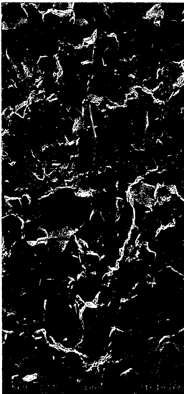
FIGURE 12—Transitions in fracture mode in response to environmental changes. Tests conducted at a \Delta K of 25 \text{ MPa}\sqrt{\text{m}} , a frequency of 1 Hz, and an R ratio of 0.1 (crack proceeded from top to bottom).
