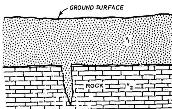
Figure B-22. Offset in time-distance plot due to discontinuity in rock surface (prepared by WES)
