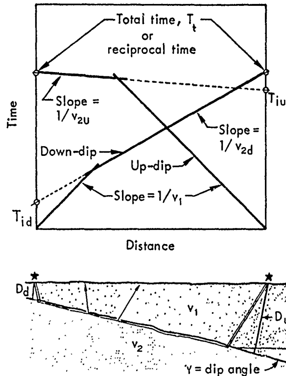
Figure B-8. Example of dipping interface and concepts of "reverse shooting" and "apparent velocity" (after Redpath 20 )
