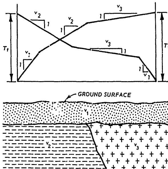
Figure B-23. Subsurface fault (prepared by WES)
