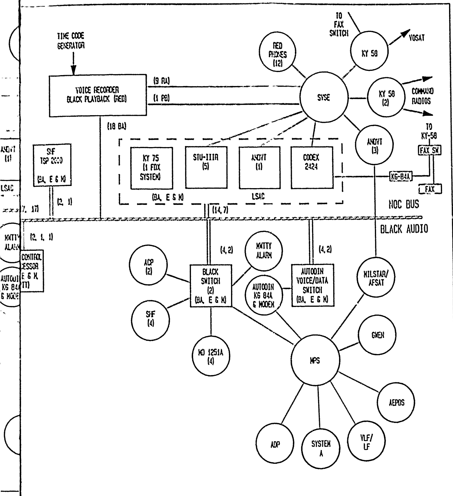
Figure 4-1. ATSS Functions on Bus
