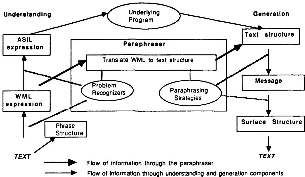
Figure 15: Architecutre of the Paraphraser
