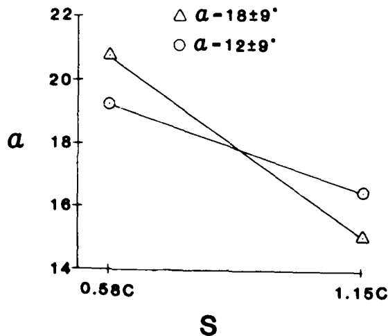
Fig. 10 Leading edge vortex initiation point, Re = 40,000 , K = 1.0 , \alpha_m = 12^\circ and 18^\circ , \alpha_i = 9^\circ .
