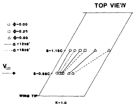
Fig. 12 Planform leading edge vortex position, Re = 40,000 , K = 1.0 , \alpha_m = 12^\circ and 18^\circ , \alpha_i = 9^\circ .
