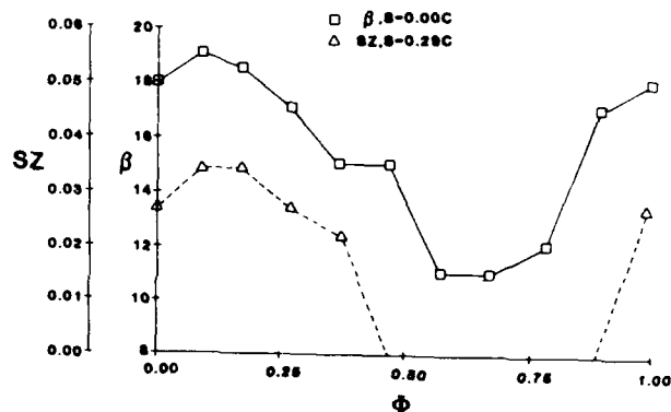
Fig. 13 Wing tip deflection angle and leading edge vortex size comparison, \beta at S=0.0 , SZ at S=0.29c , Re = 40,000 , K = 1.0 , \alpha_m = 15^\circ , \alpha_i = 10^\circ .
