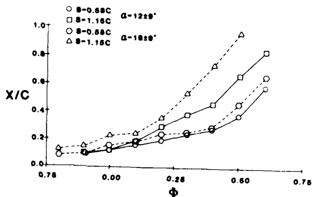
Fig. 11 Leading edge vortex position, Re = 40,000 , K = 1.0 , \alpha_m = 12^\circ and 18^\circ , \alpha_i = 9^\circ .
