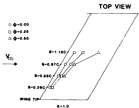
Fig. 9 Planform leading edge vortex position, Re = 40,000 , K = 1.0 , \alpha_m = 15^\circ , \alpha_w = 10^\circ , \phi = 0^\circ \alpha = 25^\circ , \phi = .5 \alpha = 5^\circ .
