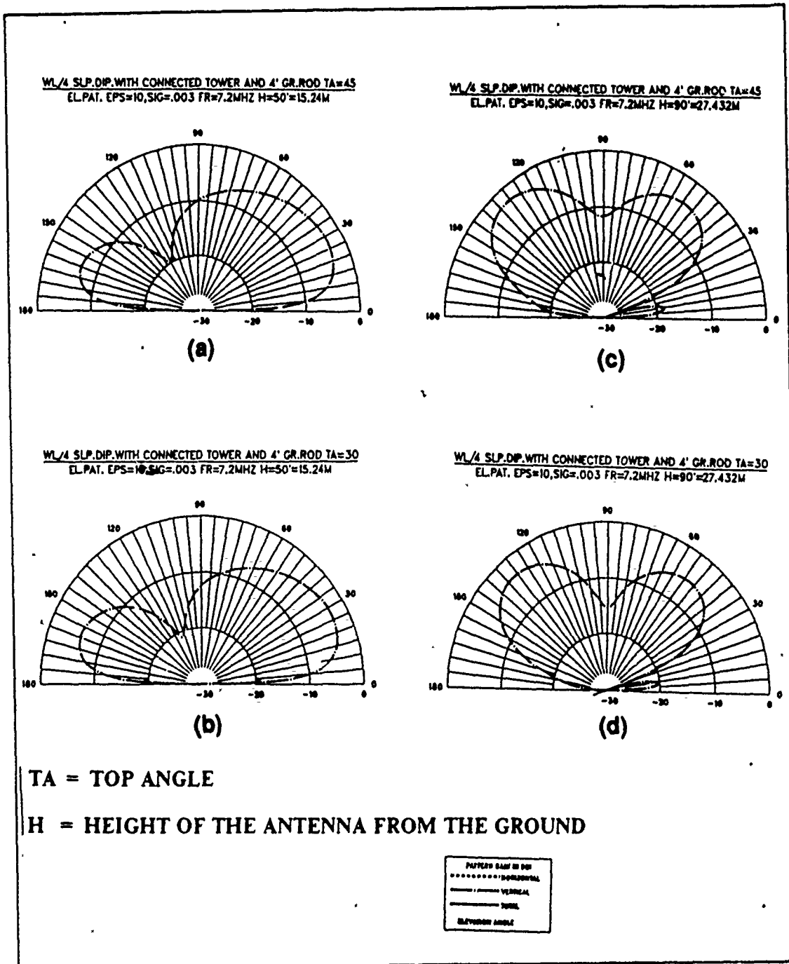
Figure 13. The elevation patterns of the sloping wire for 7.2 MHz: (a) TA = 45 degrees, H = 50-ft. (b) TA = 30 degrees, H = 50 ft. (c) TA = 45 degrees, H = 90ft. (d) TA = 30 degrees, H = 90 ft.
