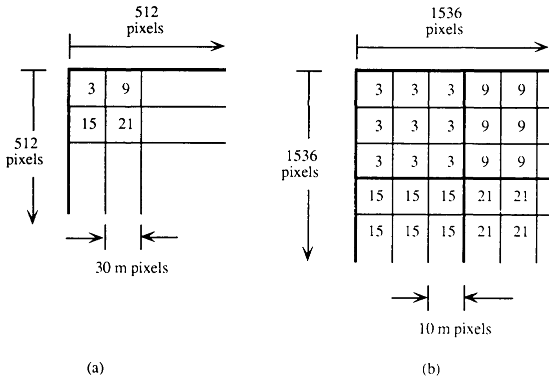
Figure 2-7 Pixel Replication
